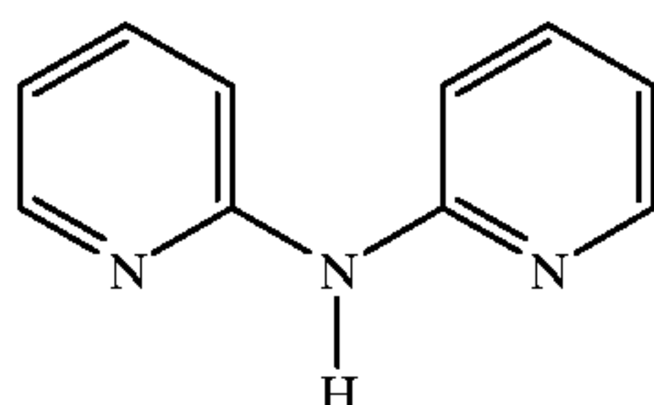
di-2-pyridyl amine
