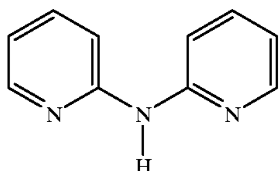
di-2-pyridyl amine
