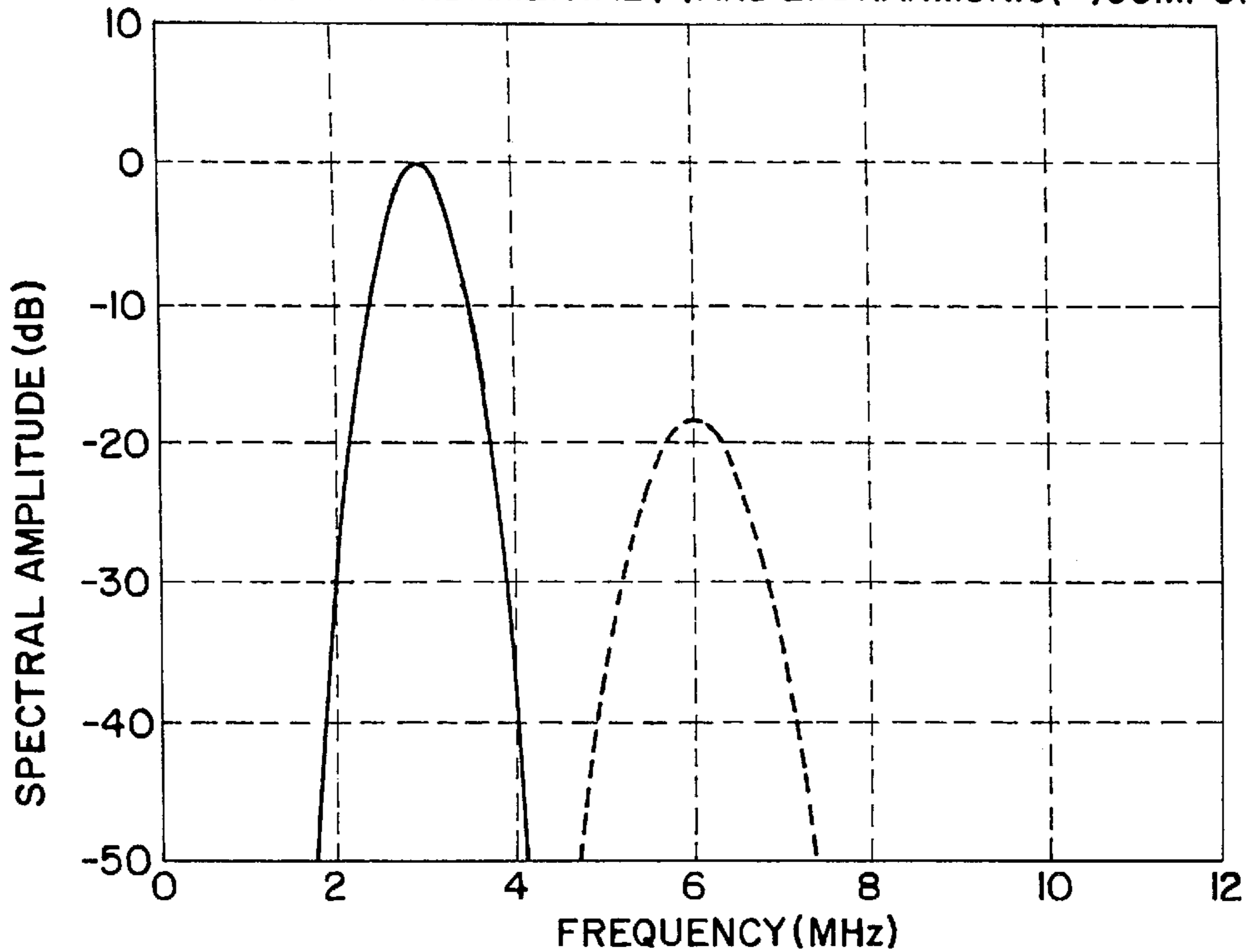
SOURCE SPECTRUM: FUNDAMENTAL (—) AND 2nd HARMONIC (---) COMPONENTS
