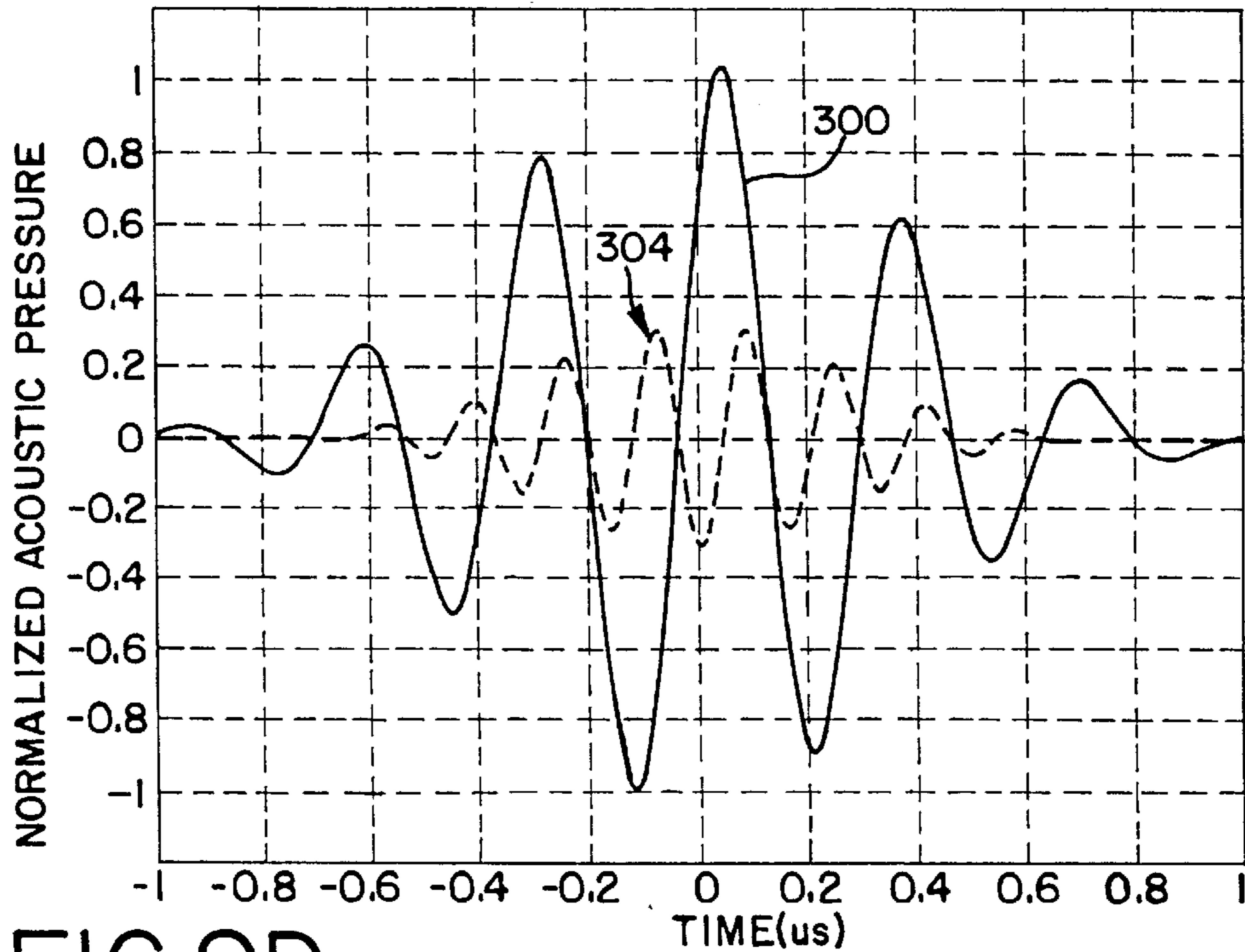
SOURCE WAVEFORM: FUNDAMENTAL (—) AND 2nd HARMONIC (---) COMPONENTS
