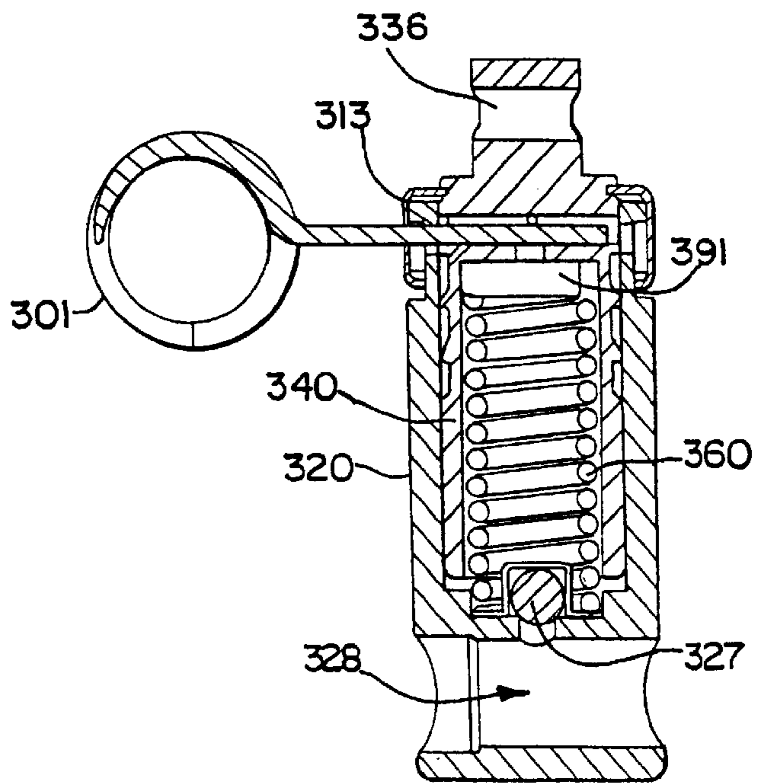
SECTION B-B
