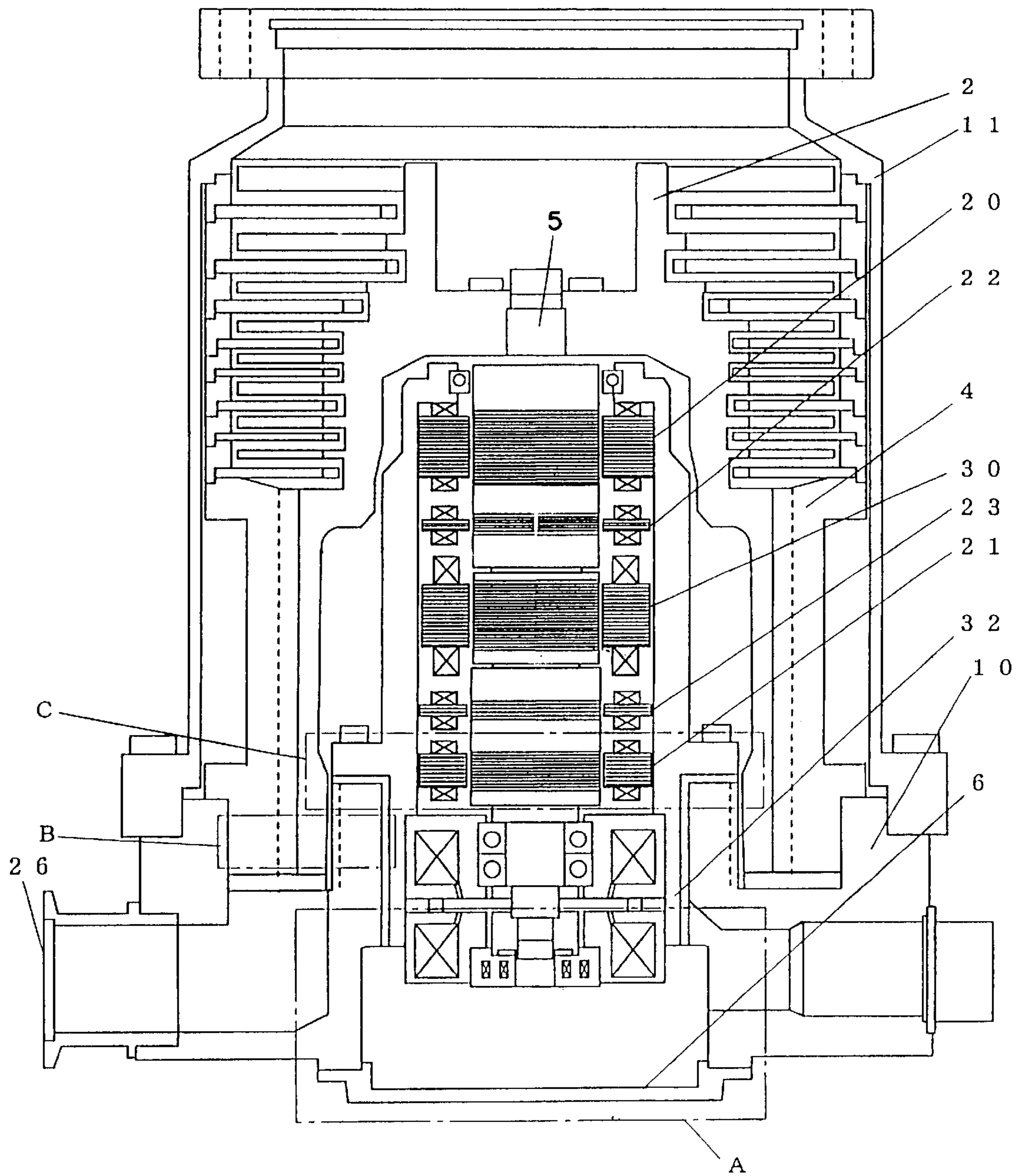
Fig. 6 PRIOR ART
