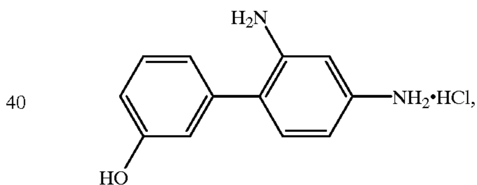
and the like; Diphenal, of the formula
