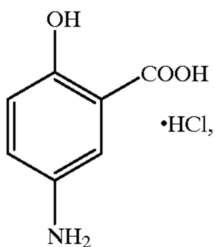
p-aminosalicylic acid (Neol), of the formula
