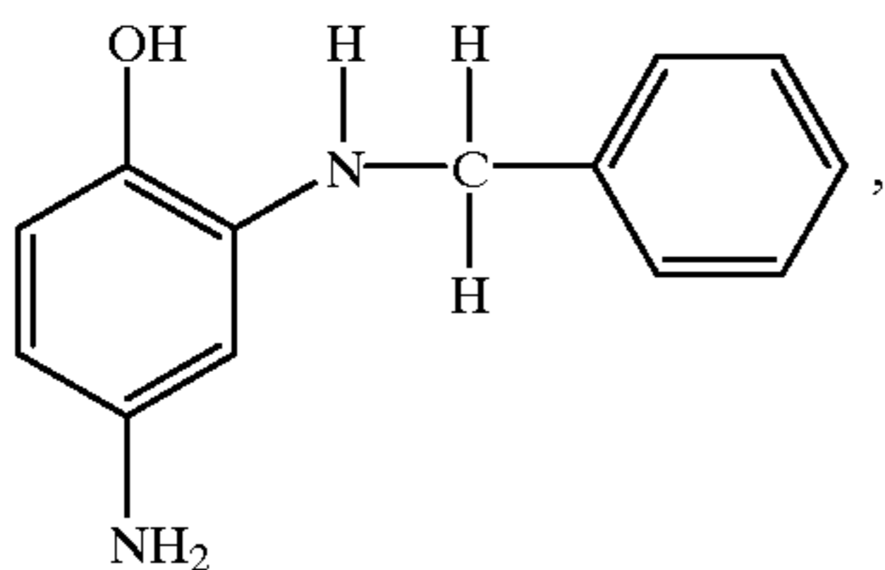
2-amino-4-(p-hydroxybenzylamino)phenol, of the formula
