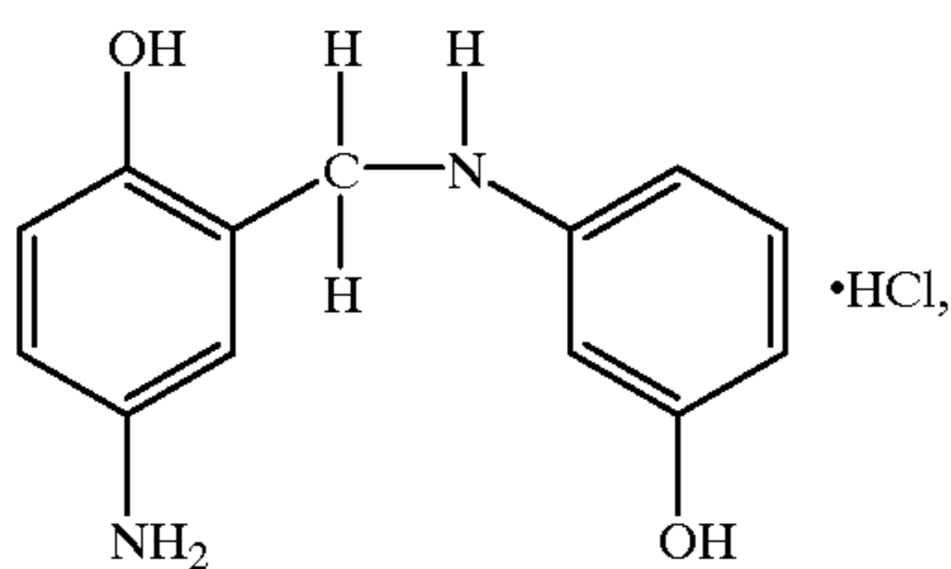
4-amino-2-benzylaminophenol, of the formula
