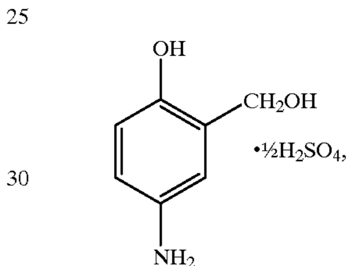
3-(hydroxymethyl)-4-hydroxyaniline hemisulfate (Edinol), of the formula
