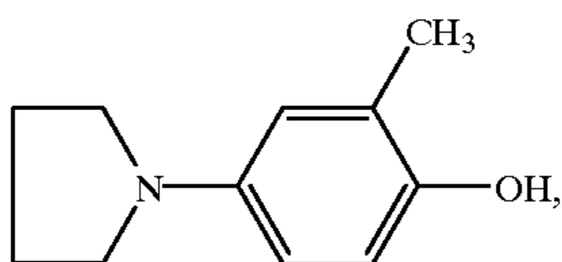
1-(4-hydroxyphenyl)pyrrolidine, of the formula
