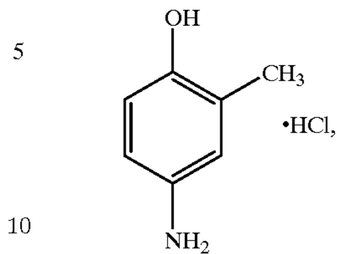
N-(hydroxyethyl)-o-aminophenol (Atomal), of the formula
