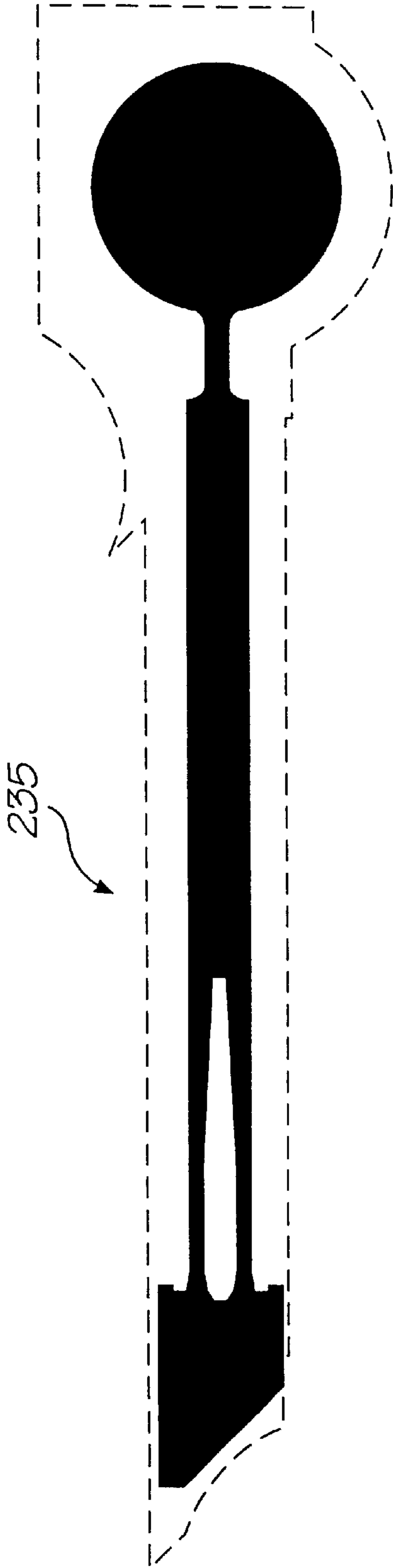
Actuator / bend compensator mask
