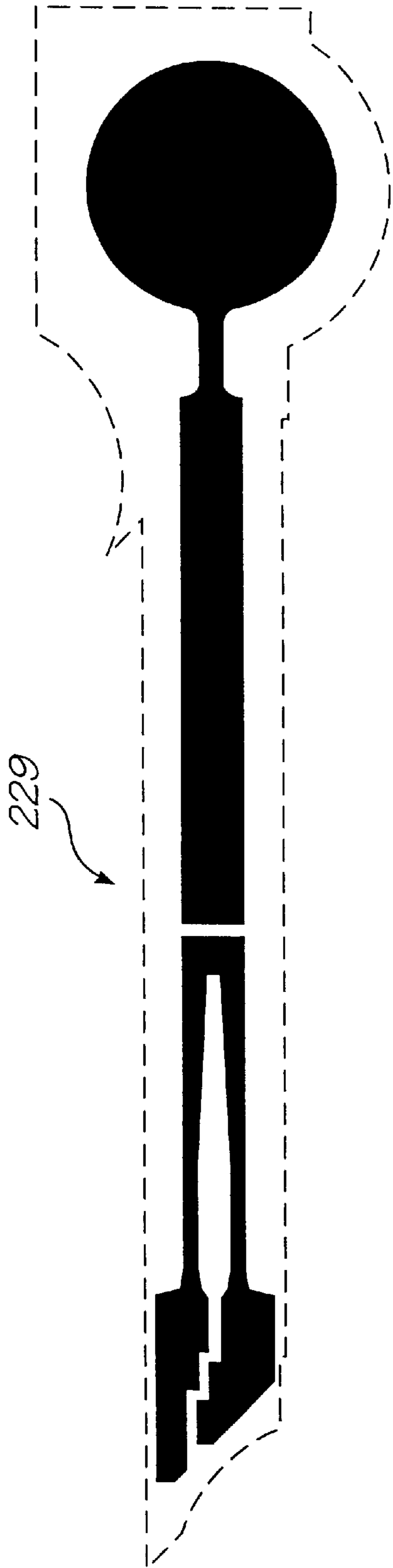
Heater mask
