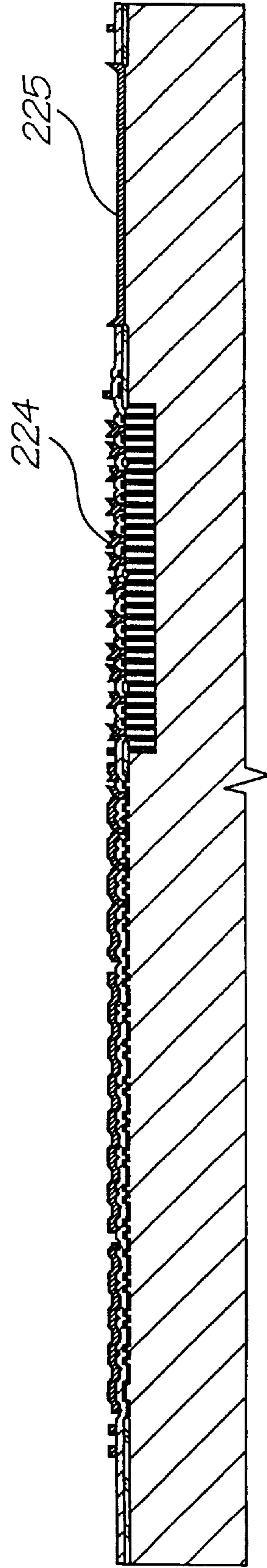
Deposit Metal 1
