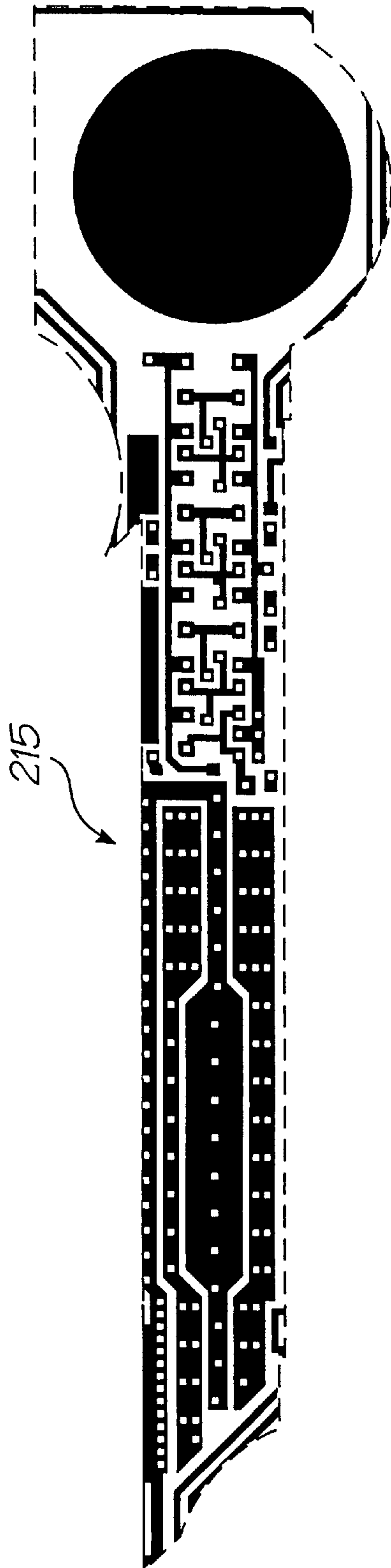
Metal 1 mask
