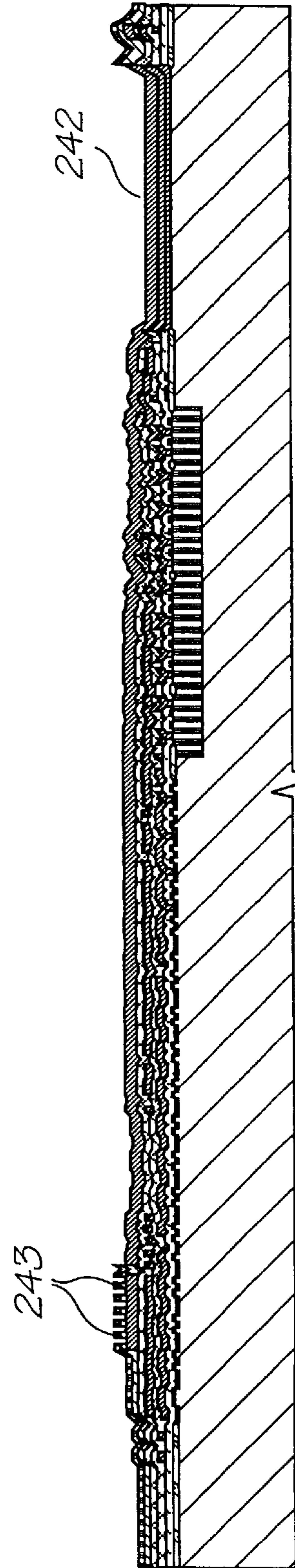
Deposit passivation oxide & nitride, etch vias
