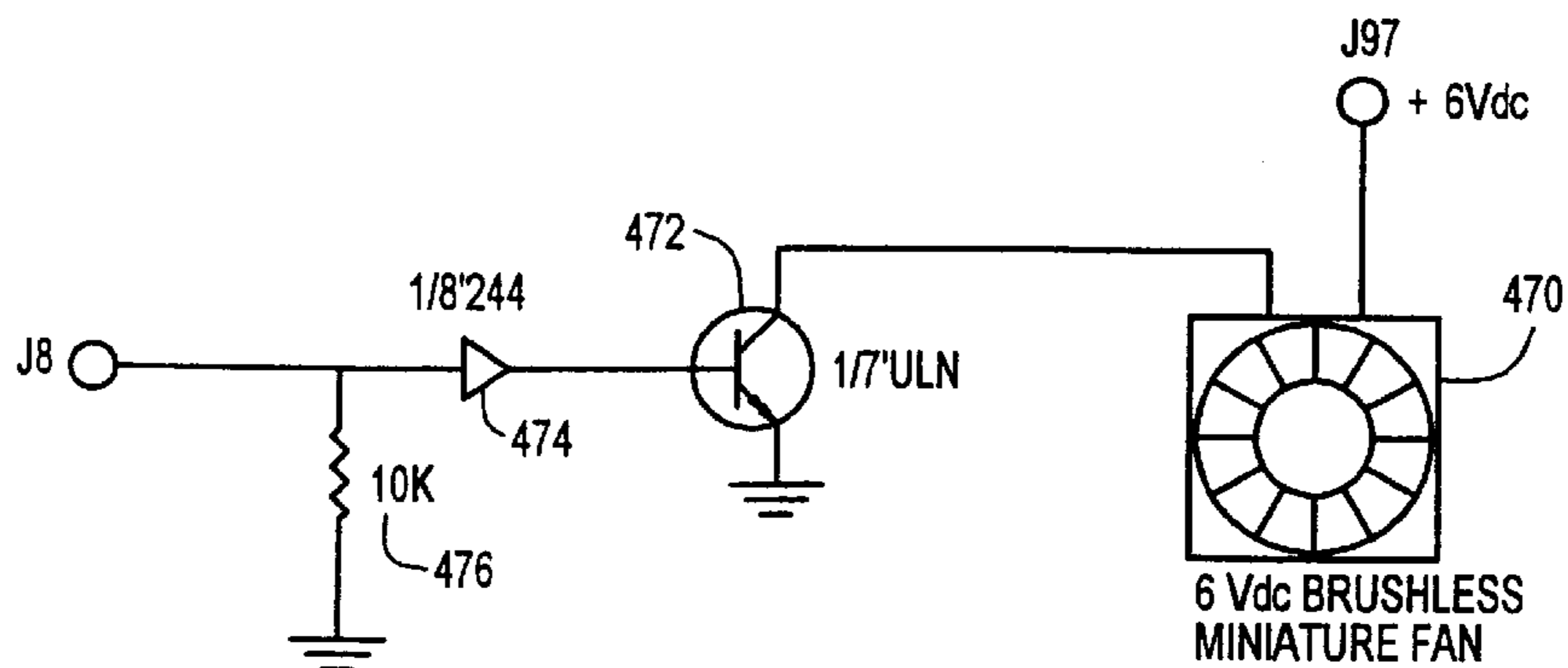
FIG. 36 SCAVENGING SYSTEM 468
