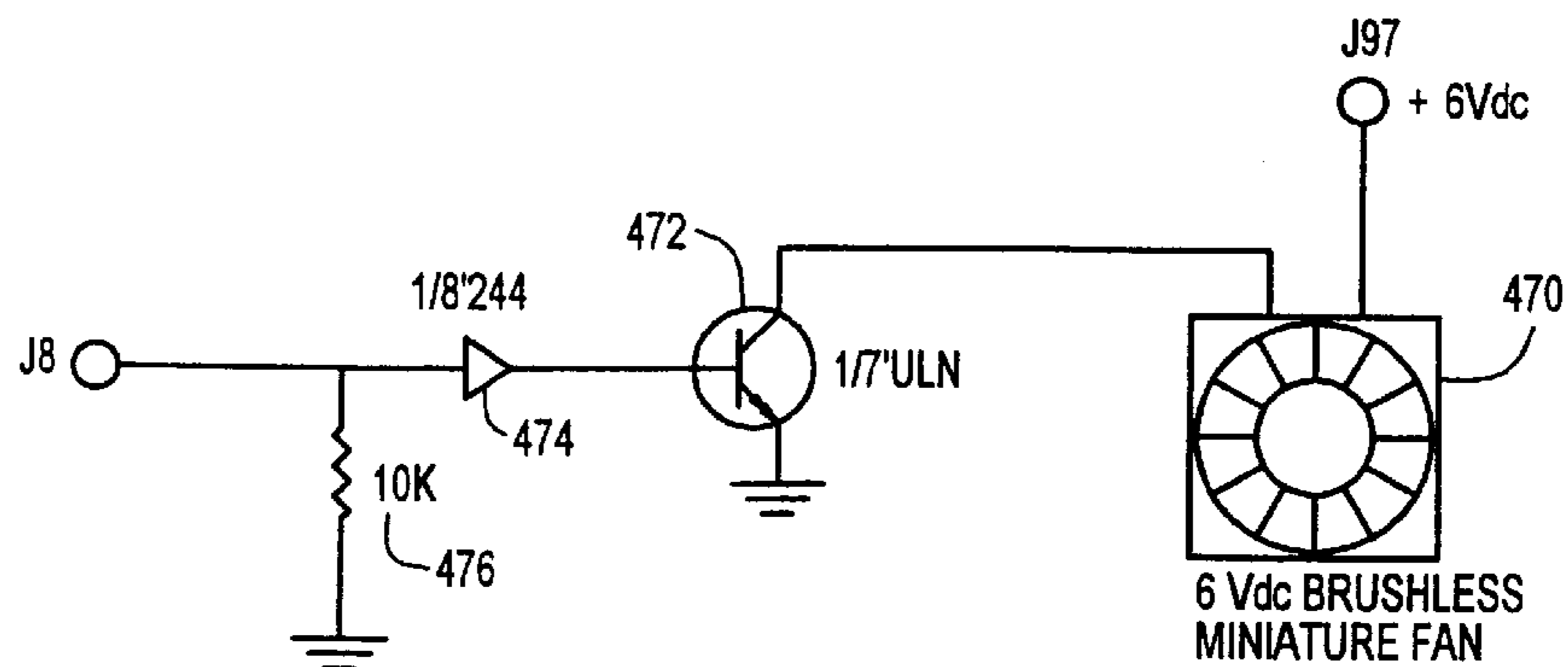
FIG. 36 SCAVENGING SYSTEM 468
