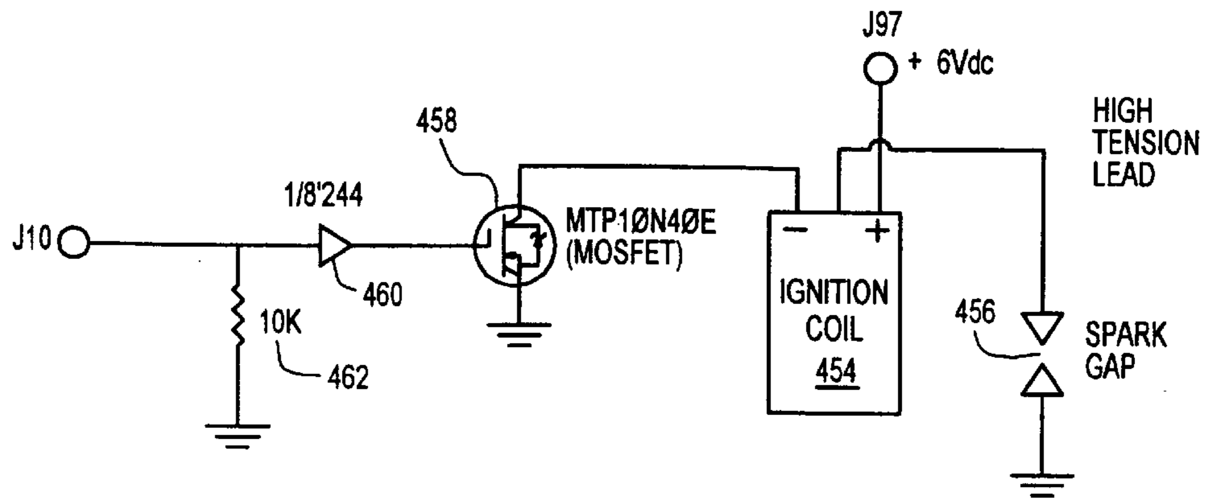
FIG. 35 IGNITION SYSTEM 452
