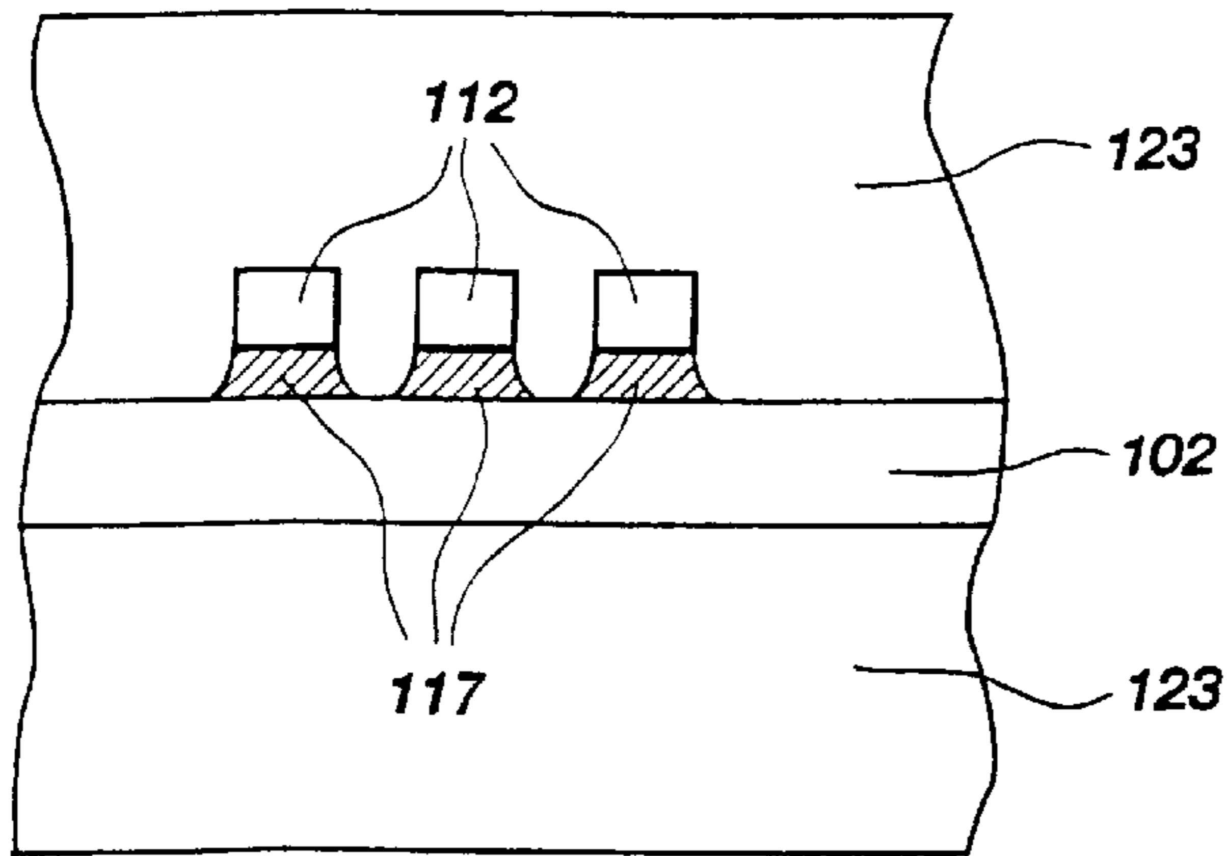
SECTION 10-10
