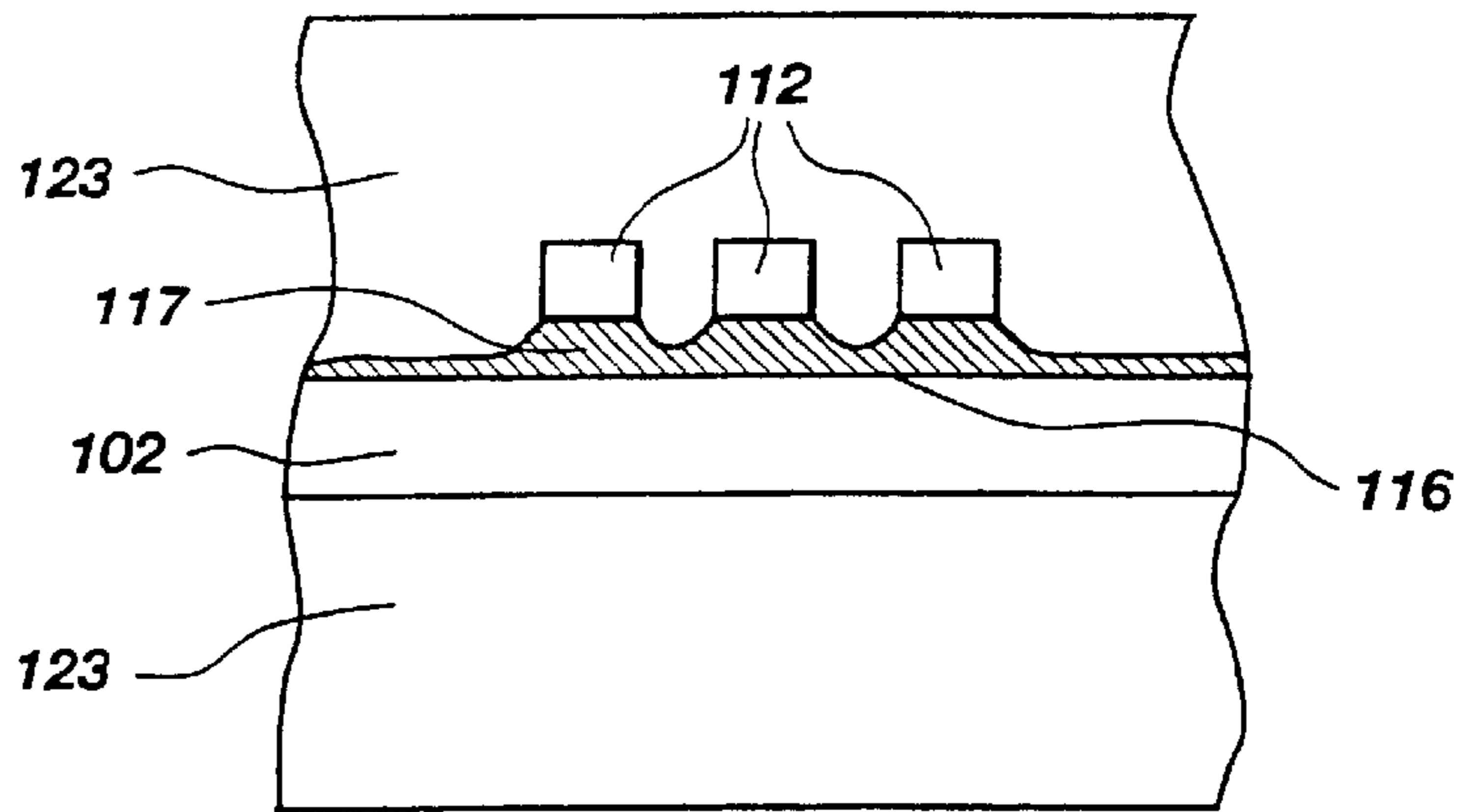
SECTION 10-10
