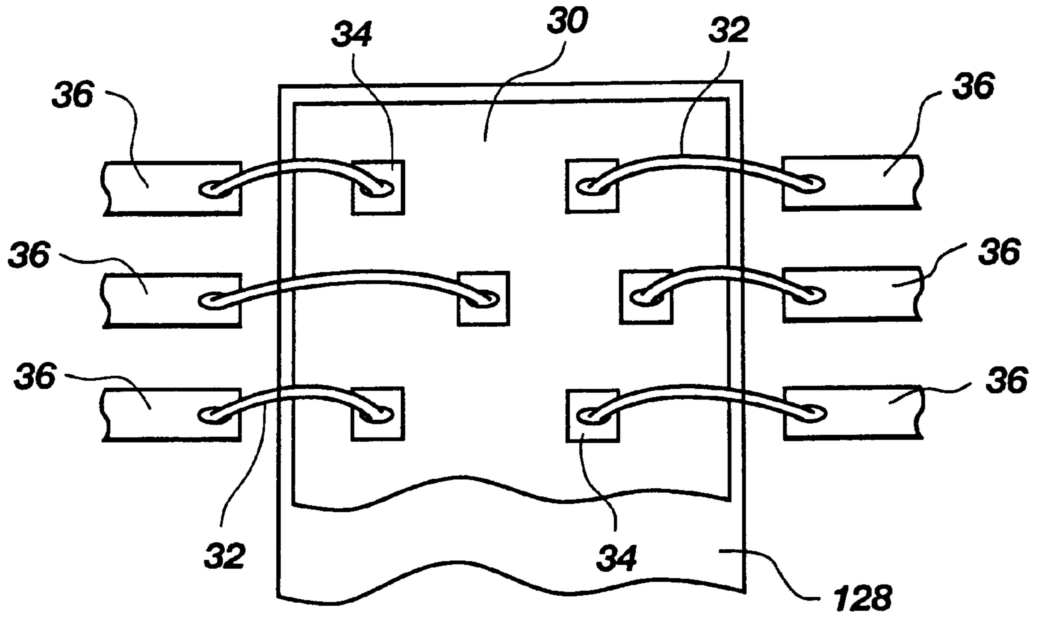
Fig. 6 (PRIOR ART)
