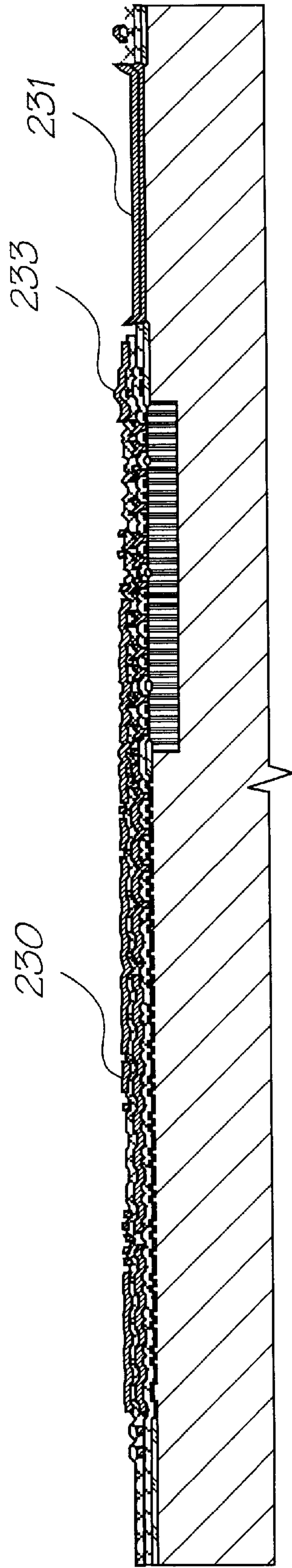
Deposit metal 2
