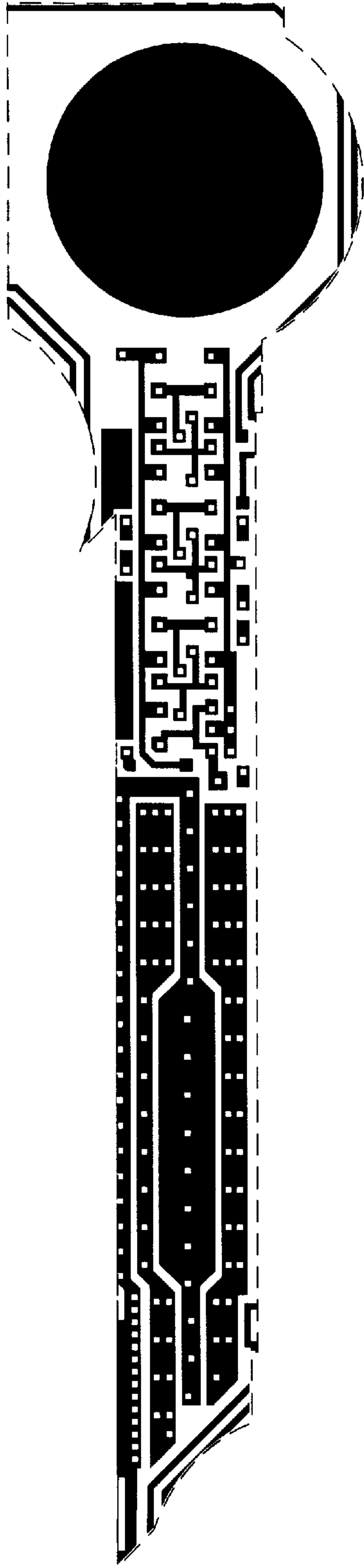
Metal 1 mask
