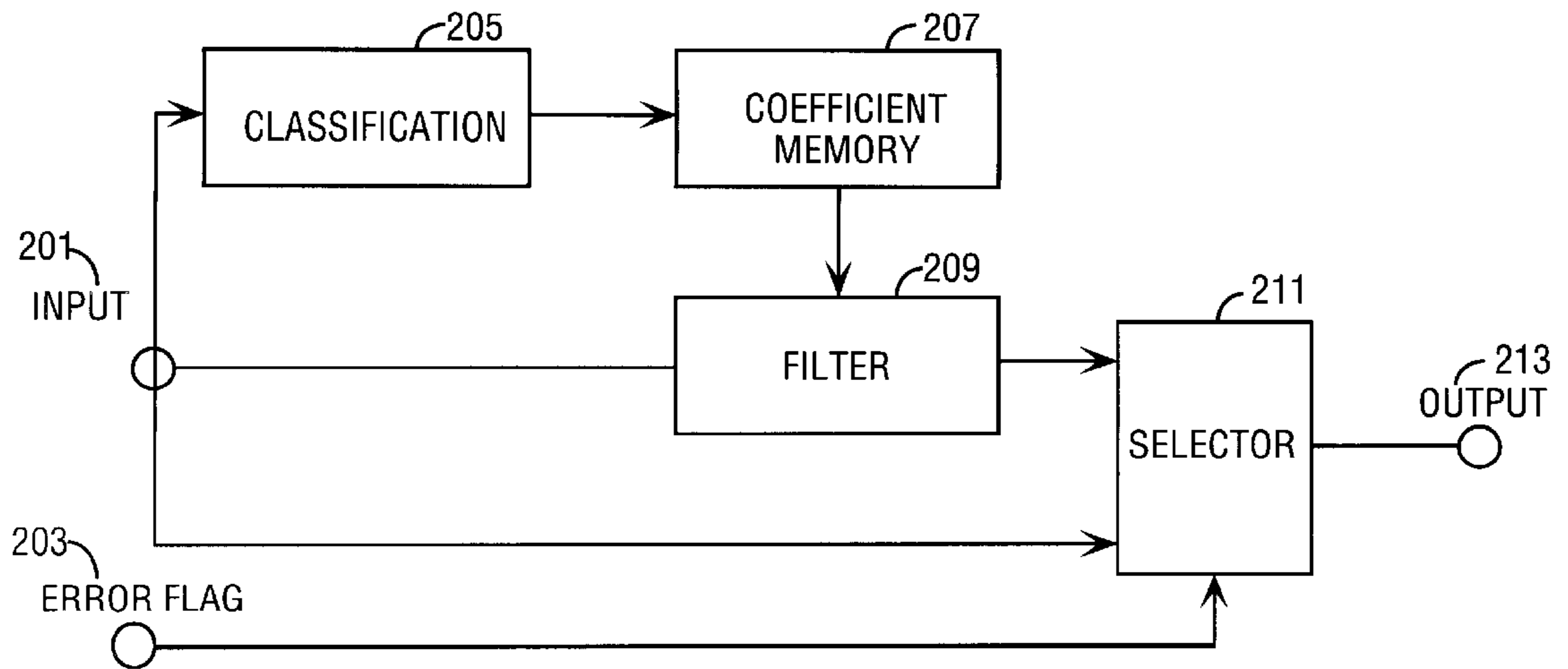
FIG. 2 (A) CLASSIFIED ADAPTIVE ERROR RECOVERY BLOCK DIAGRAM
