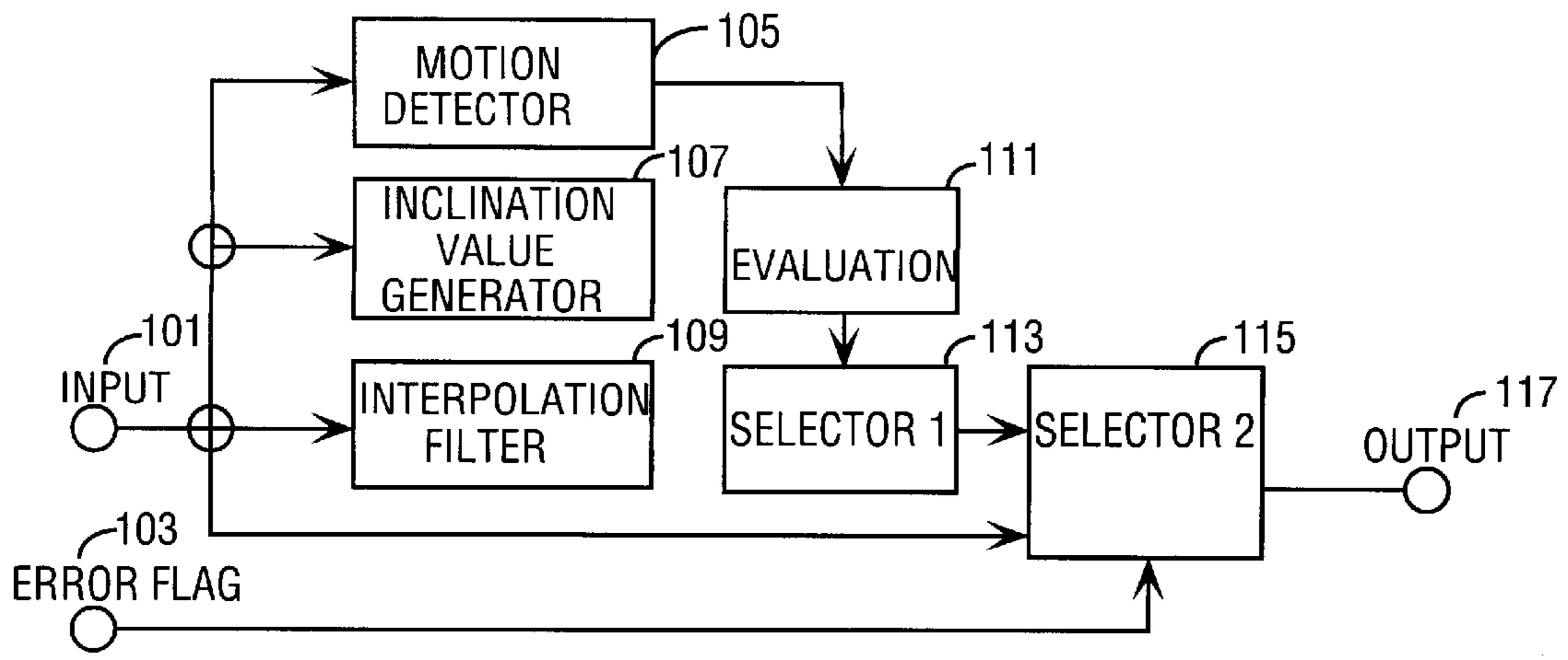
(A) CONVENTIONAL ERROR RECOVERY METHOD
