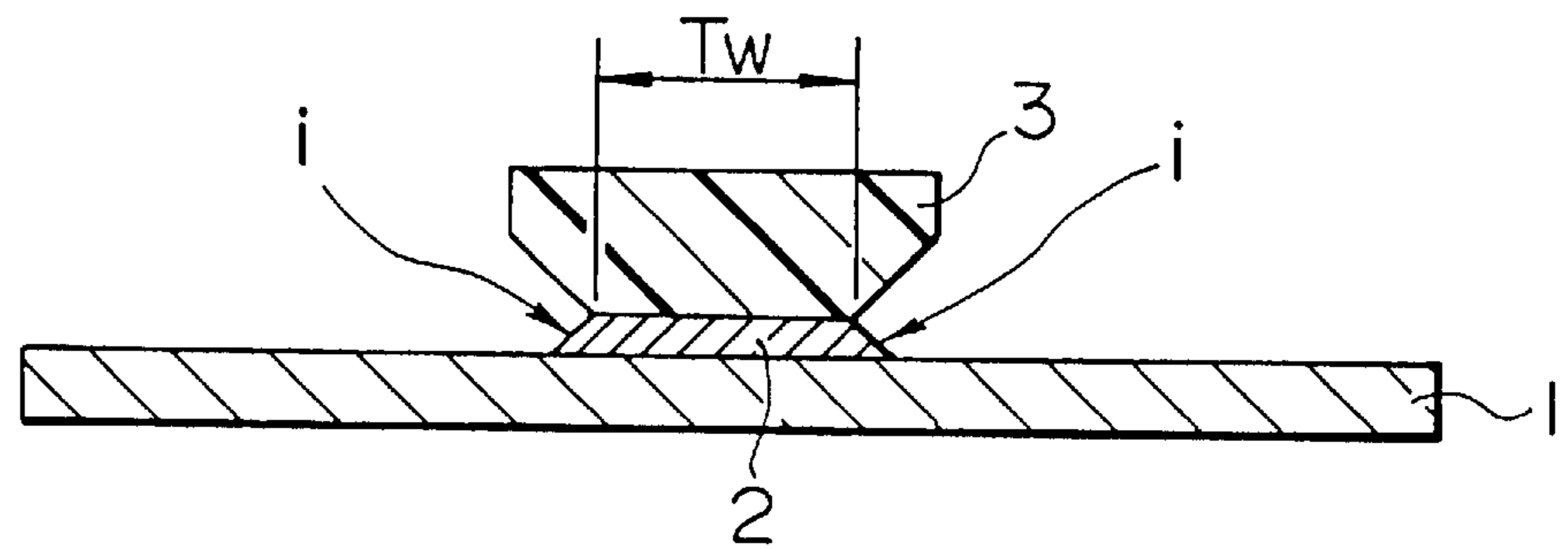
FIG. 12C (PRIOR ART)
