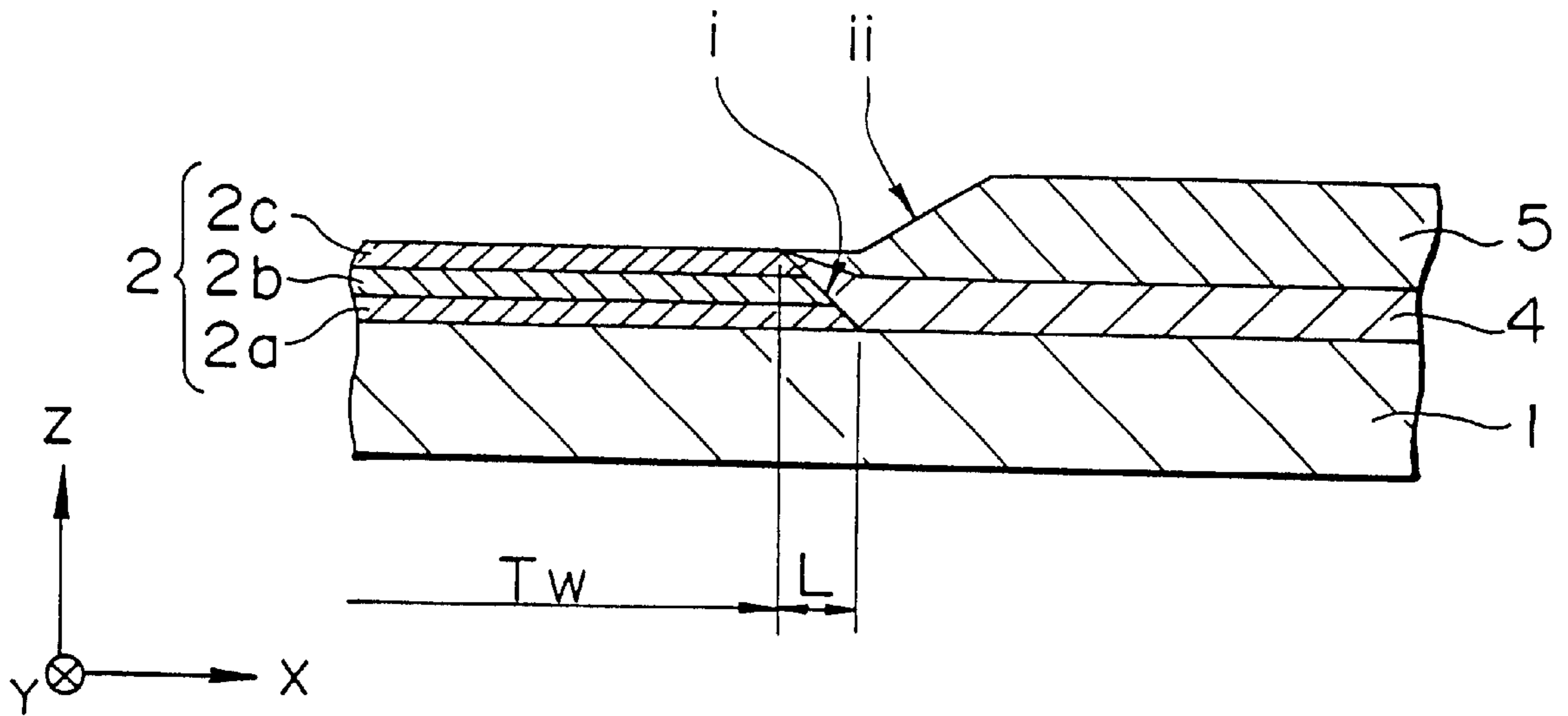
FIG. 13 (PRIOR ART)
