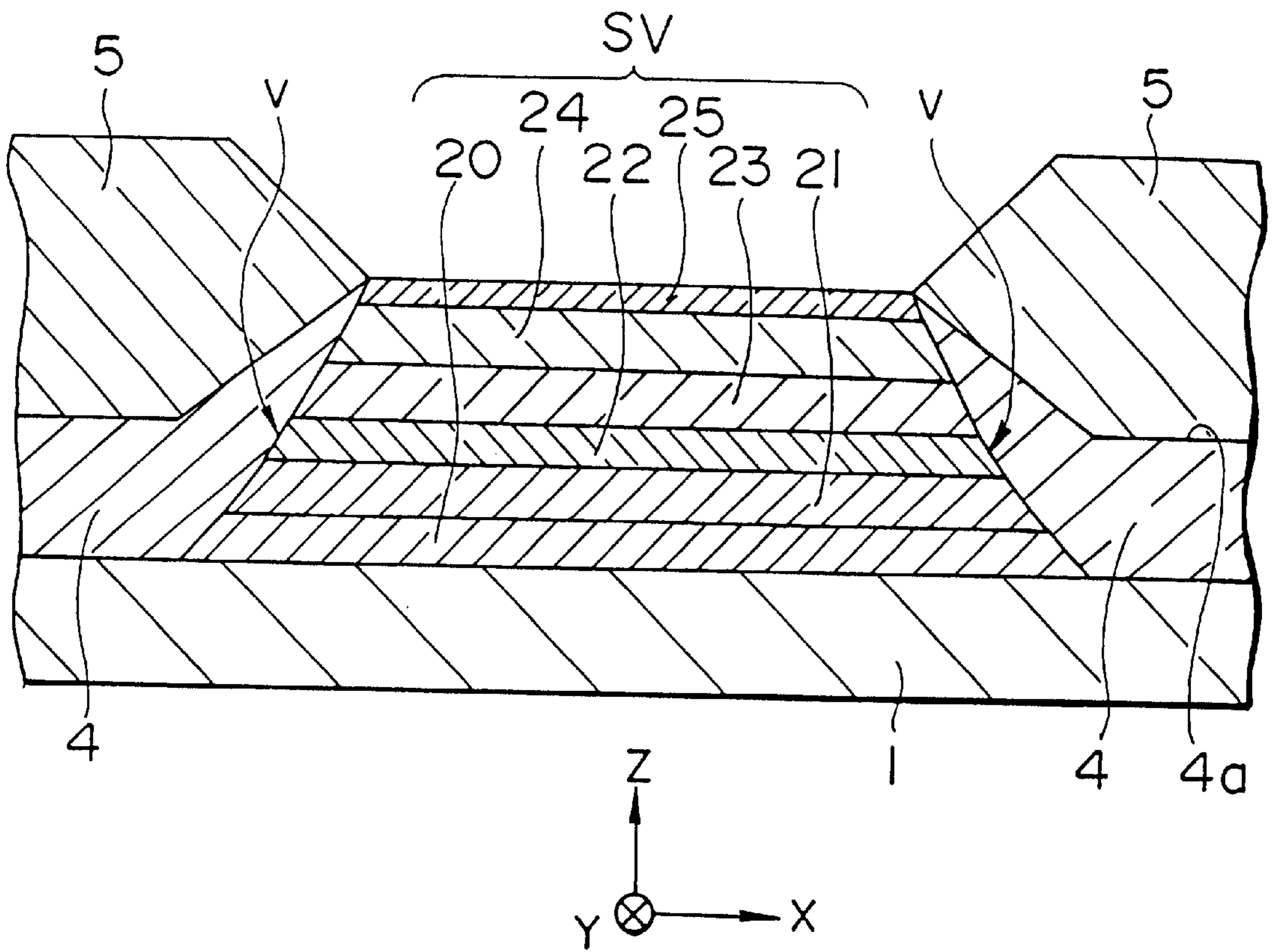
FIG. 14 (PRIOR ART)
