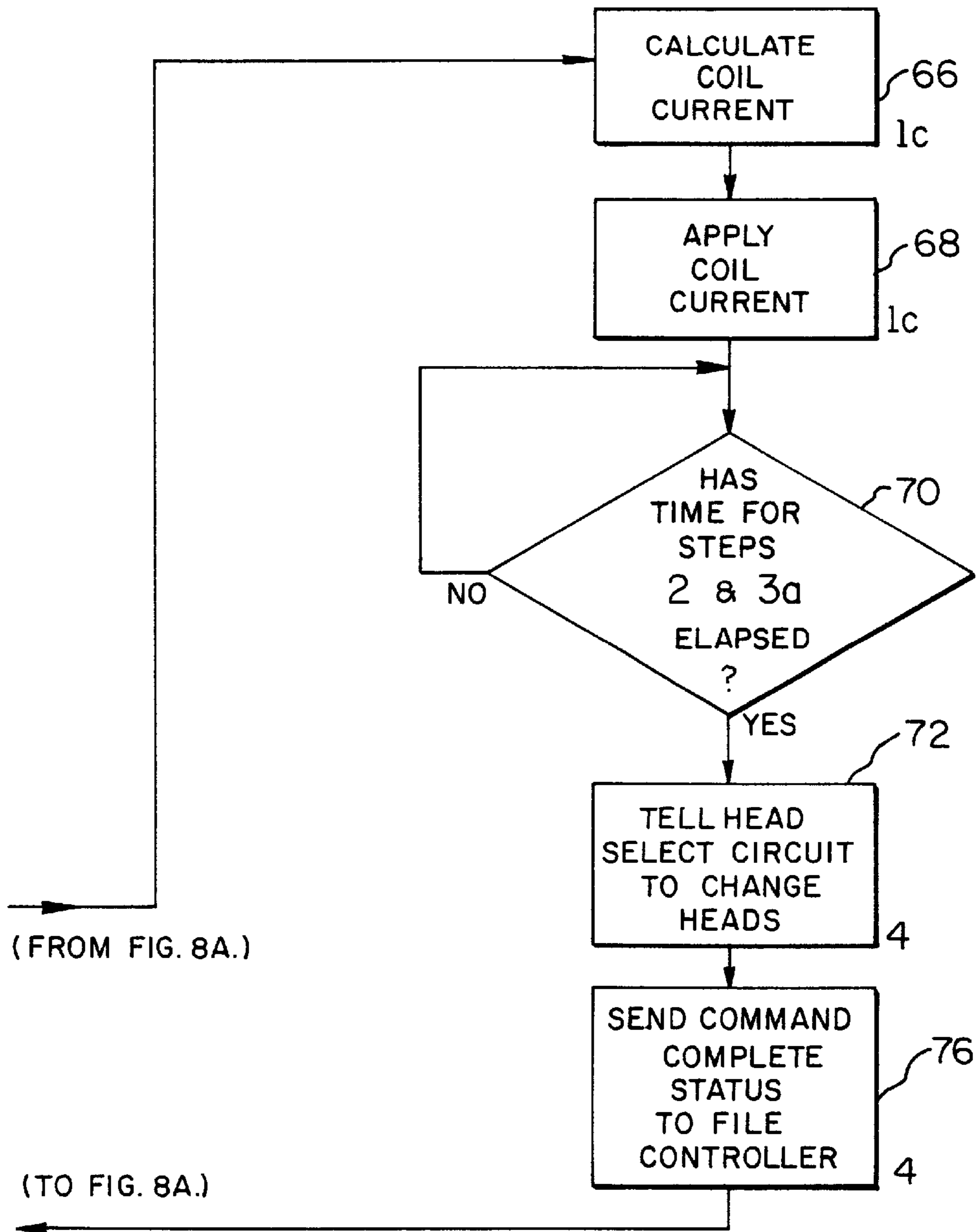
FIG. 8B. SERVO CONTROLLER PROCESS
