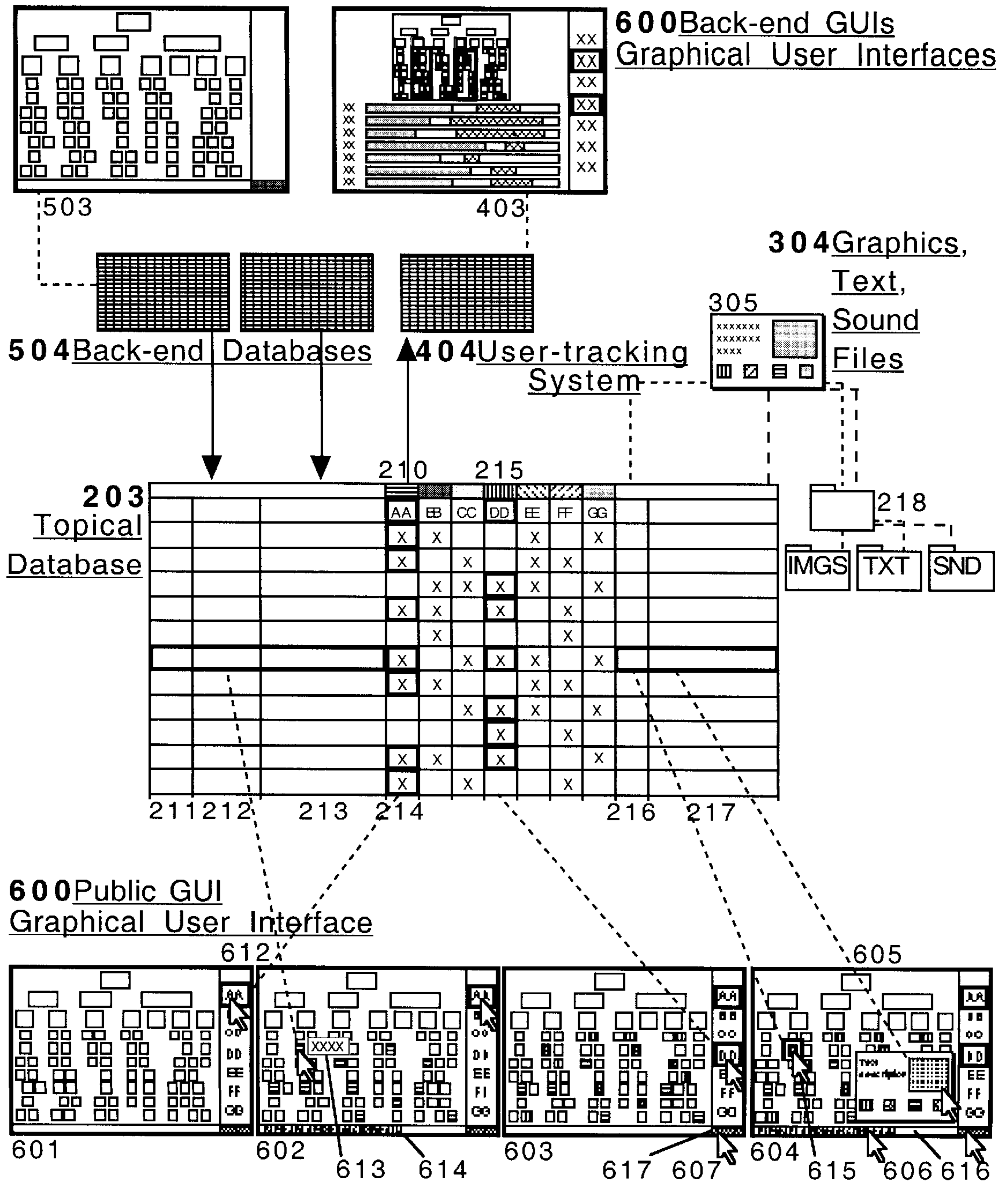
FIG. 4 GUI/Database Operations
