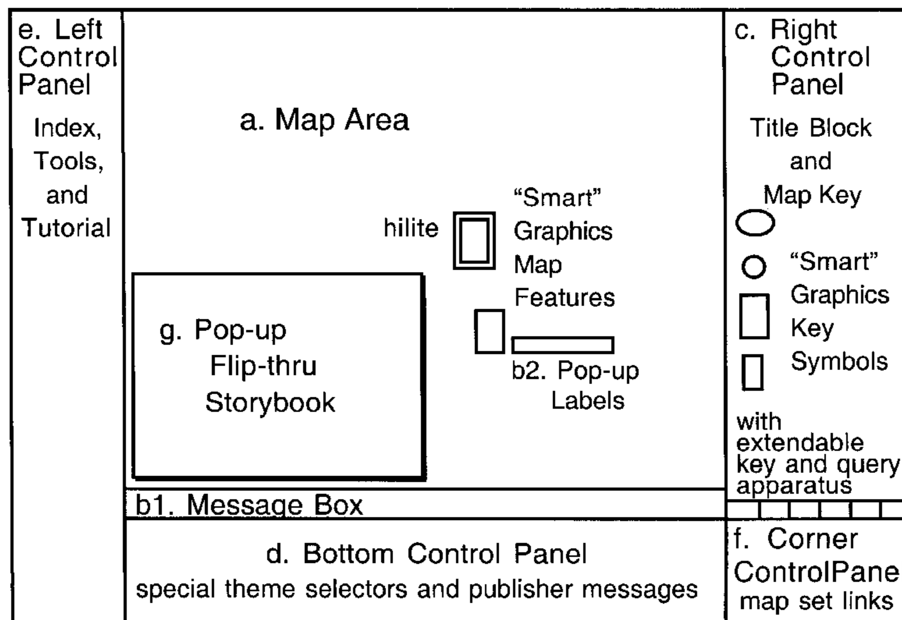
2 GUI Framework Components
