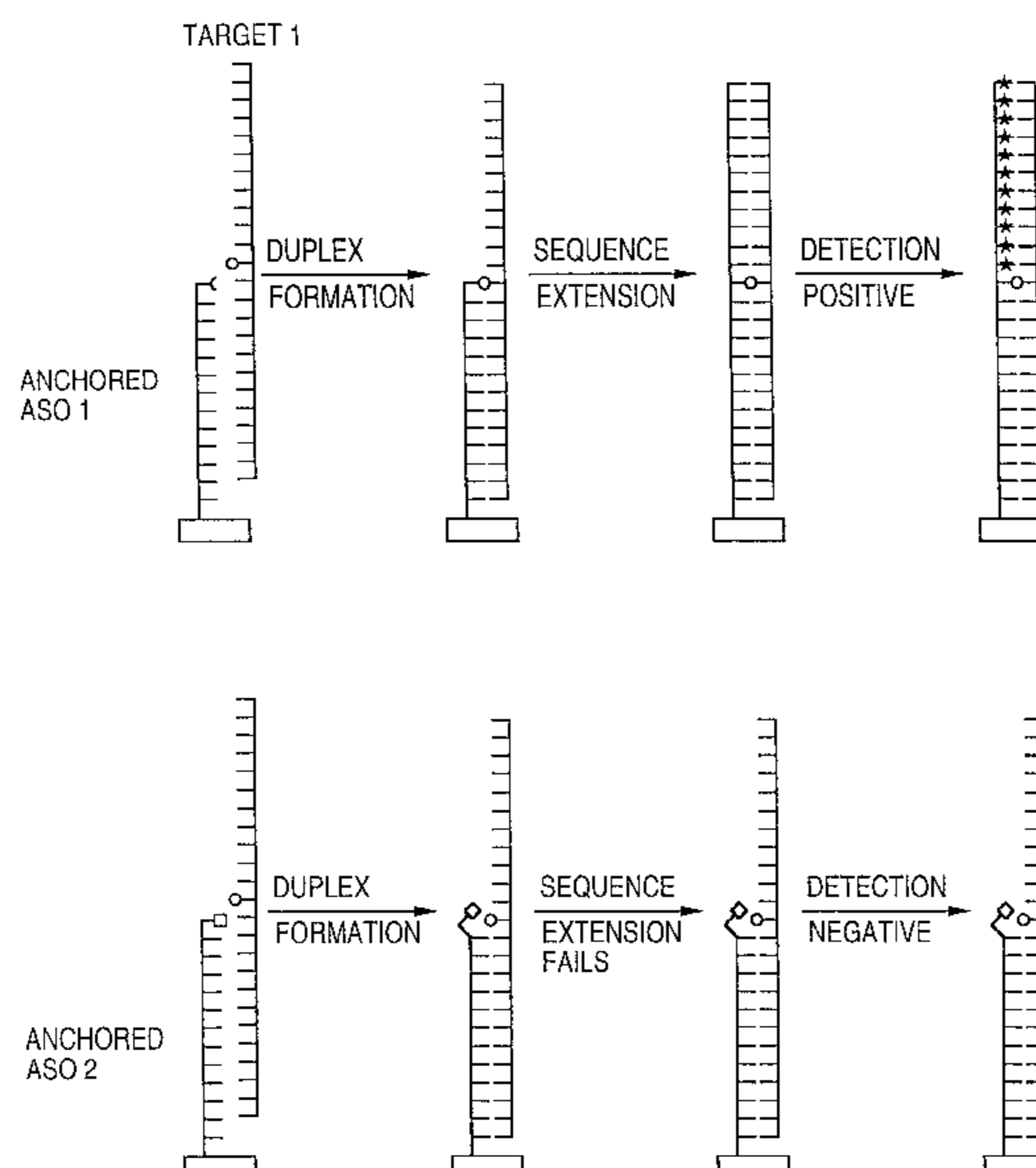
DETECTION OF POINT MUTATION BY HYBRIDISATION TO ASOs AND CHAIN EXTENSION
