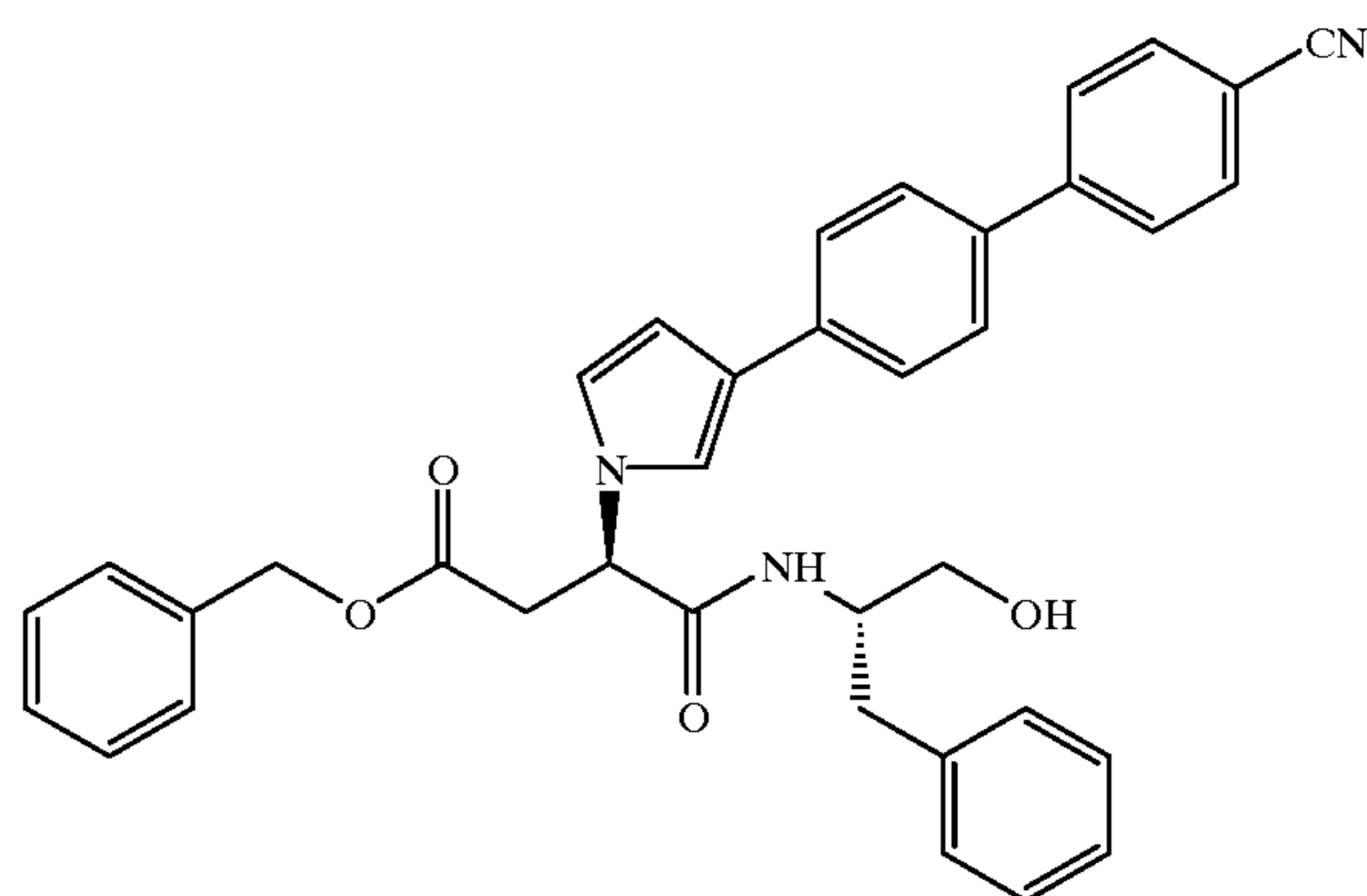
N-(1(S)-Benzyl-2-hydroxyethyl)-3(R)-[3-(4'-cyanobiphenyl-4-yl)1H-pyrrol-1-yl]succinamic Acid Benzyl Ester
