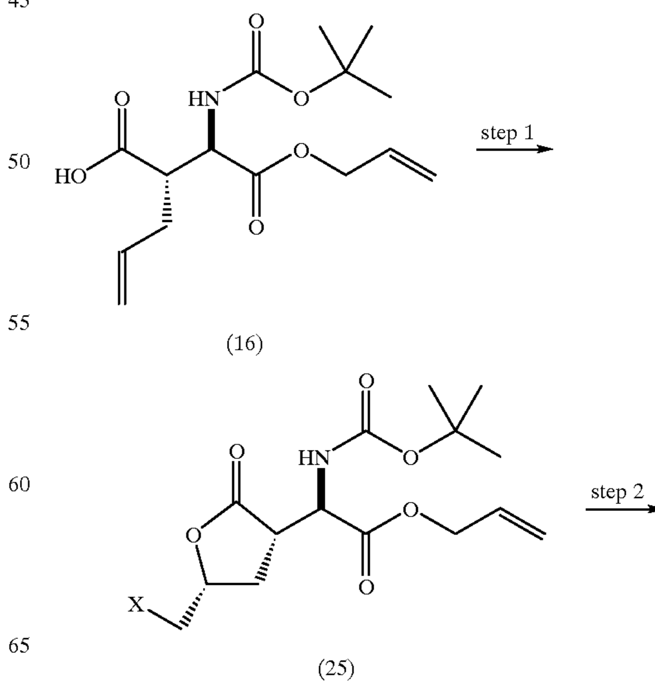
REACTION SCHEME X
