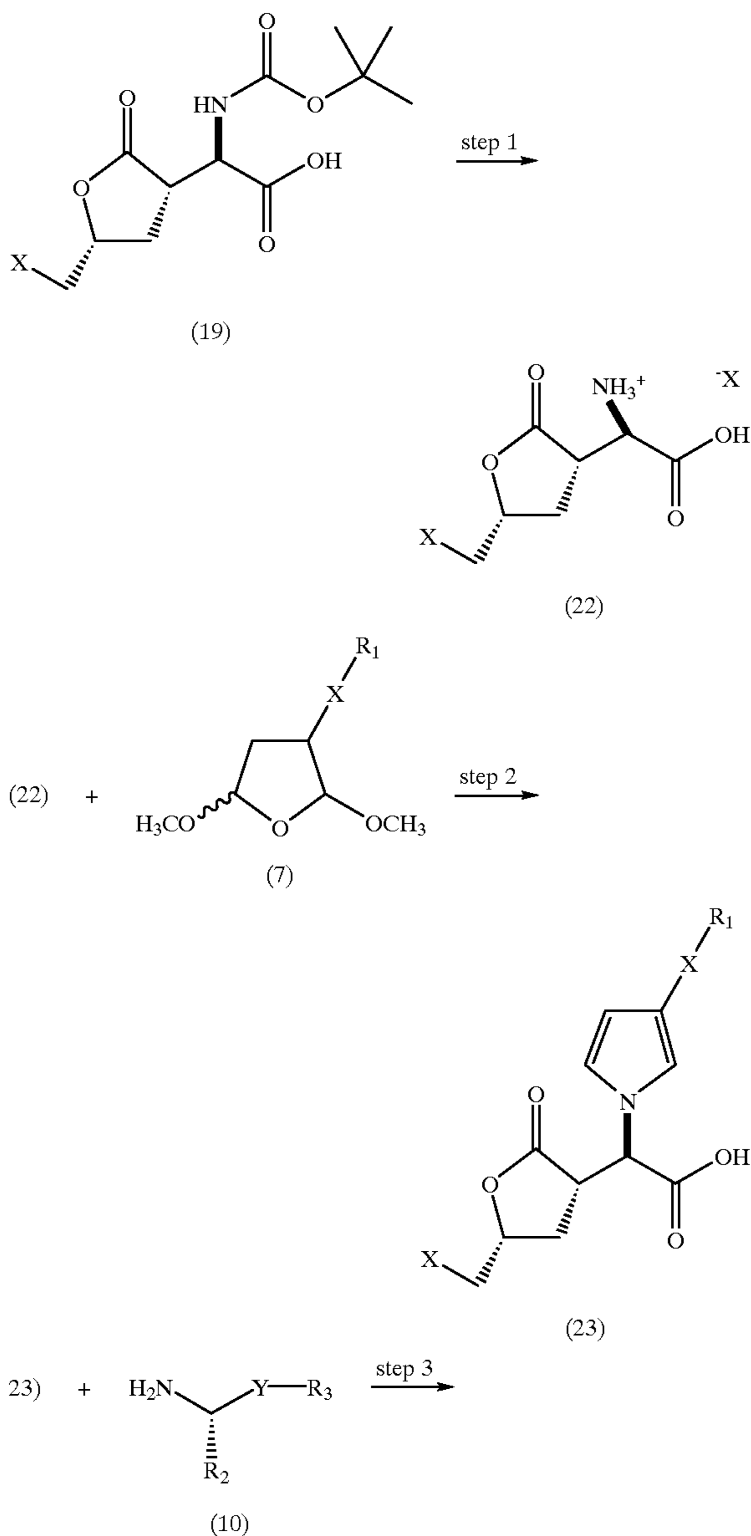
REACTION SCHEME IX
