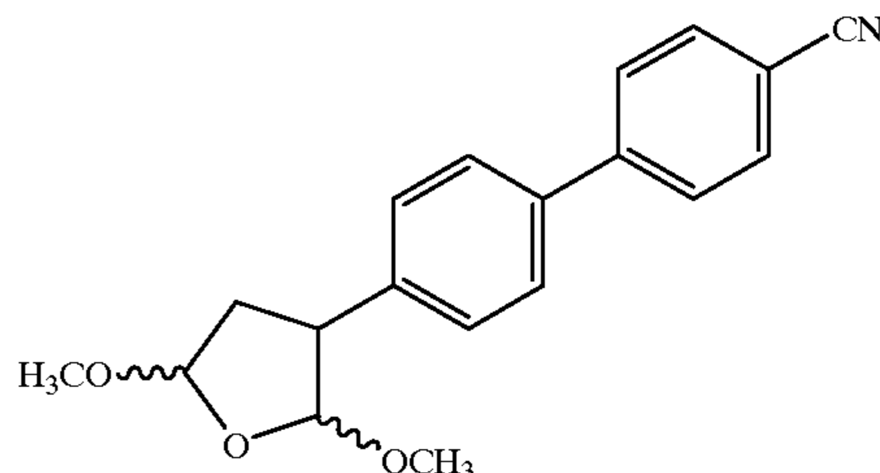
4'-(2,5-Dimethoxy-tetrahydrofuran-3-yl)-biphenyl-4-carbonitrile
