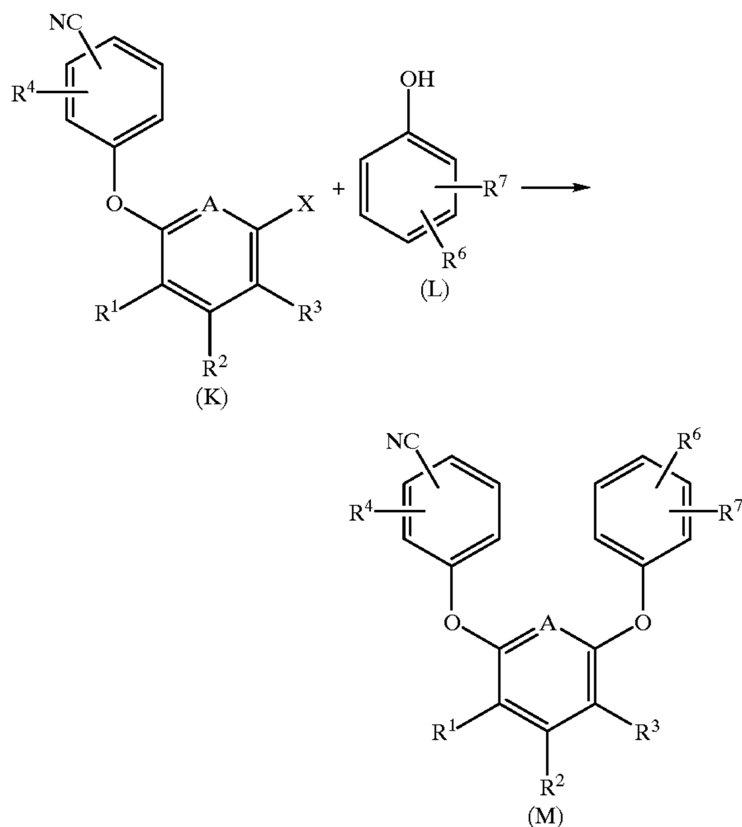
REACTION SCHEME 4
