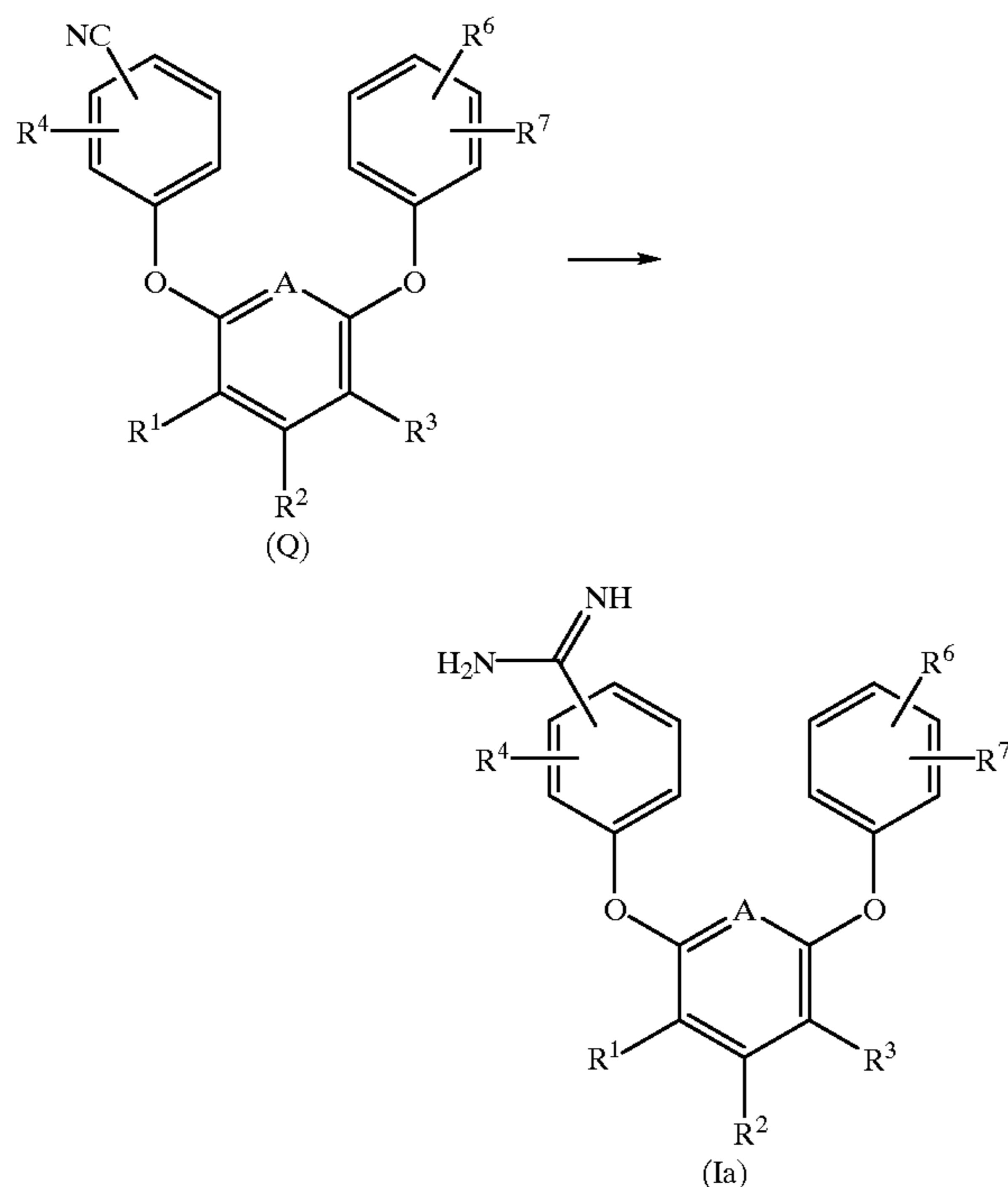
REACTION SCHEME 6
