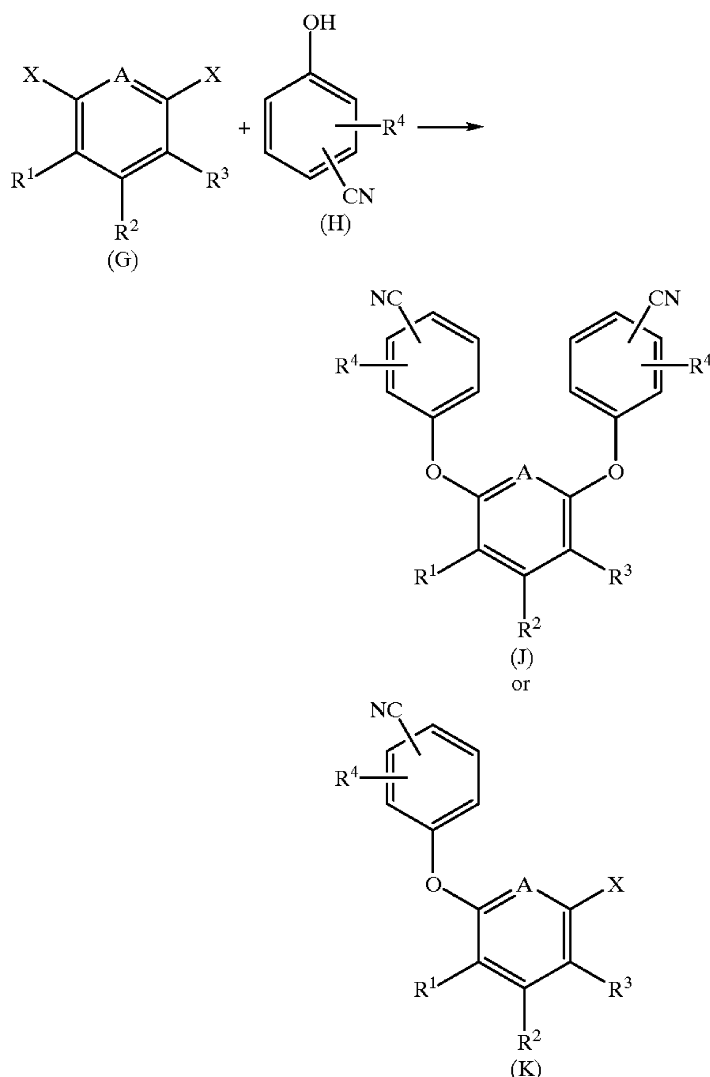
REACTION SCHEME 3
