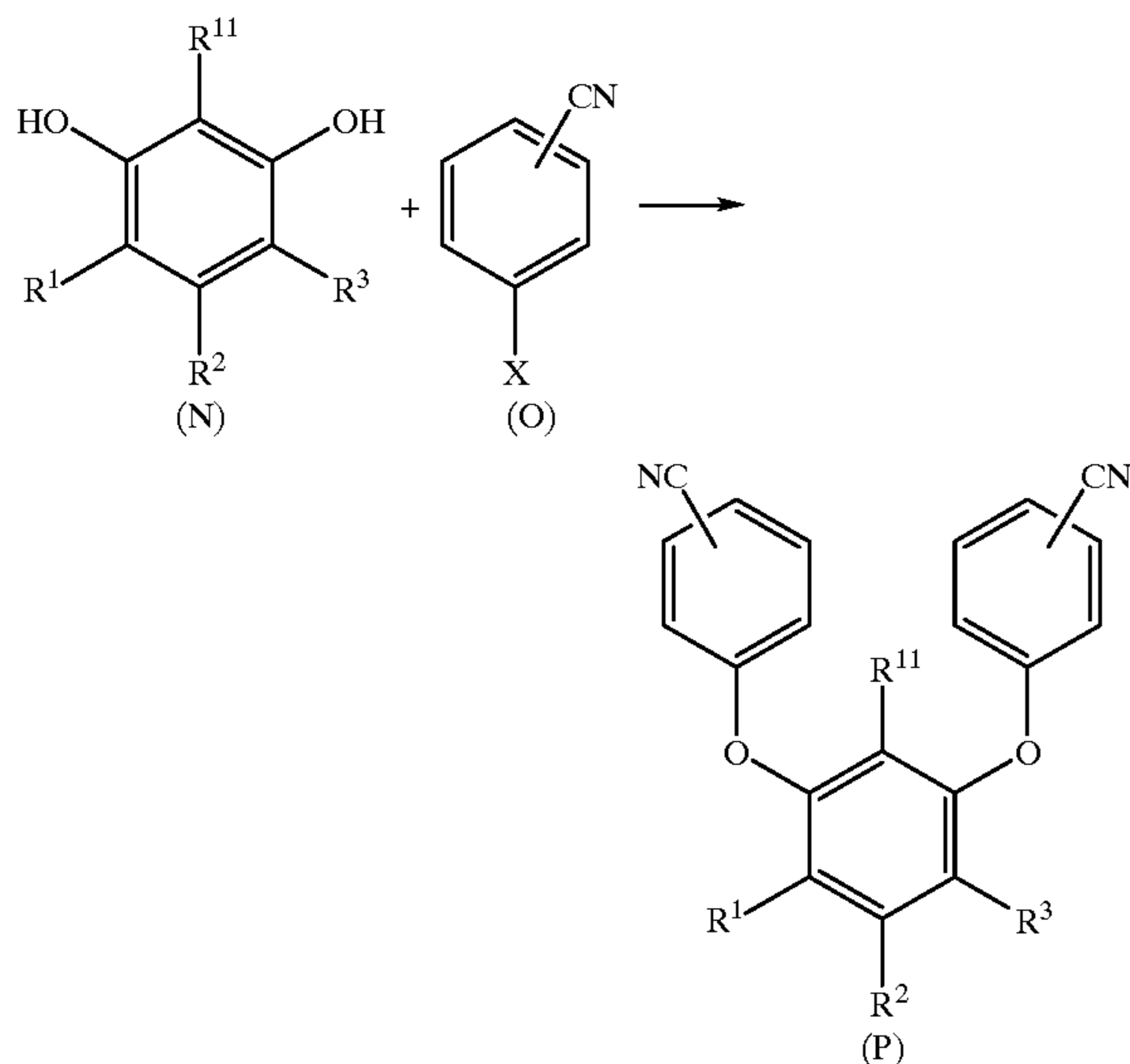
REACTION SCHEME 5
