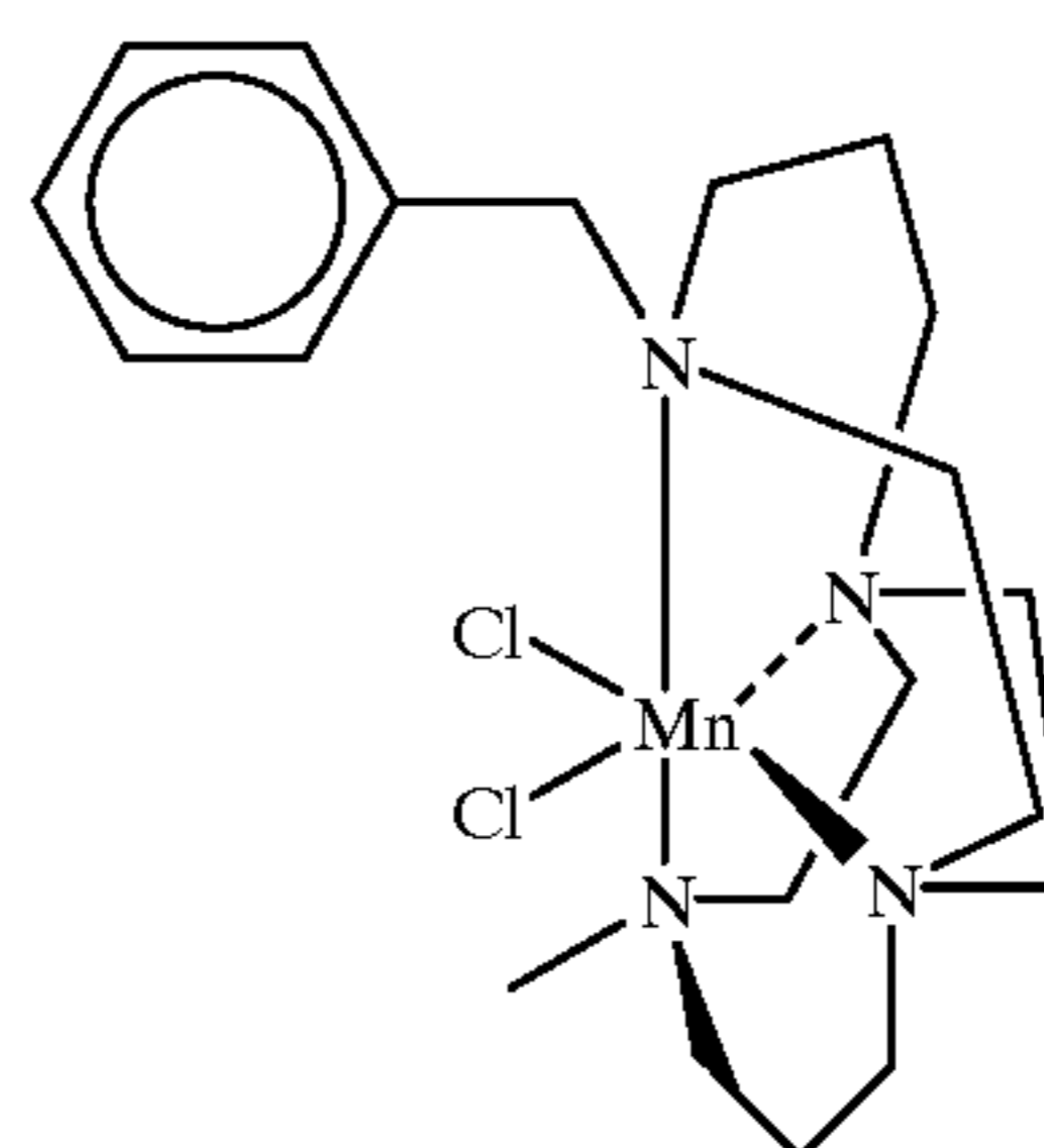
(a) Bz-Bcyclam Synthesis
