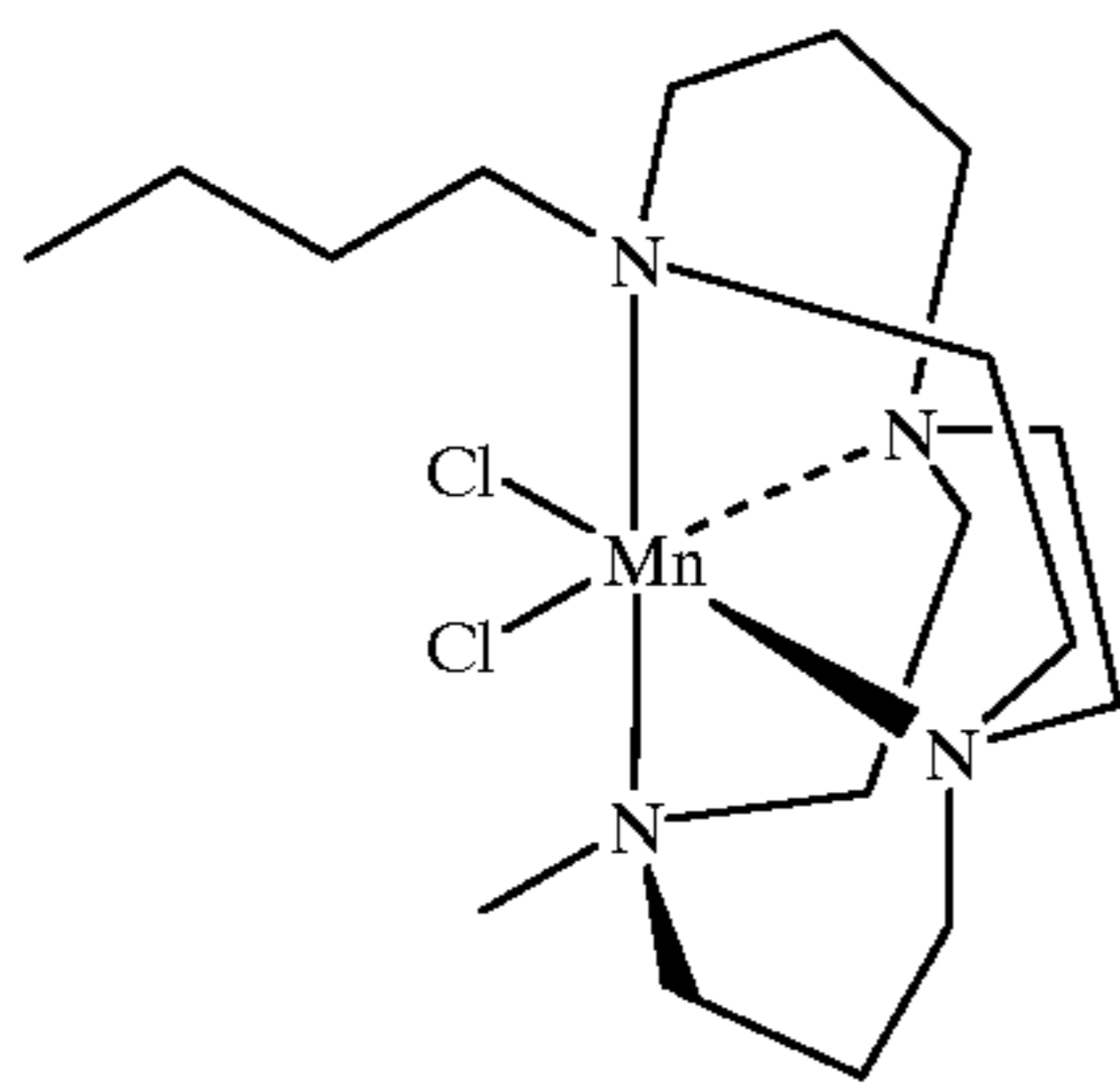
(a) C 4 -Bcyclam Synthesis
