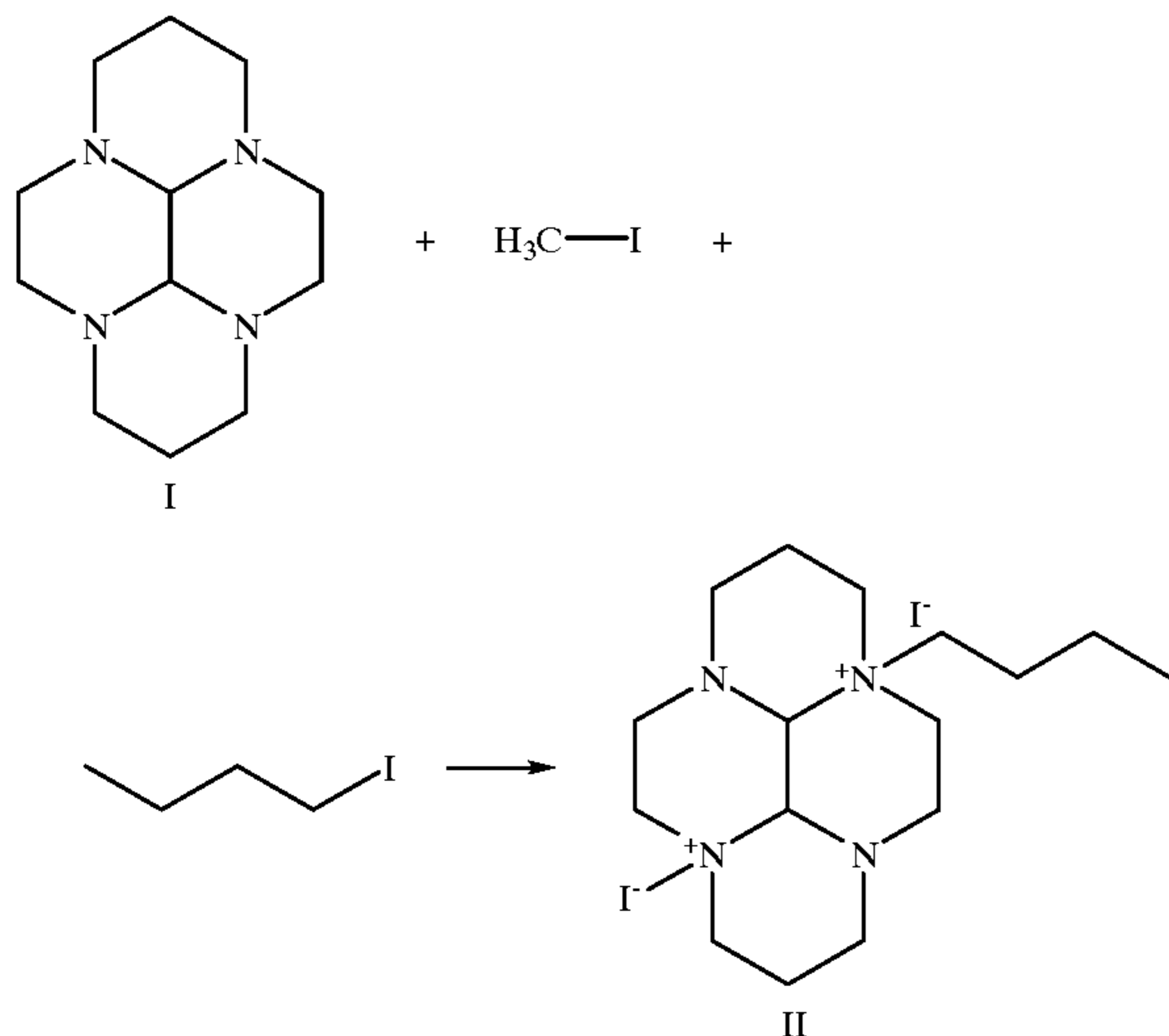
(a) C 4 -Bcyclam Synthesis
