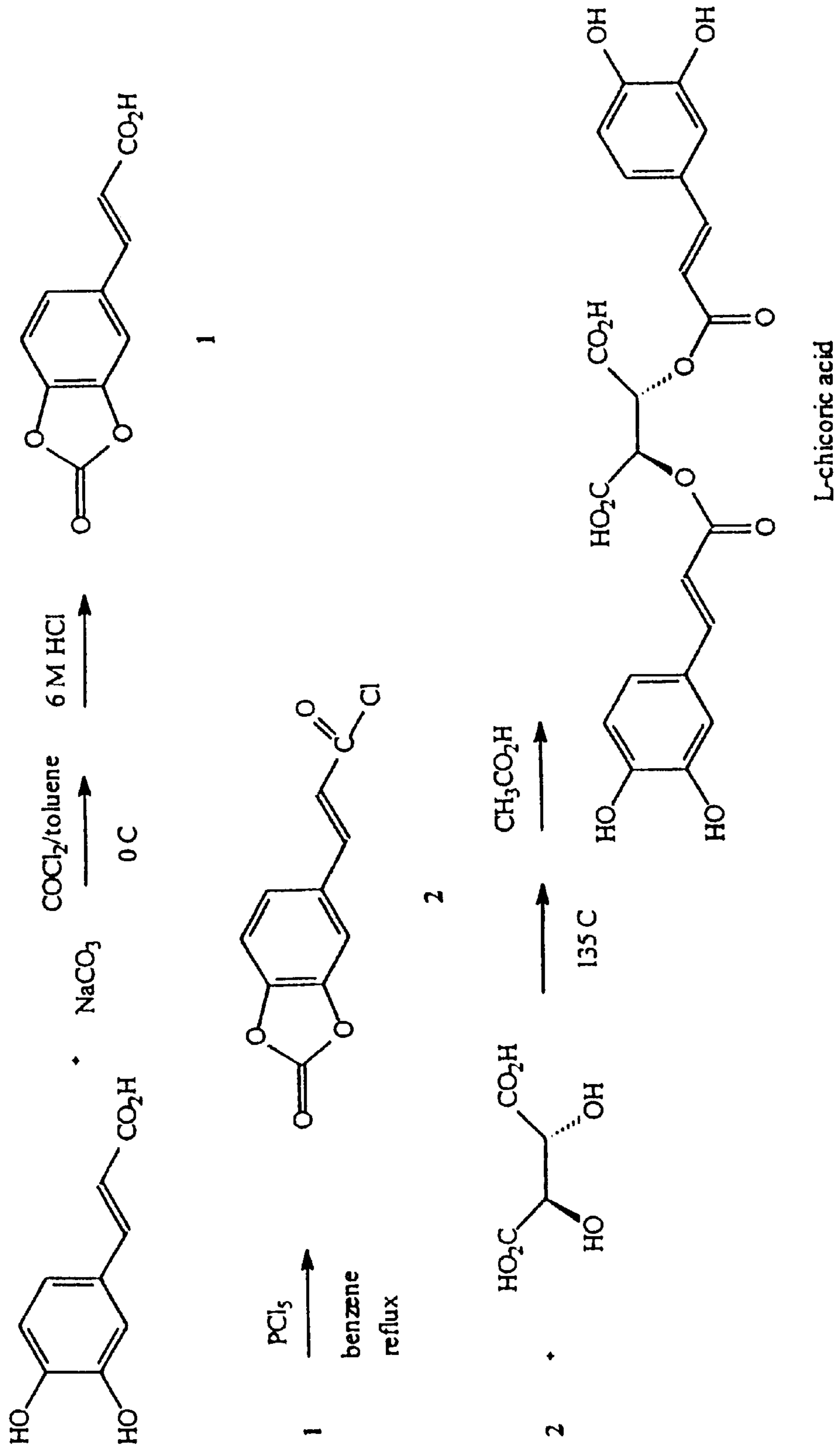
Scheme 1 Synthesis of L-chichoric acid
