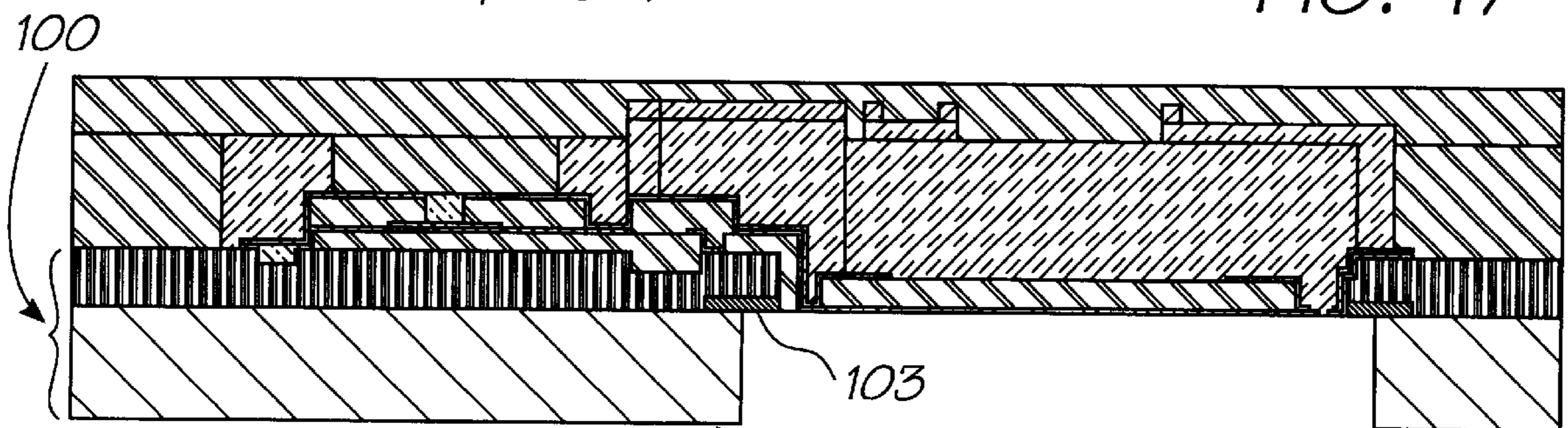
Back-etch using Bosch process
