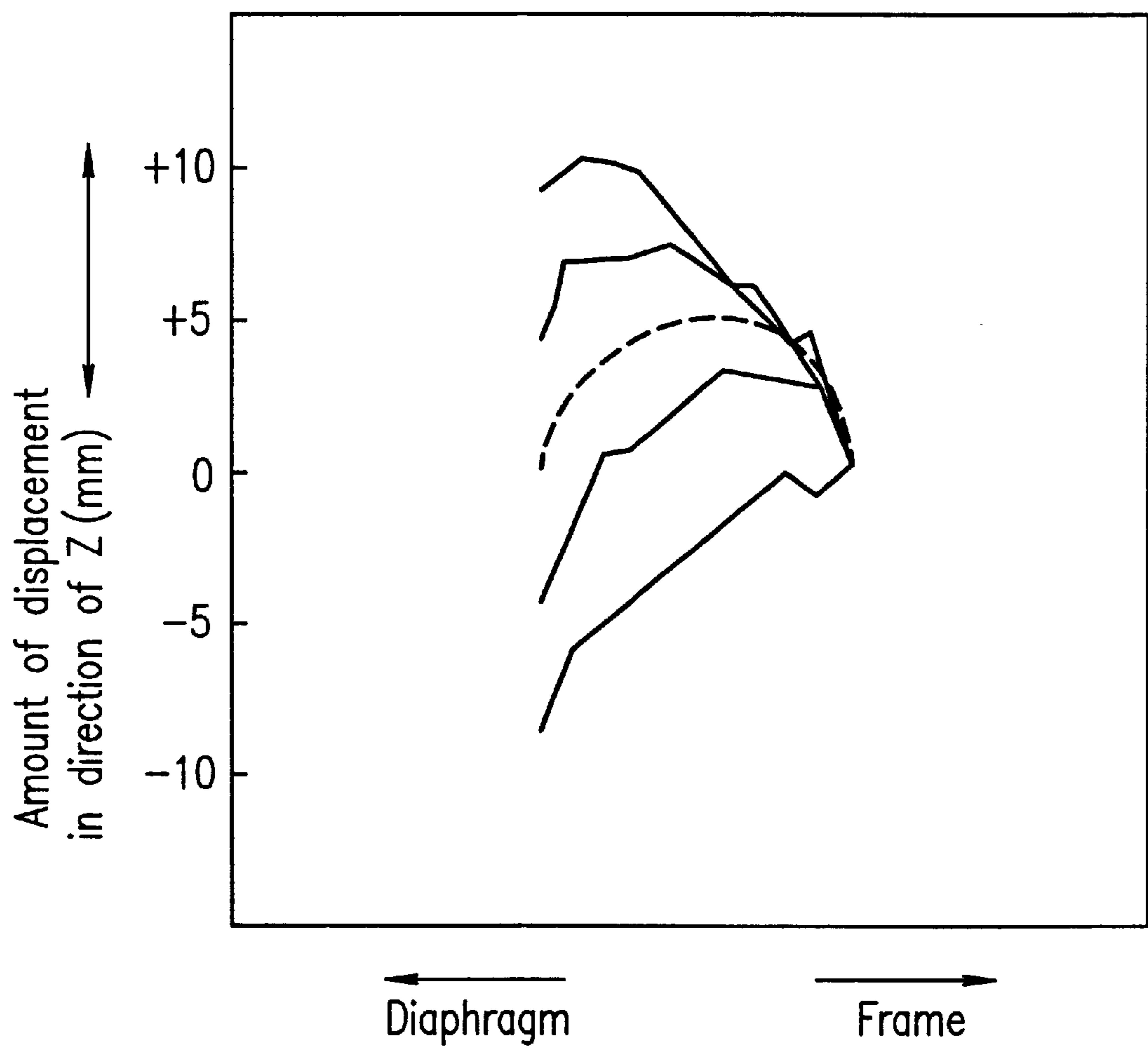
FIG. 11 PRIOR ART
