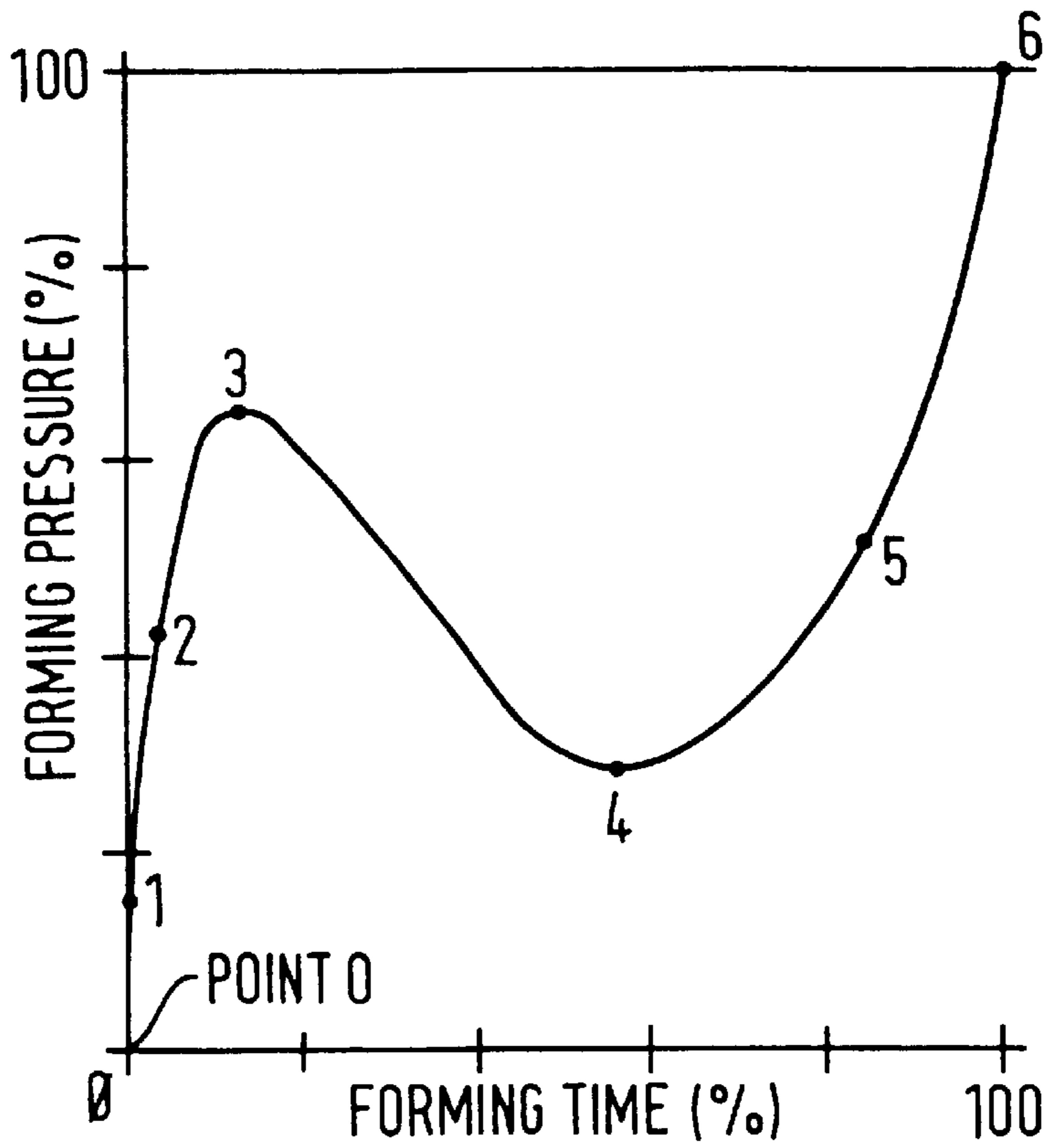
FIG. 3 PRIOR ART
