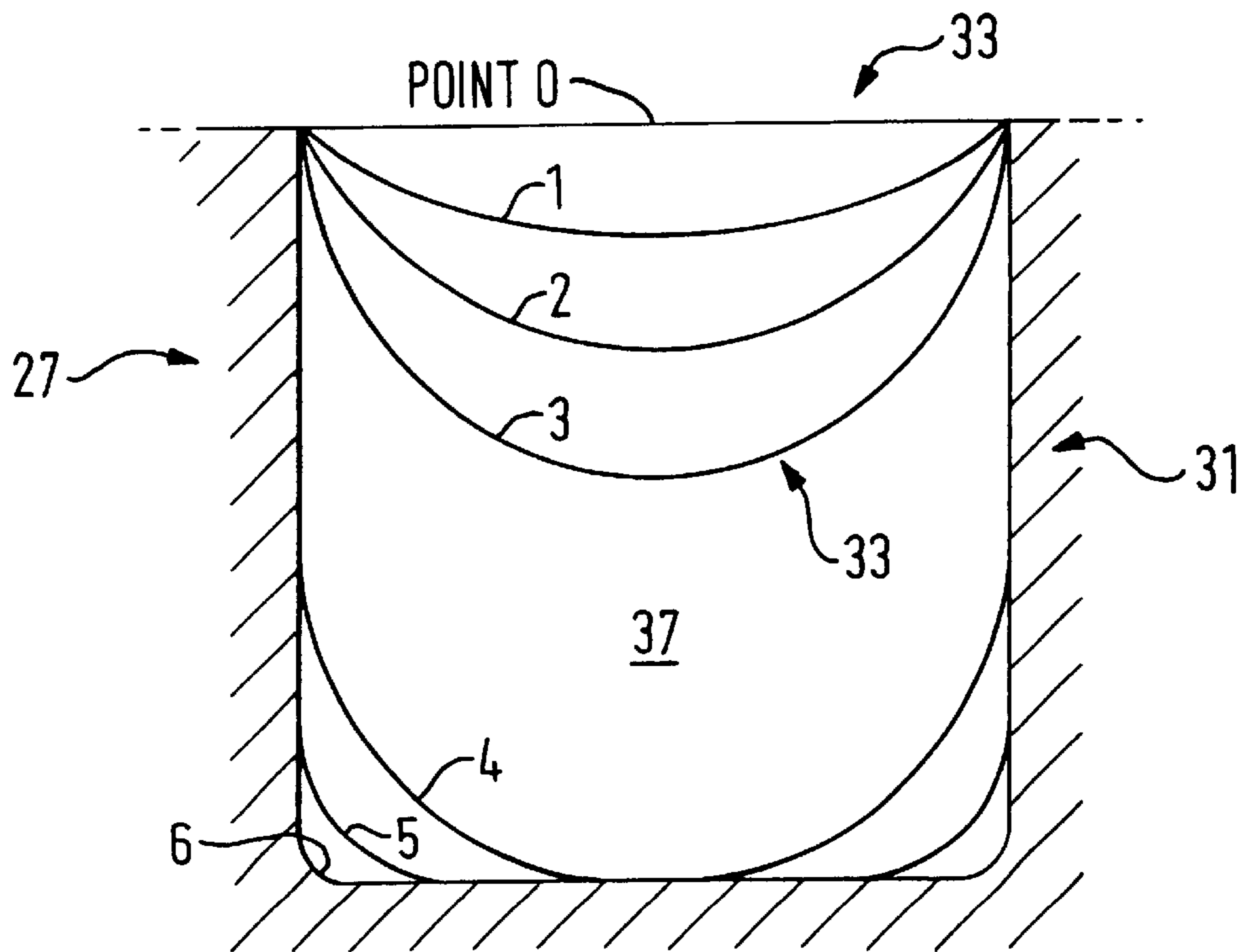
FIG. 2 PRIOR ART
