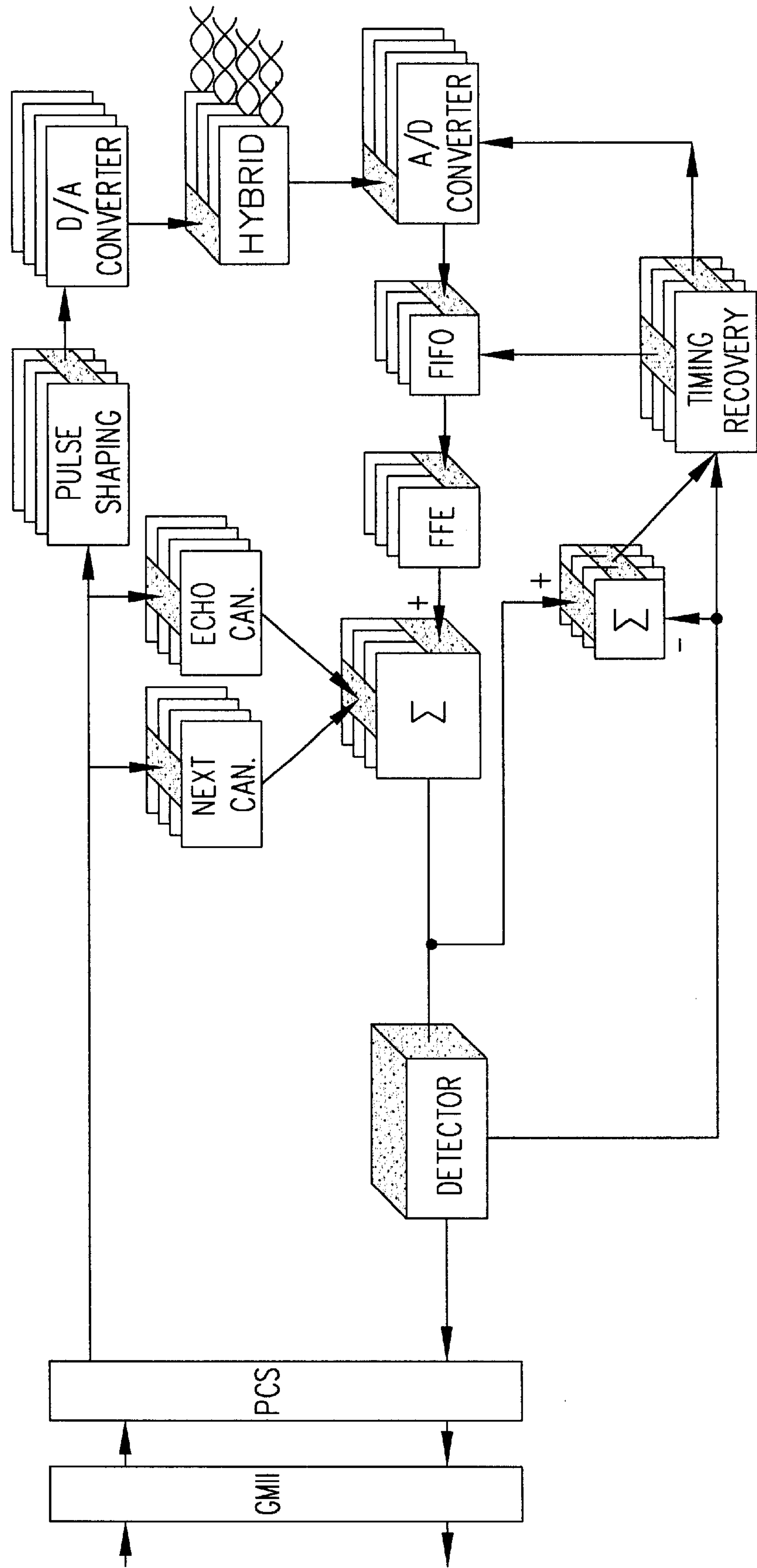
FIG. 6 PRIOR ART
