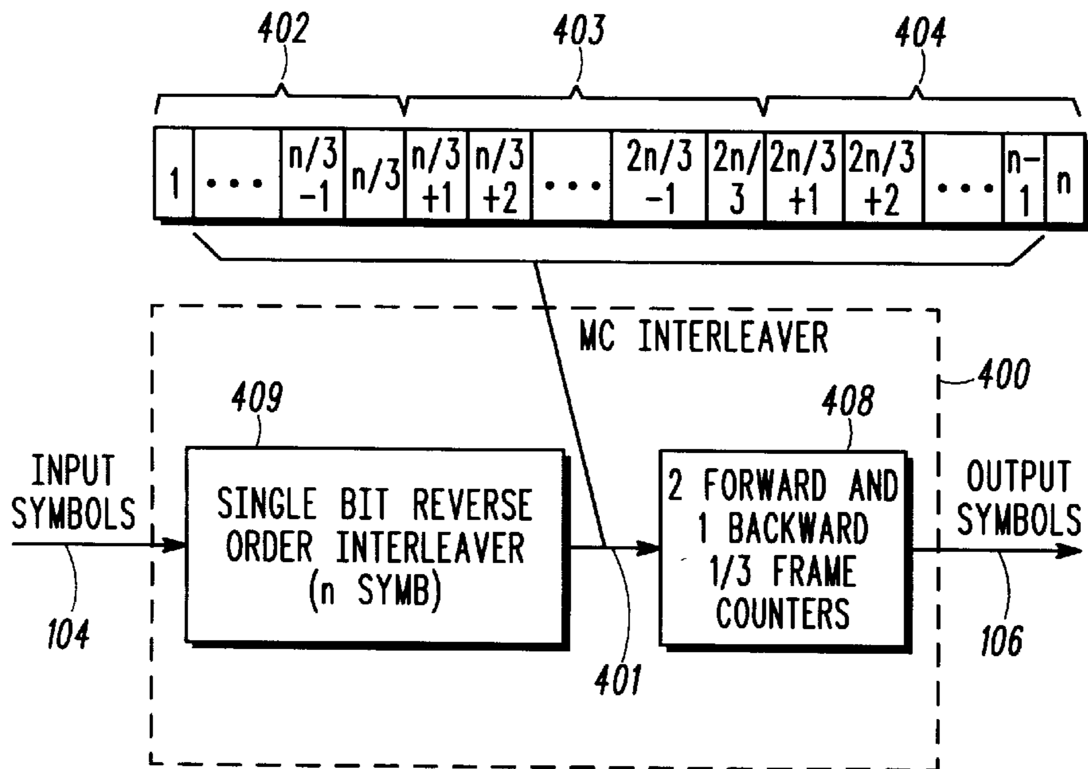
INTERLEAVING SCHEME FOR MC. OTD
