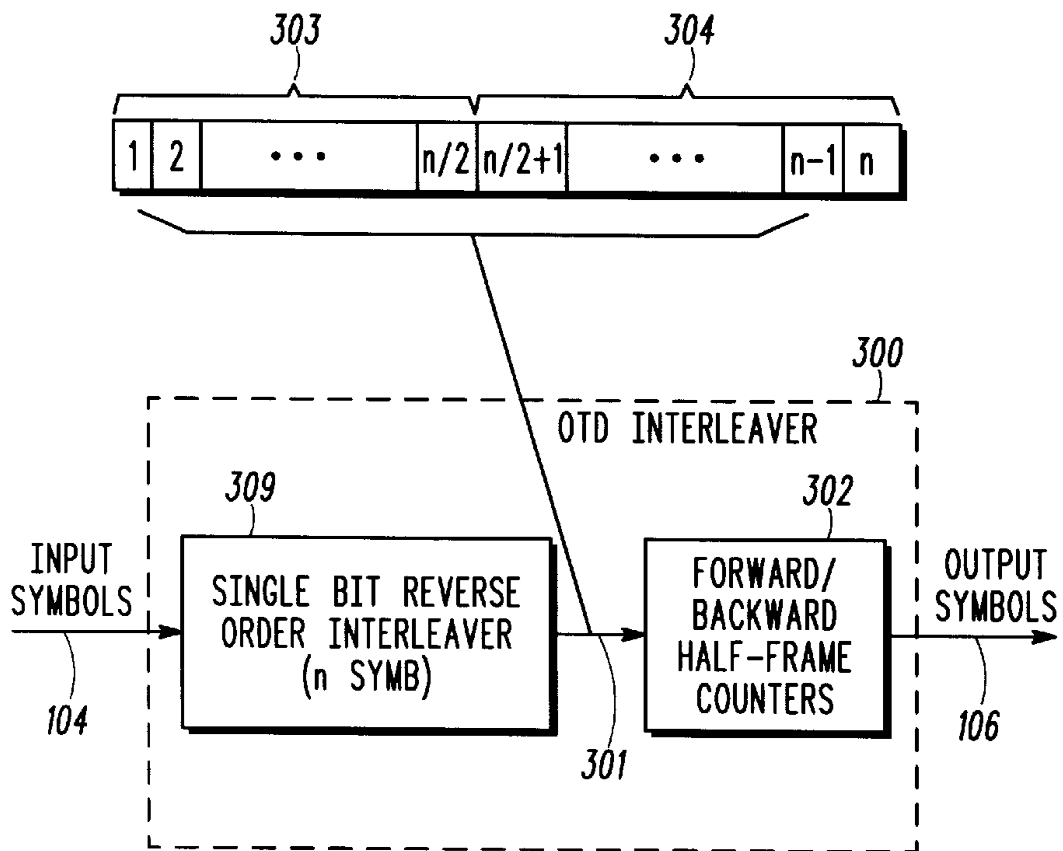
INTERLEAVING SCHEME
