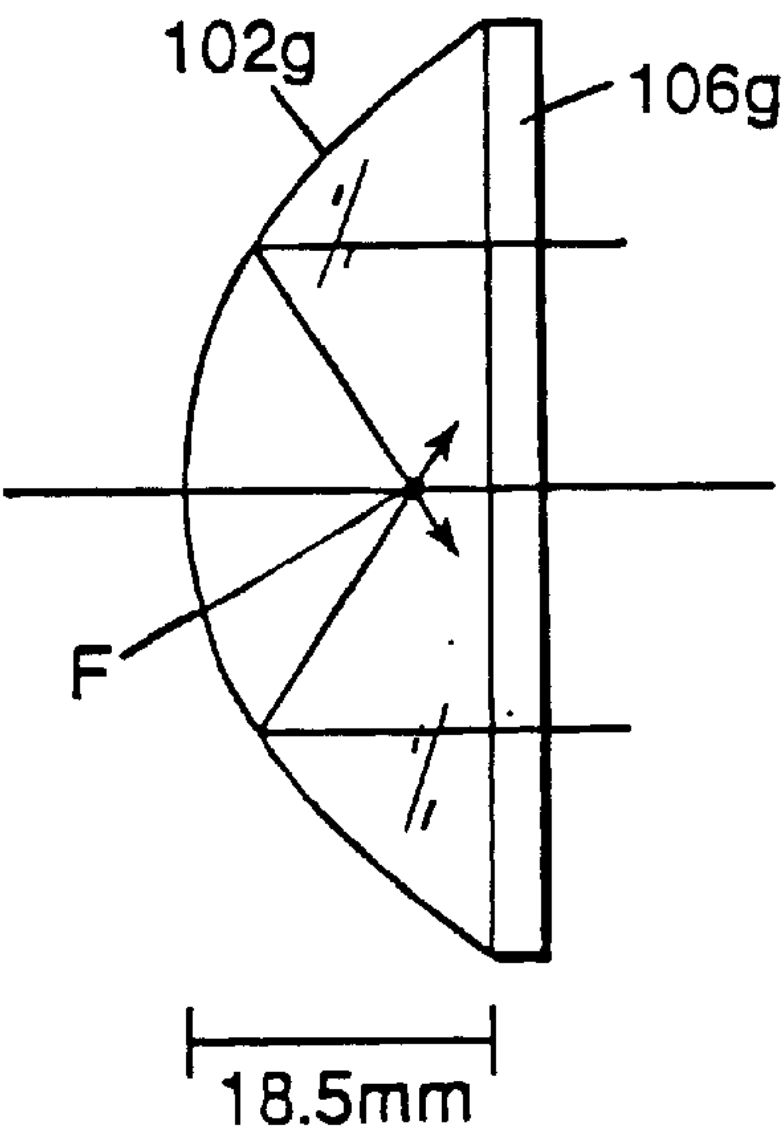
FIG.16 ( PRIOR ART )
