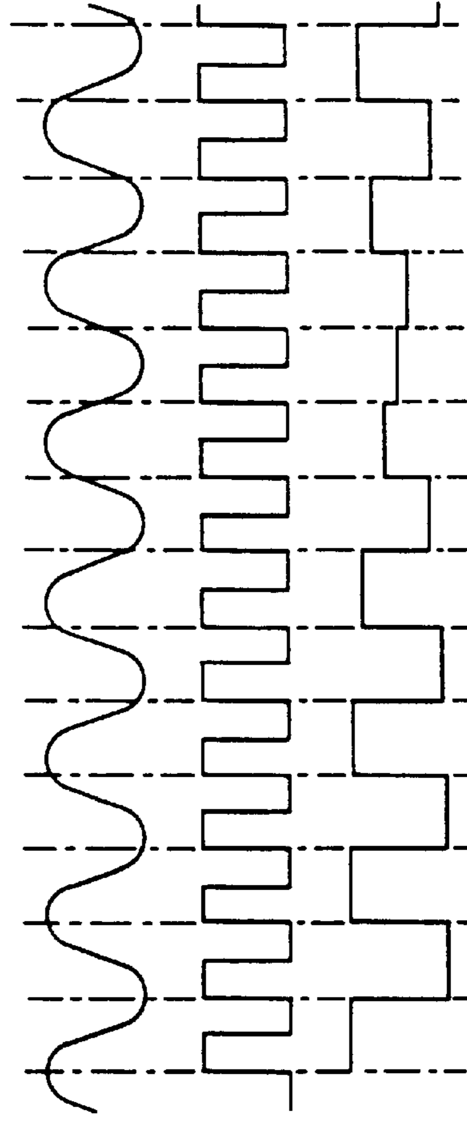
Fig. 44(b-3) DIGITAL VIDEO SIGNAL 110 (IN ANALOG FORM)
