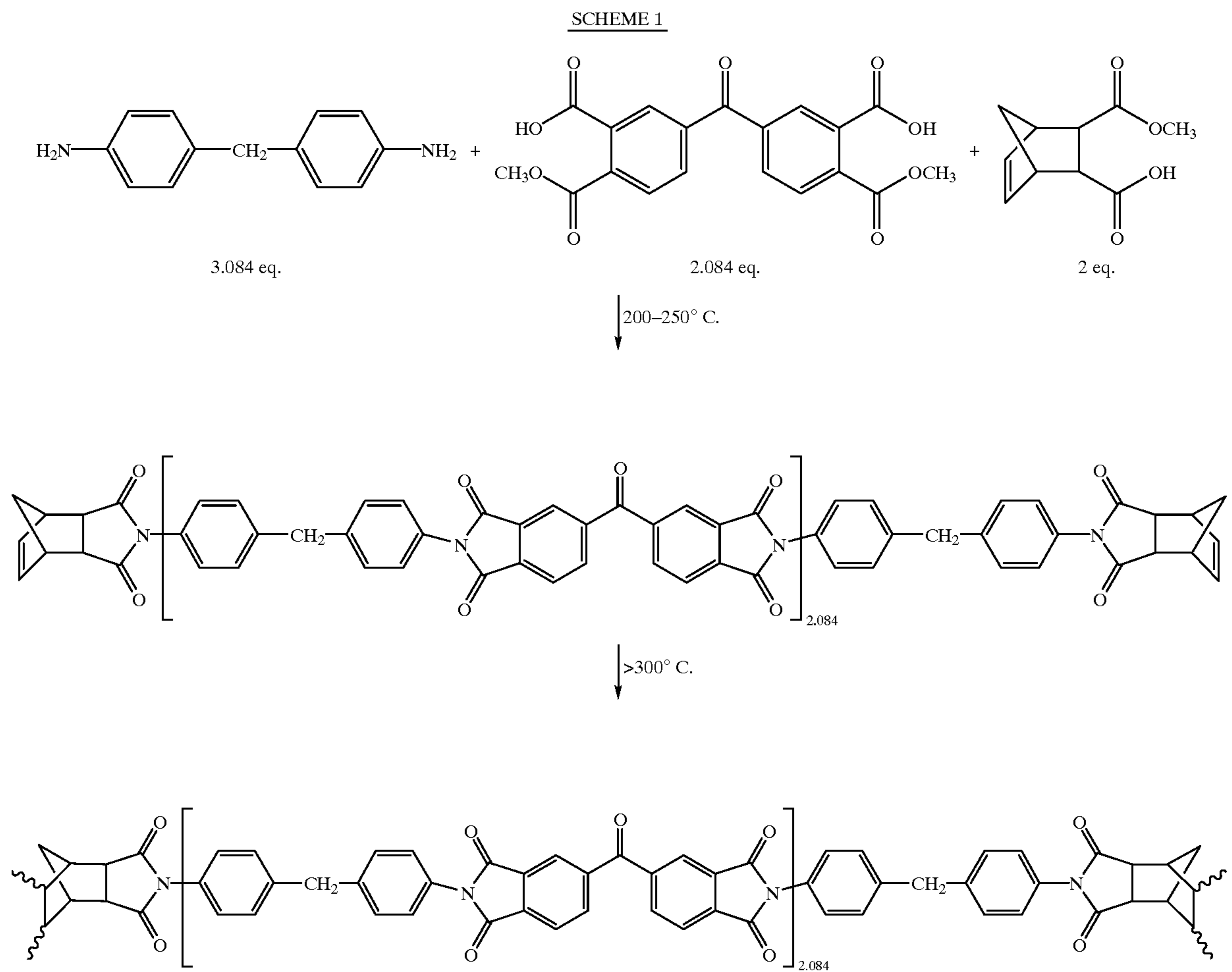
Scheme 1
