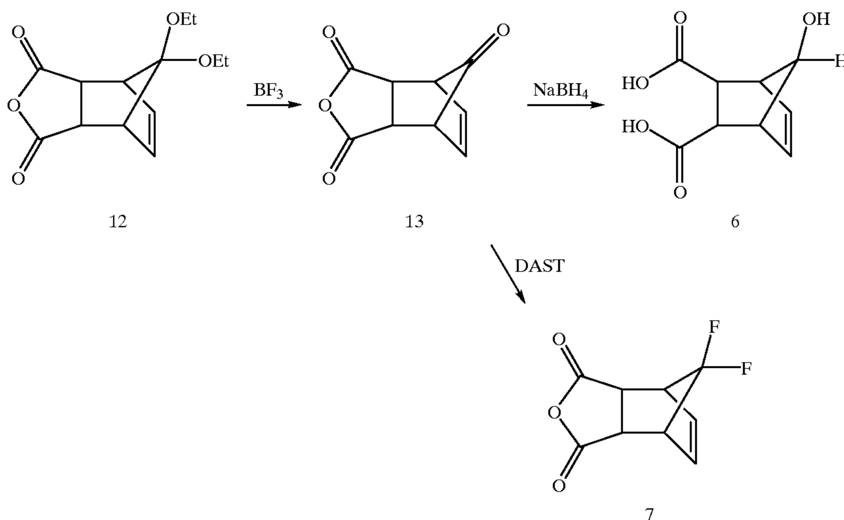
SCHEME 4
