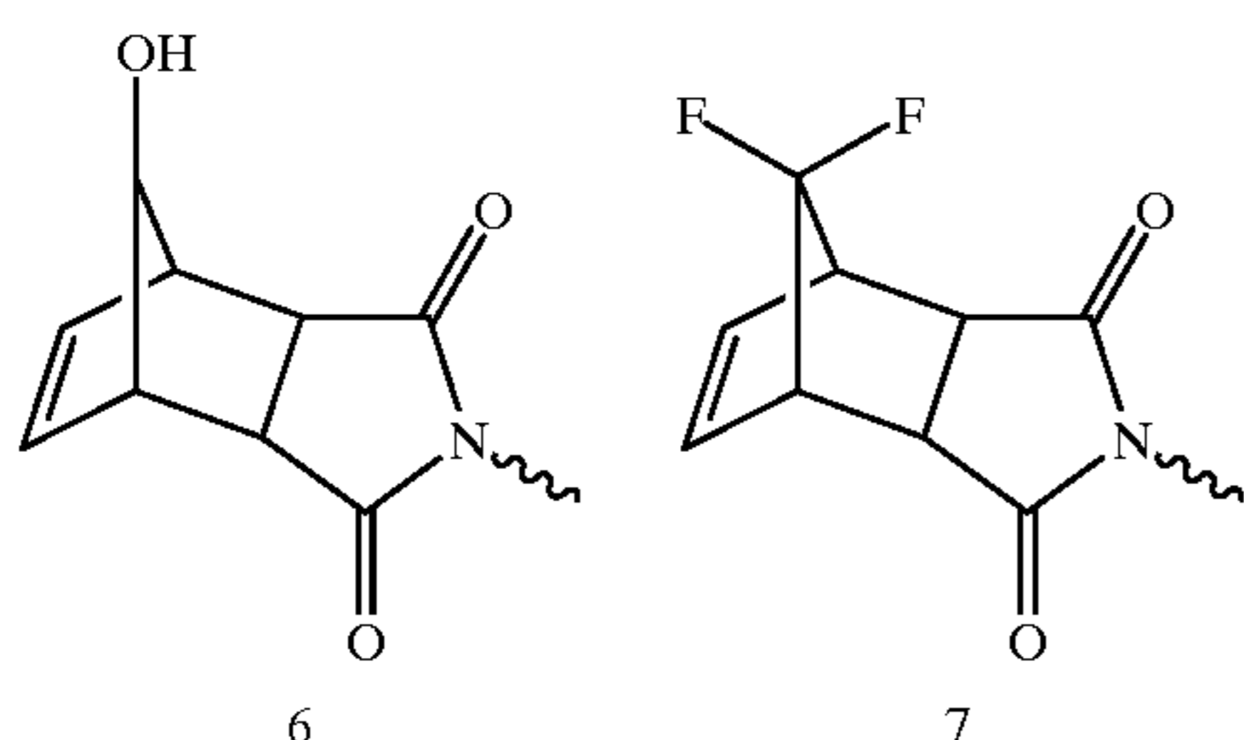
SCHEME 3
