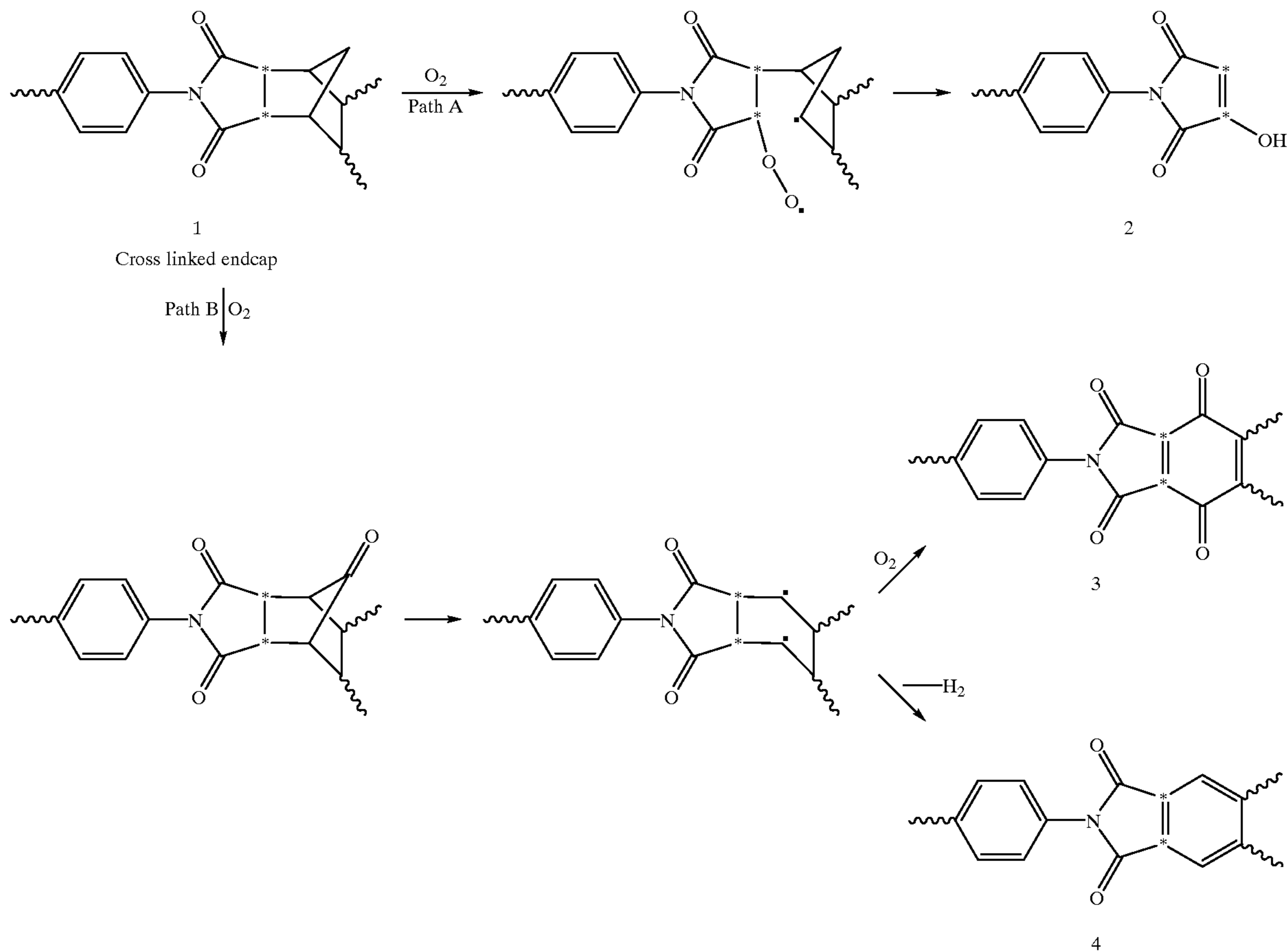
SCHEME 2
