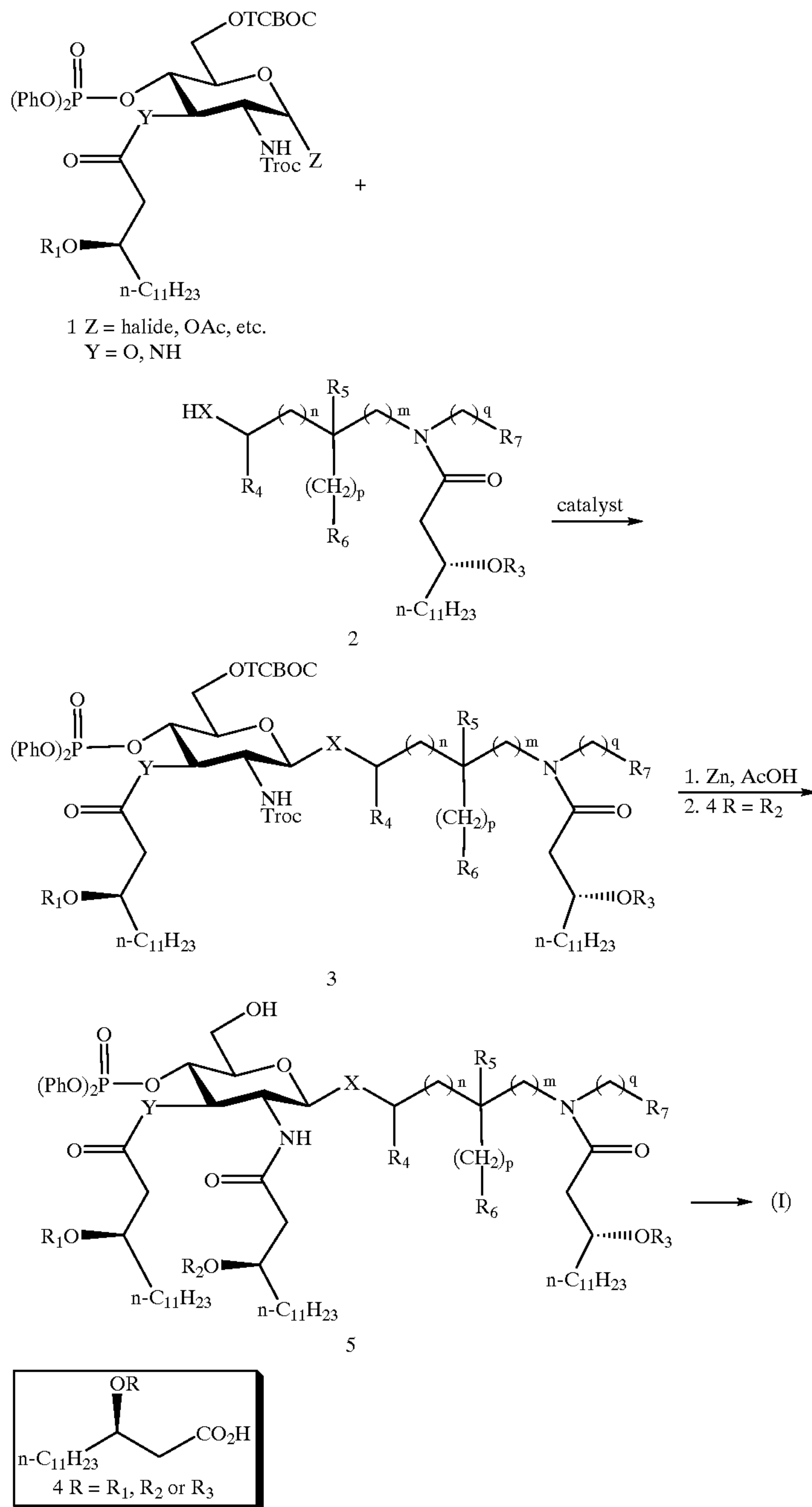
Scheme 1
