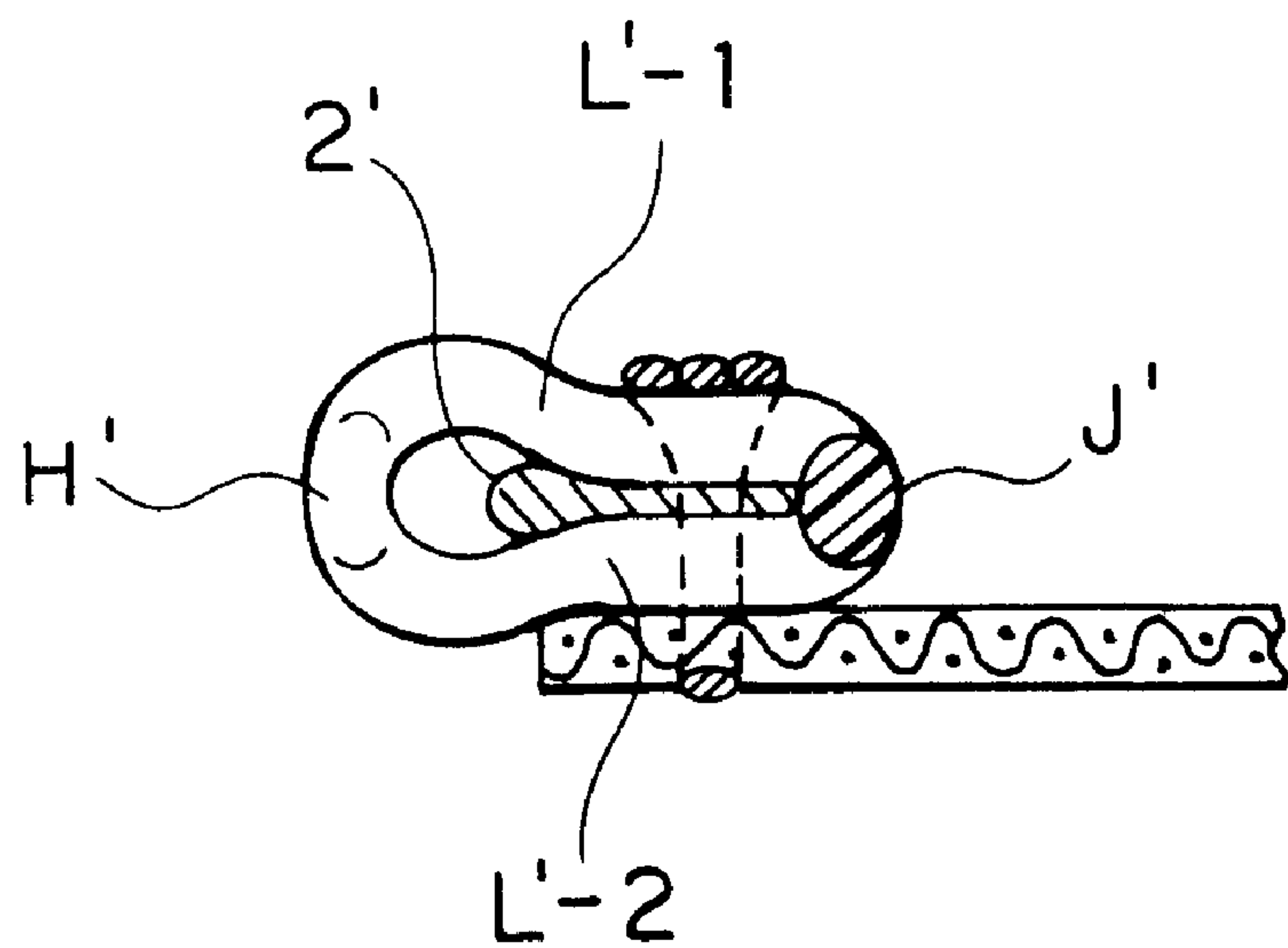
FIG. 11 PRIOR ART
