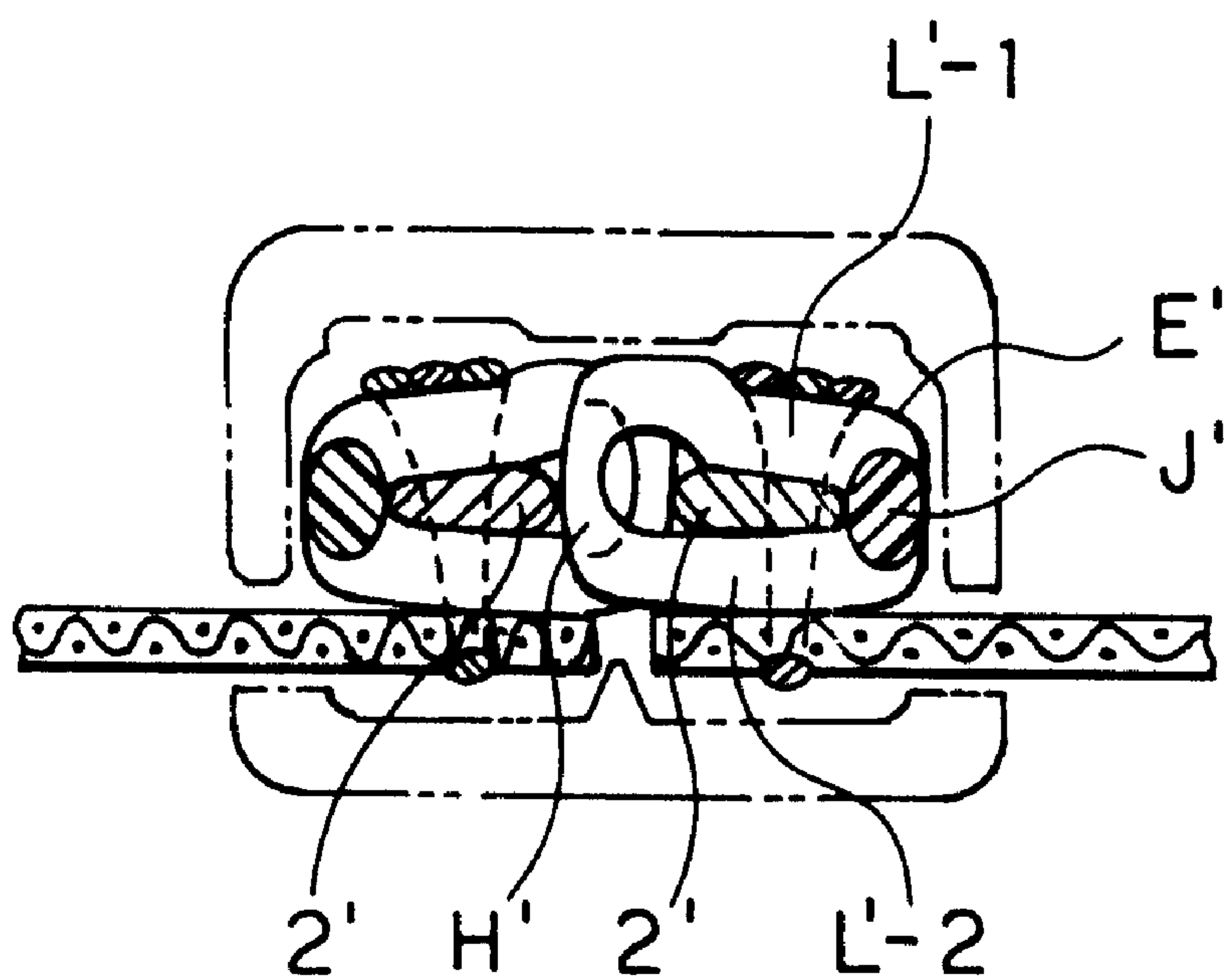
FIG. 12 PRIOR ART
