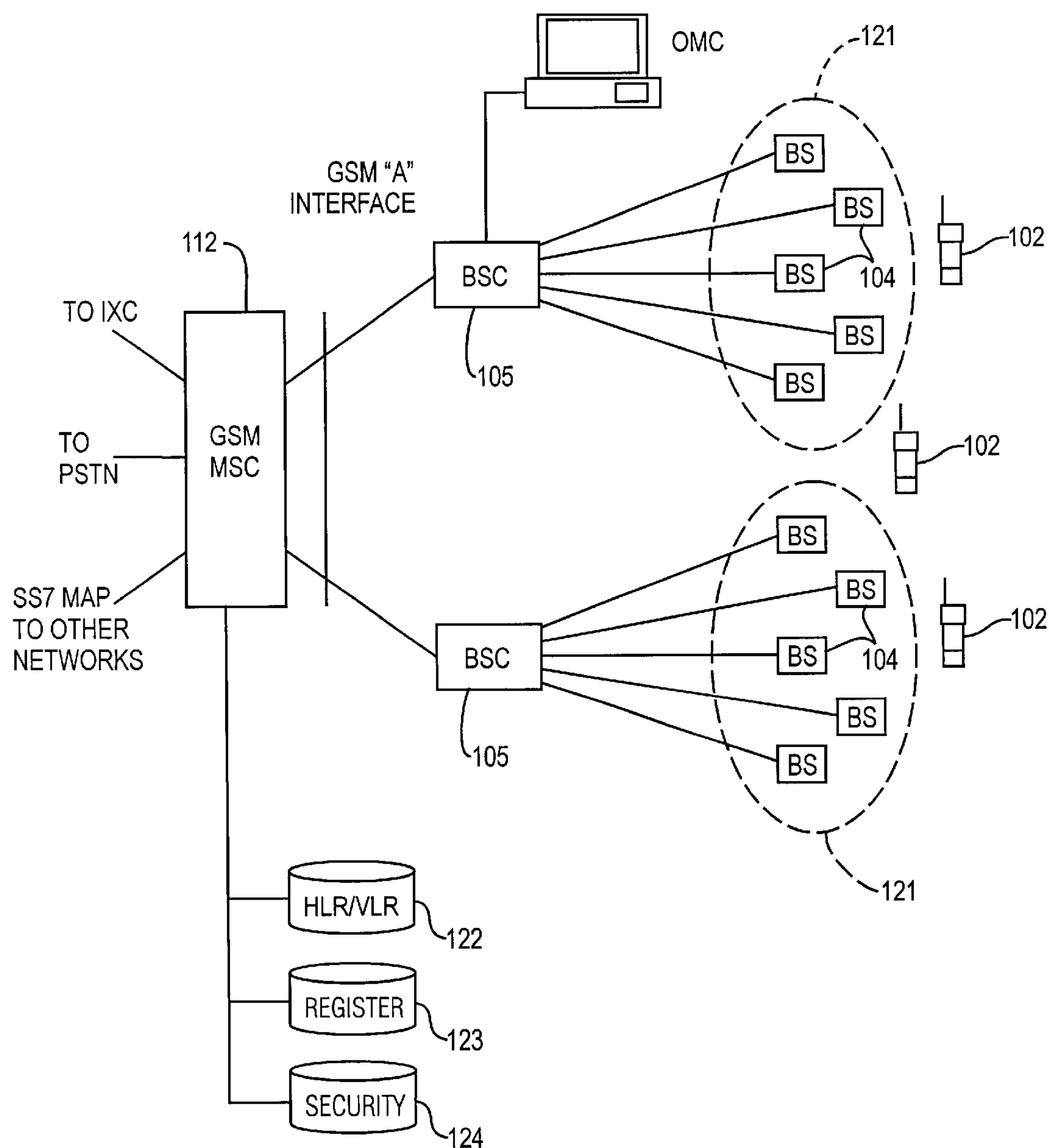
Fig.2A GSM/DSC-1900 BASED NETWORK INTERCONNECTION
