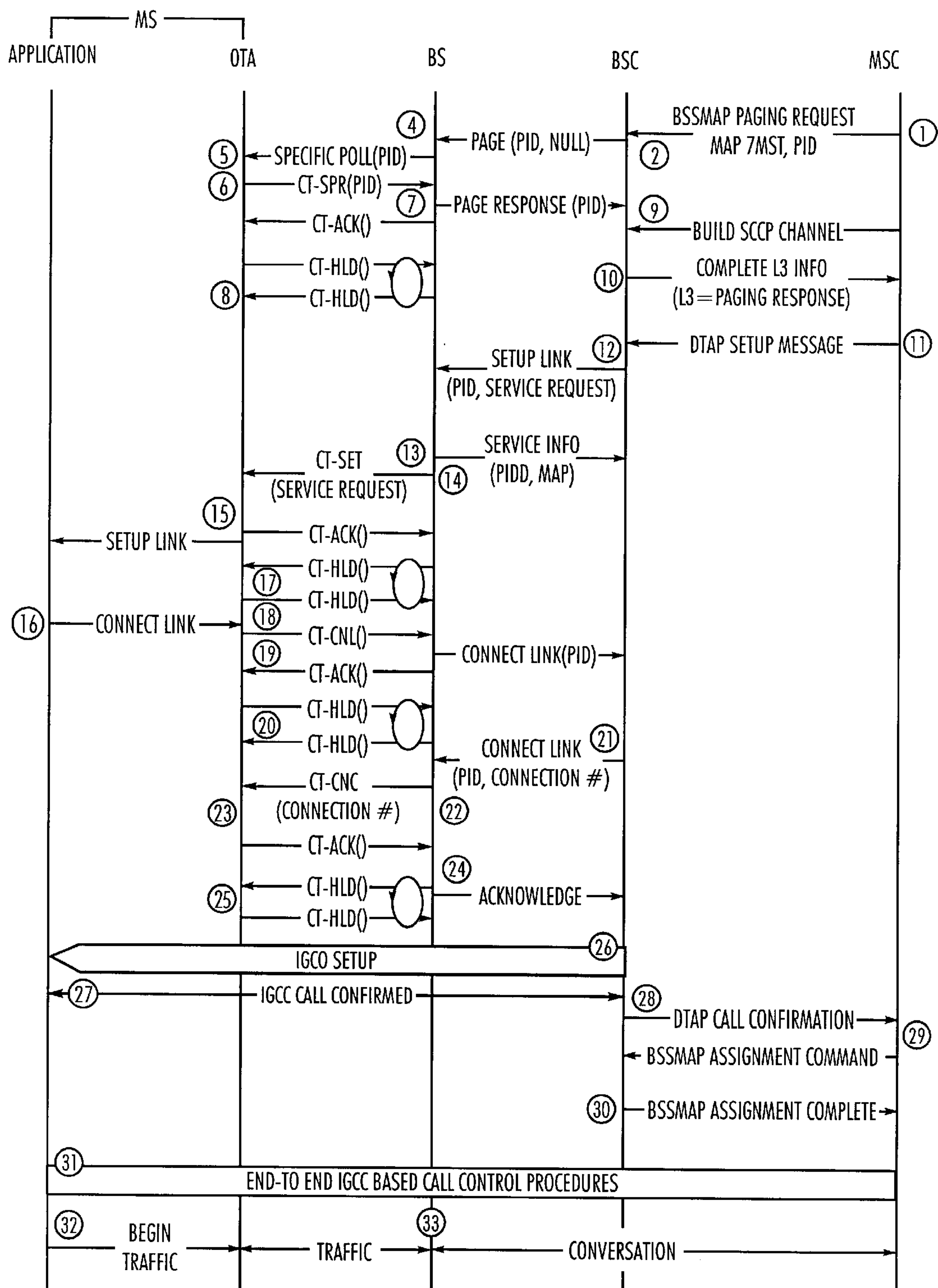
Fig. 10 MOBILE CALL TERMINATION
