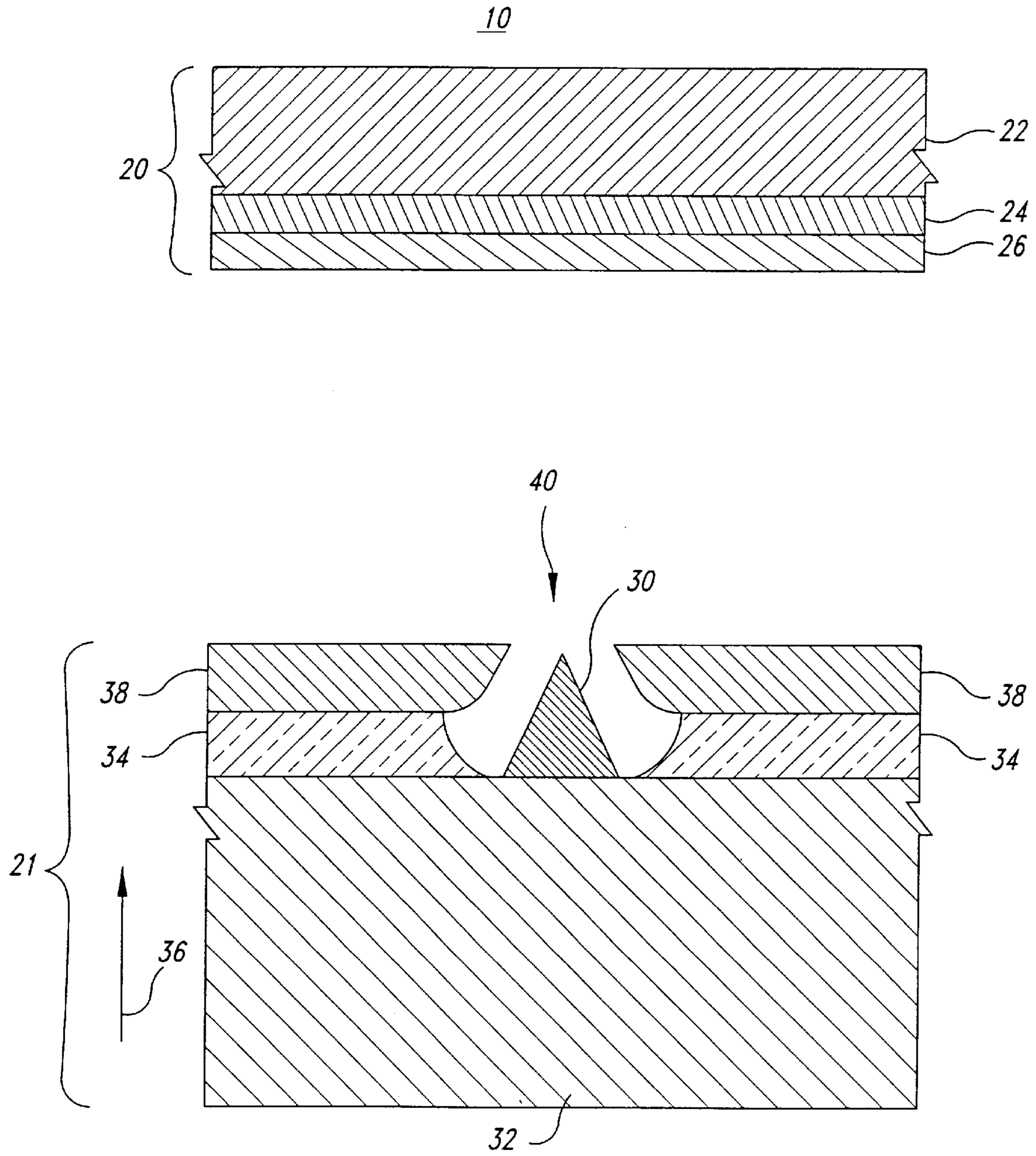
Fig. 1 (PRIOR ART)
