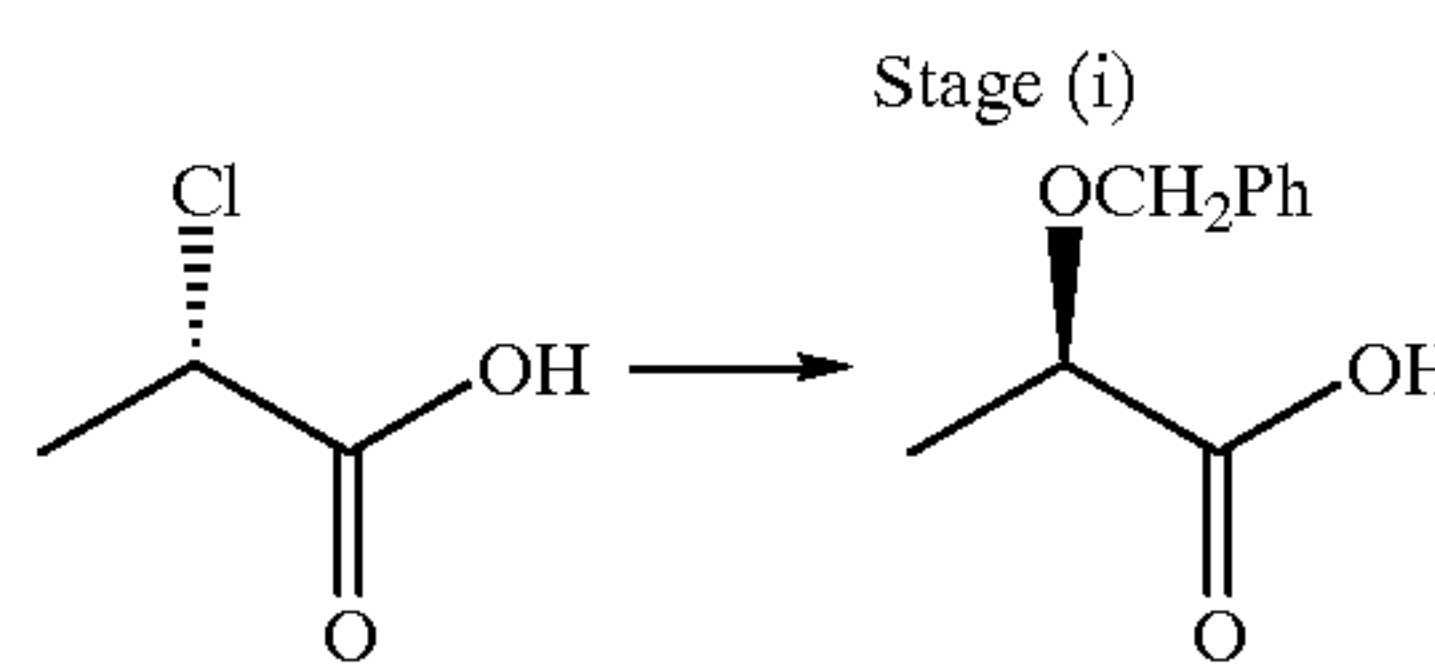
L-2-chloropropionic acid D-2-(benzyloxy)propionic acid
