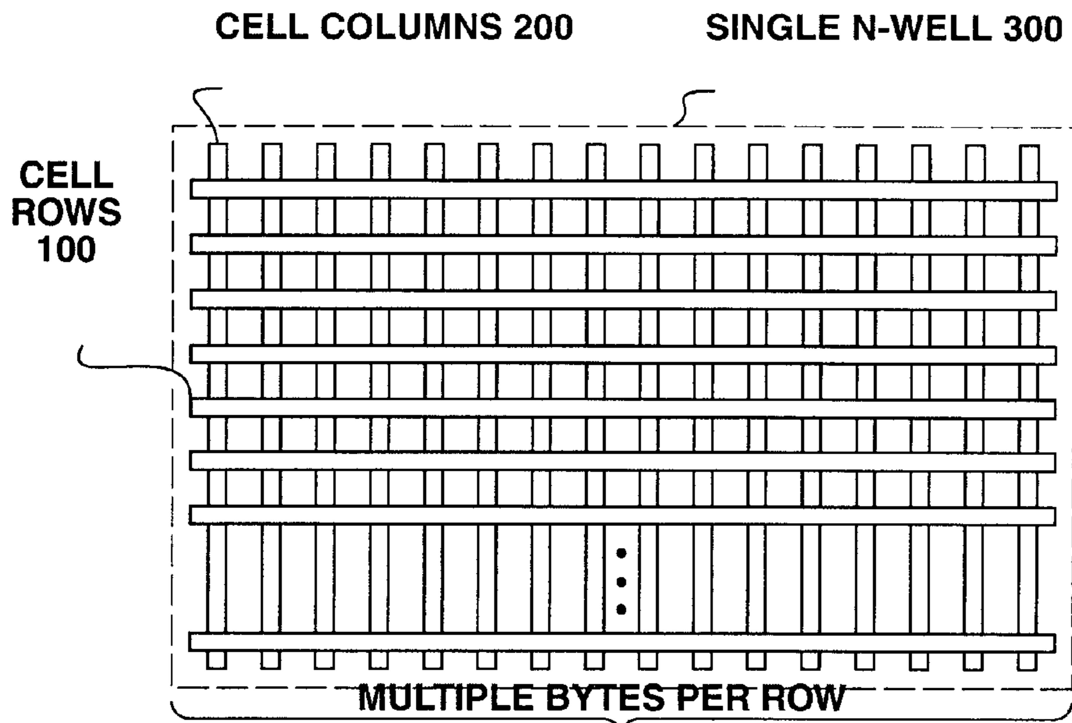
FIG. 3 (PRIOR ART)
