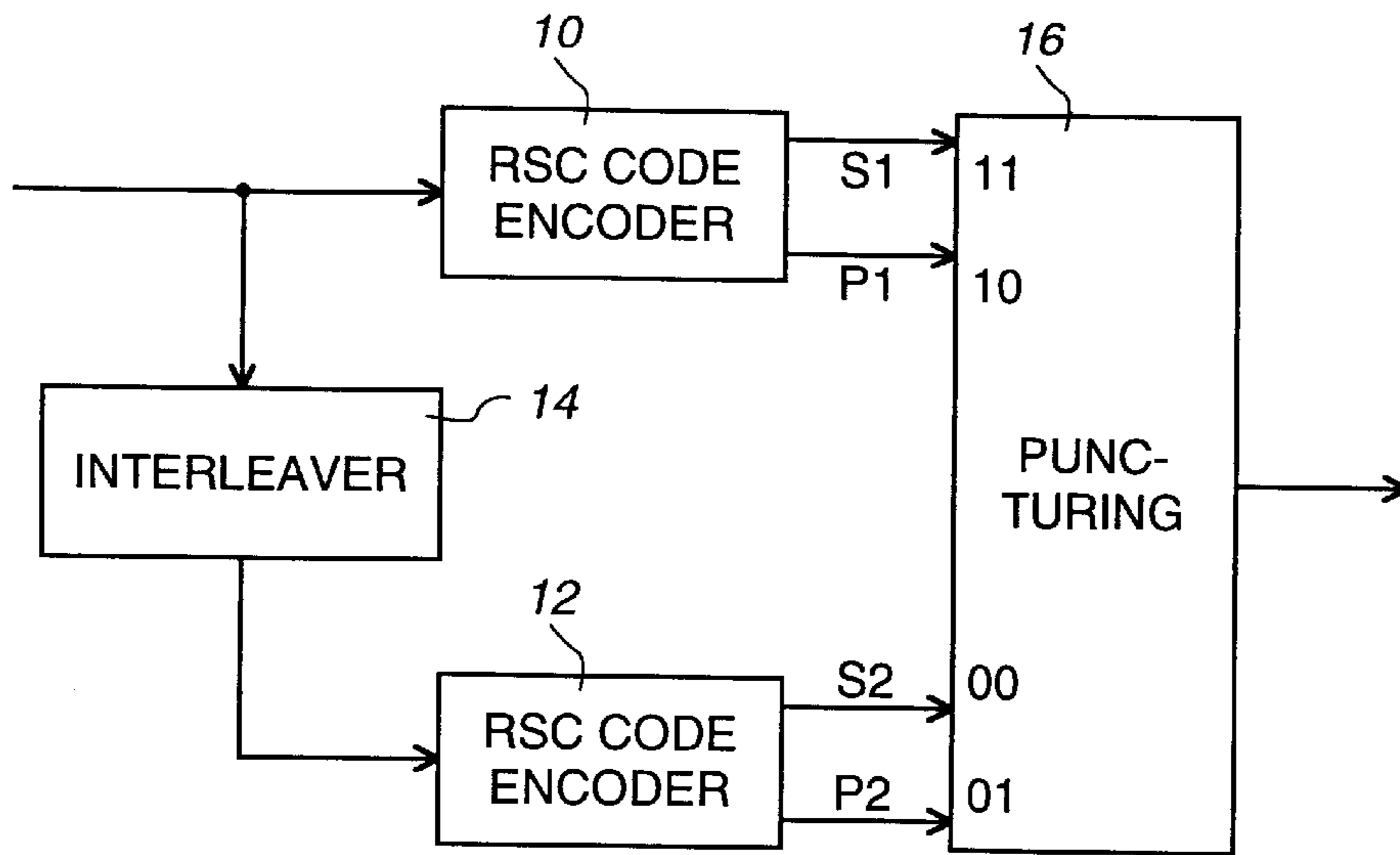
Fig. 1 PRIOR ART
