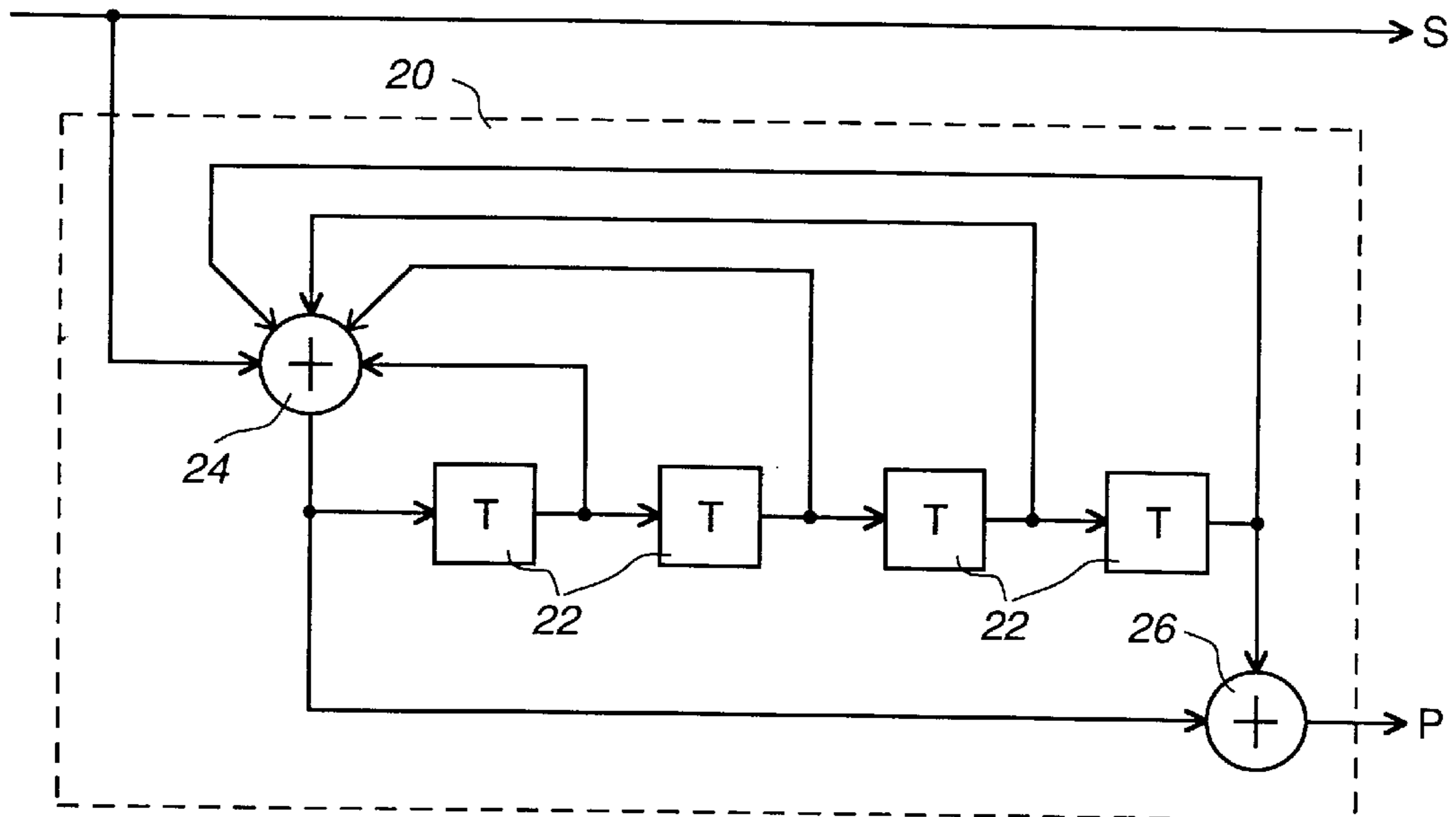
Fig. 2 PRIOR ART
