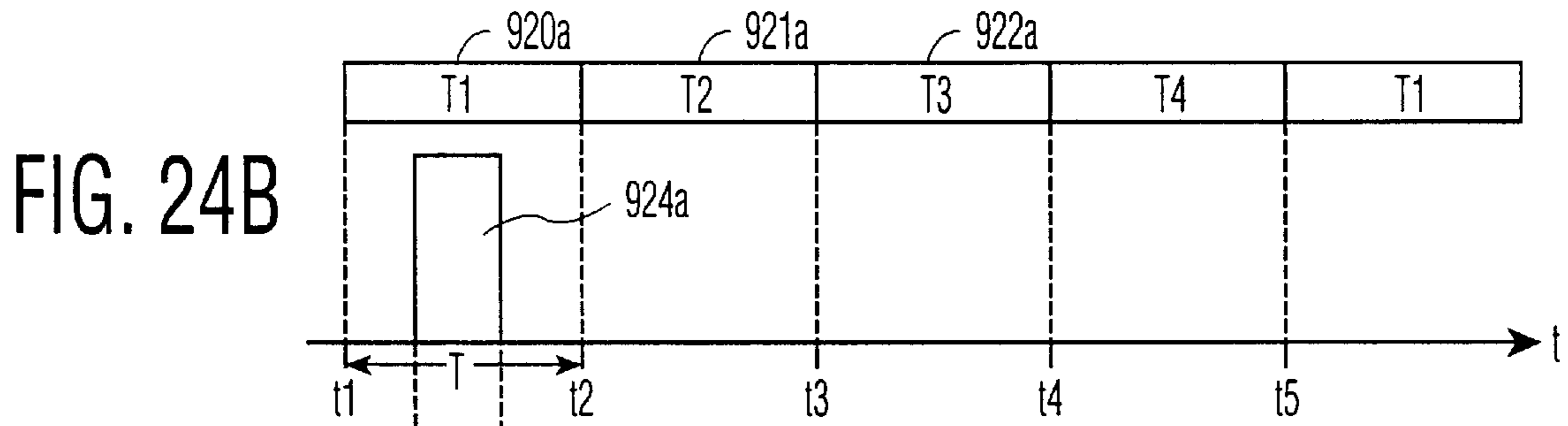
(2) TRIMMING PATTERN OF "00"
