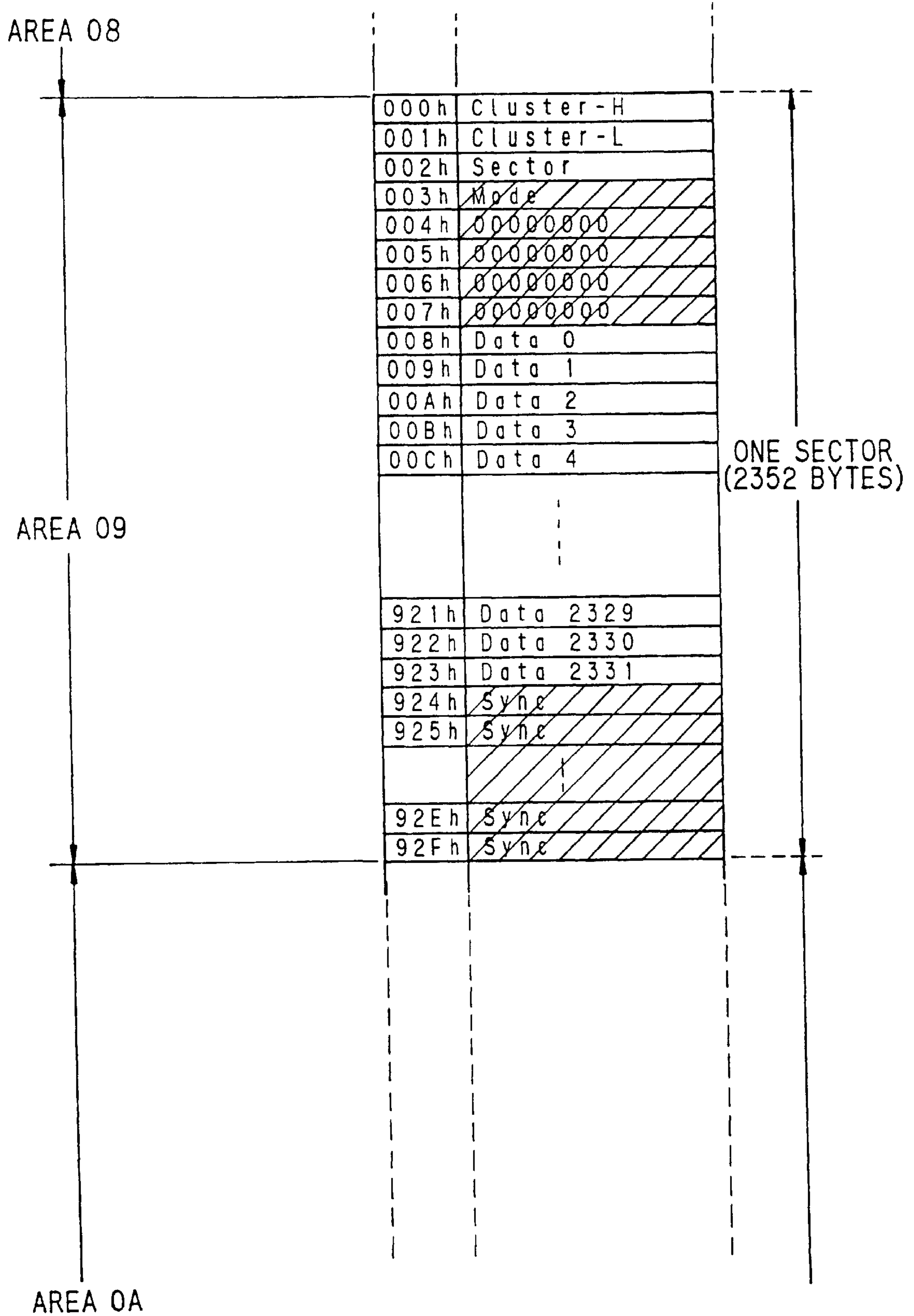
FIG. 2 PRIOR ART
