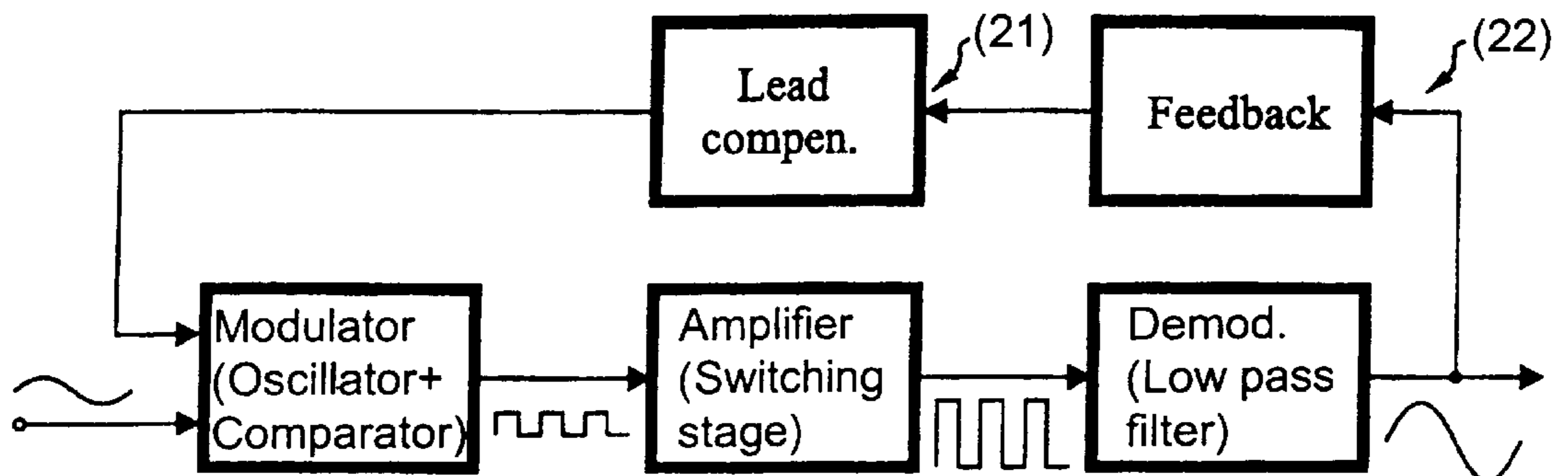
Fig. 2 (Prior art)
