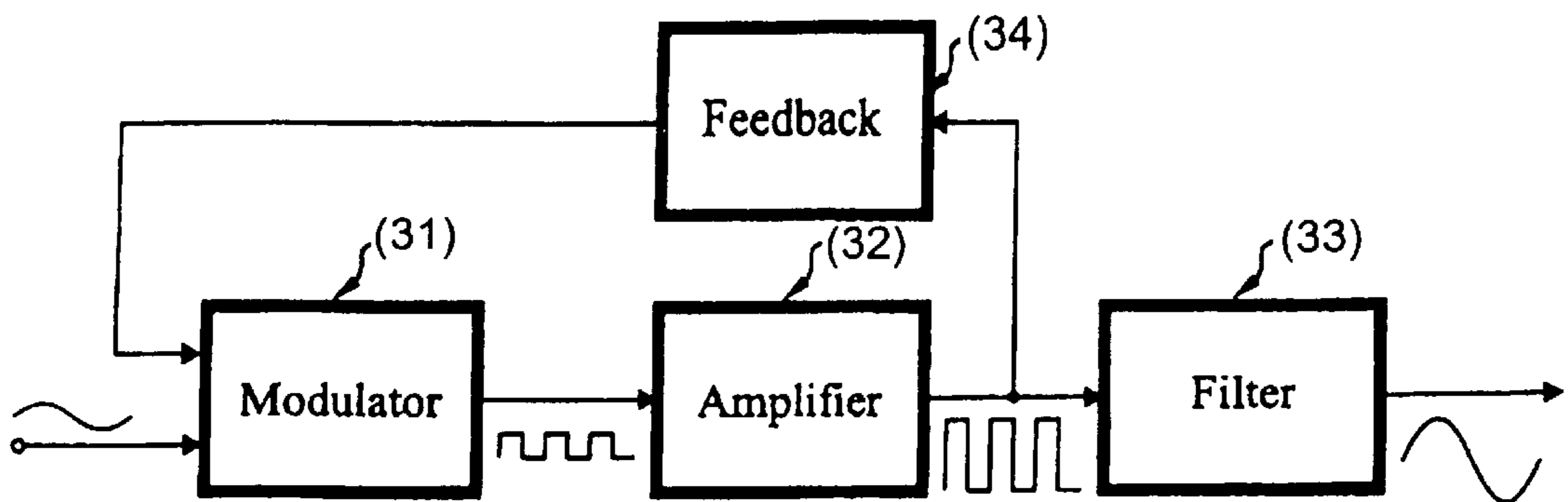
Fig. 3 (Prior art)
