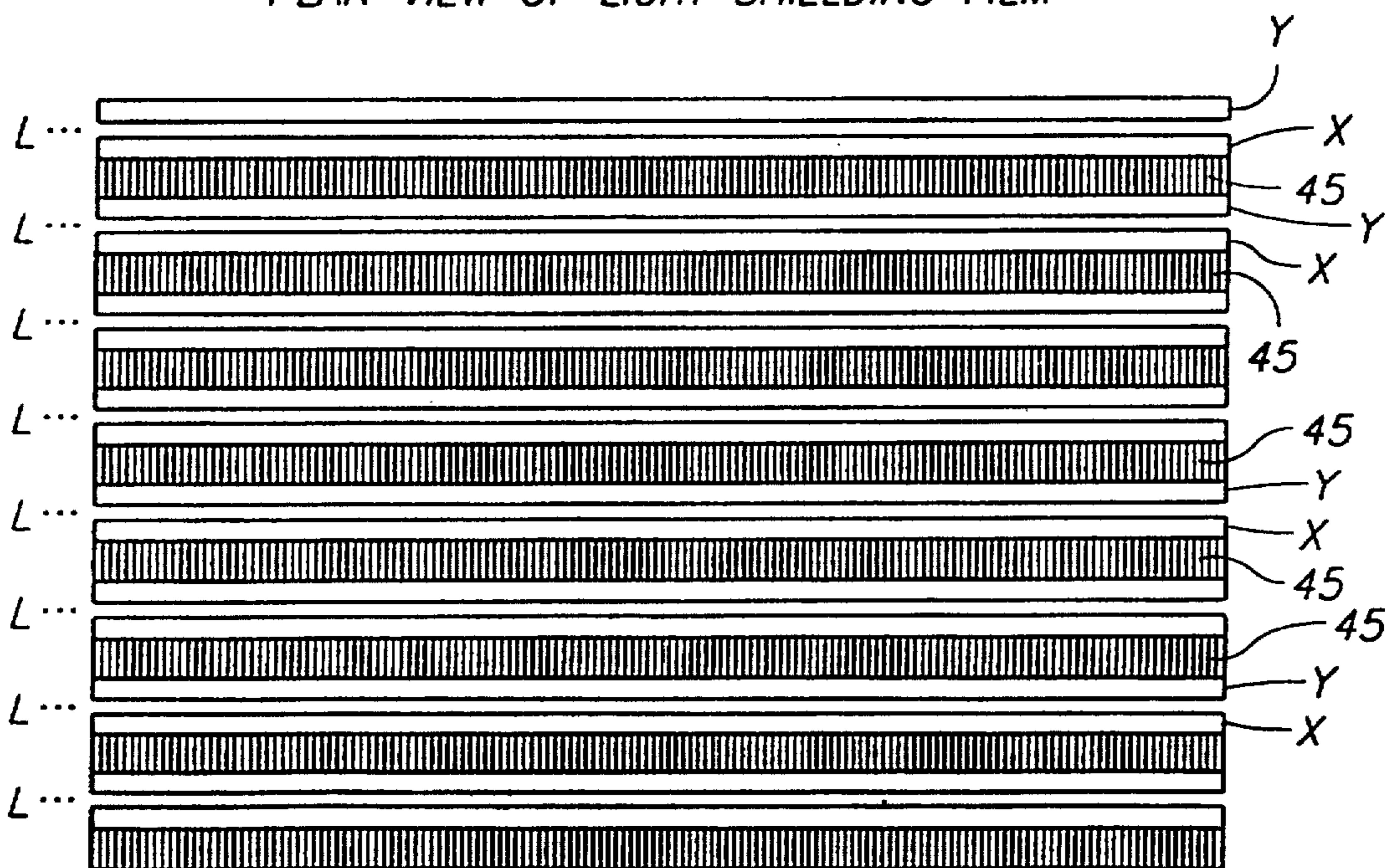
PLAN VIEW OF LIGHT SHIELDING FILM
