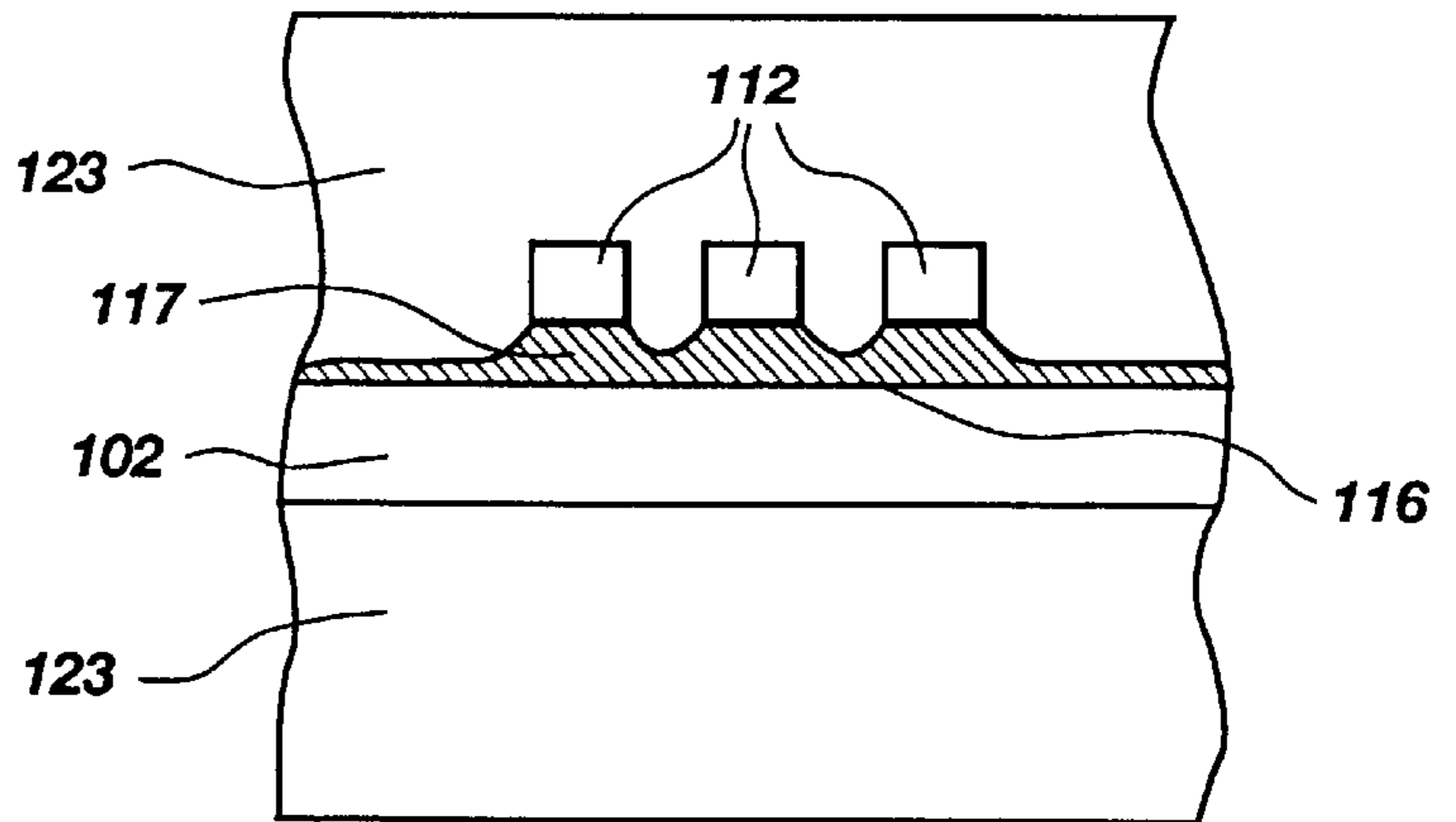
SECTION E-E
