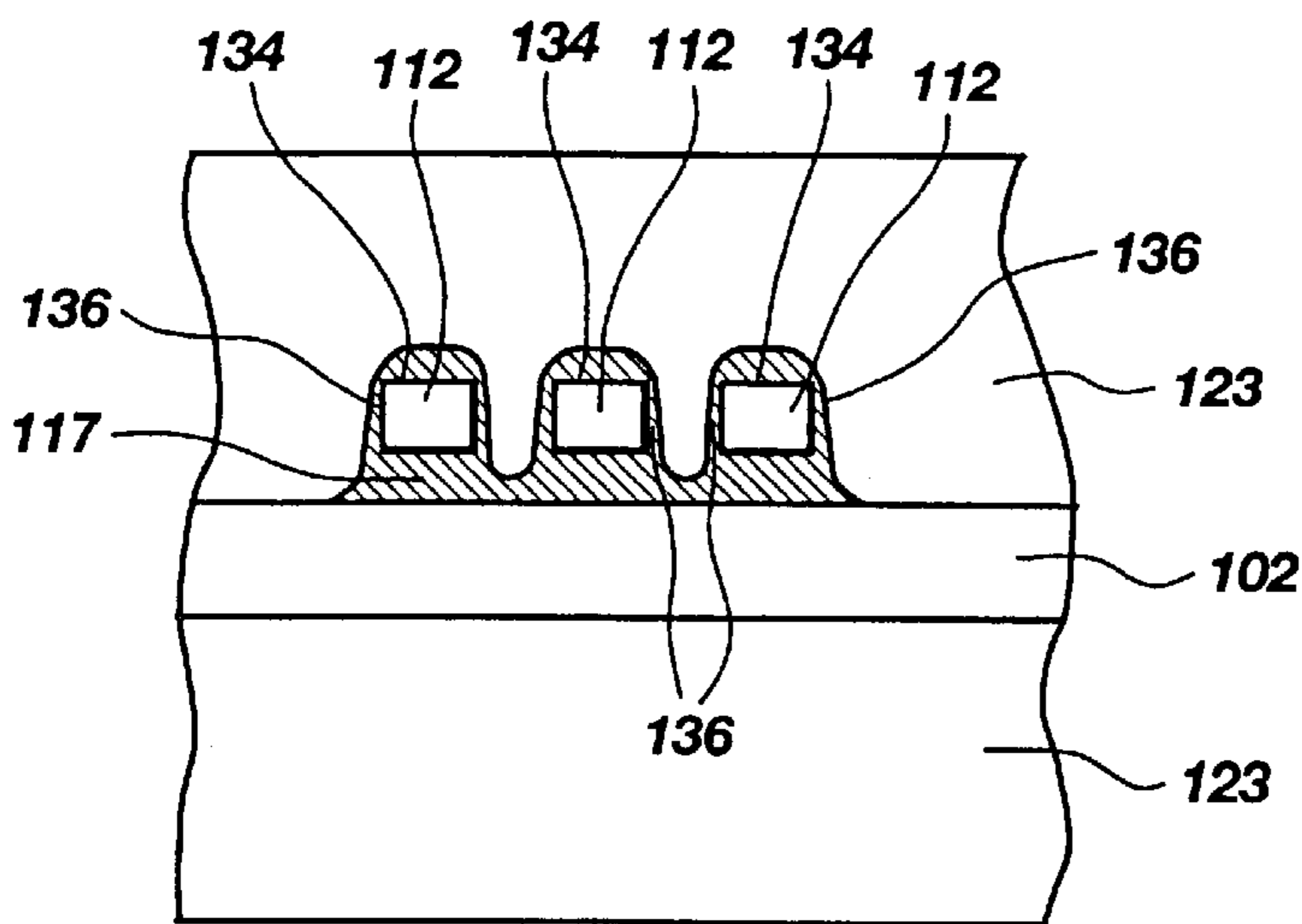
SECTION E-E
