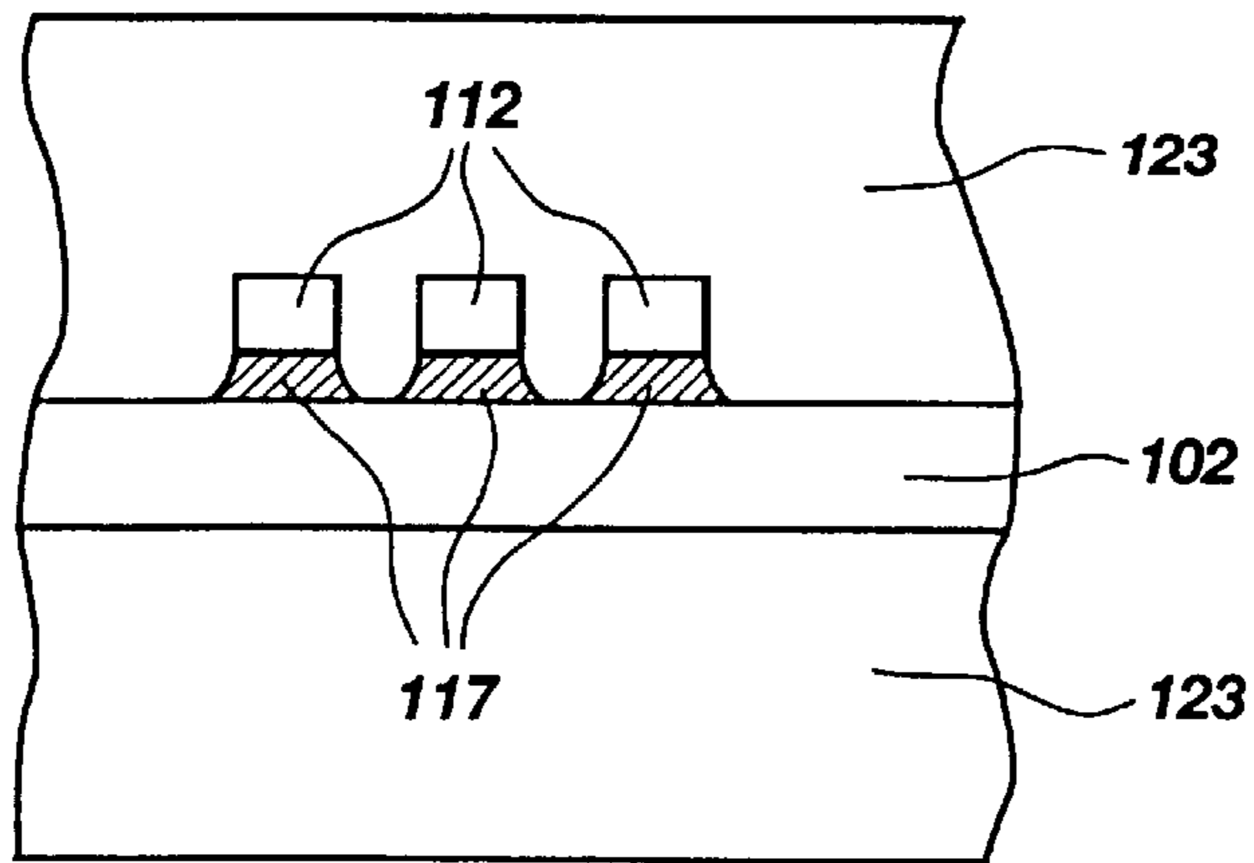
SECTION E-E
