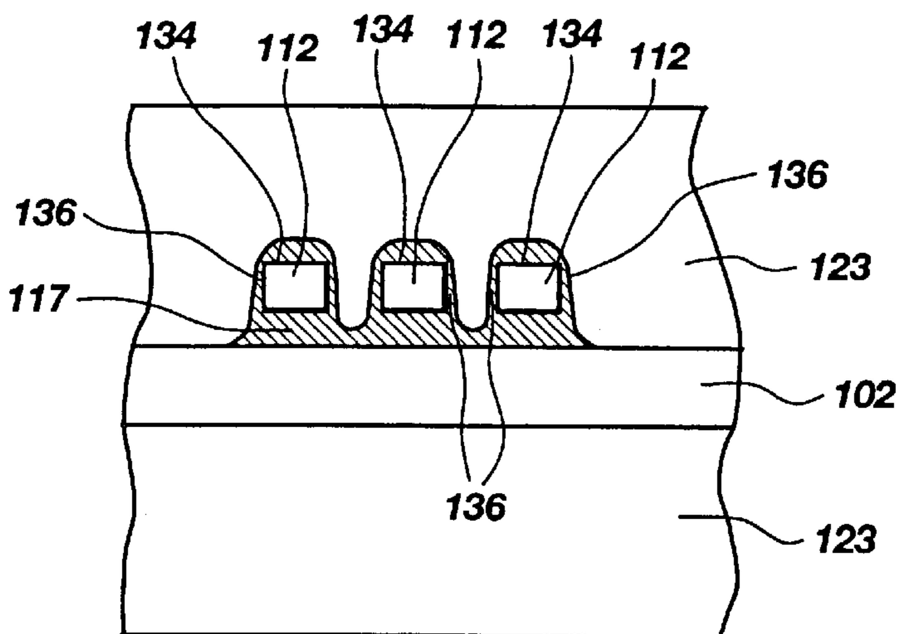
SECTION E-E
