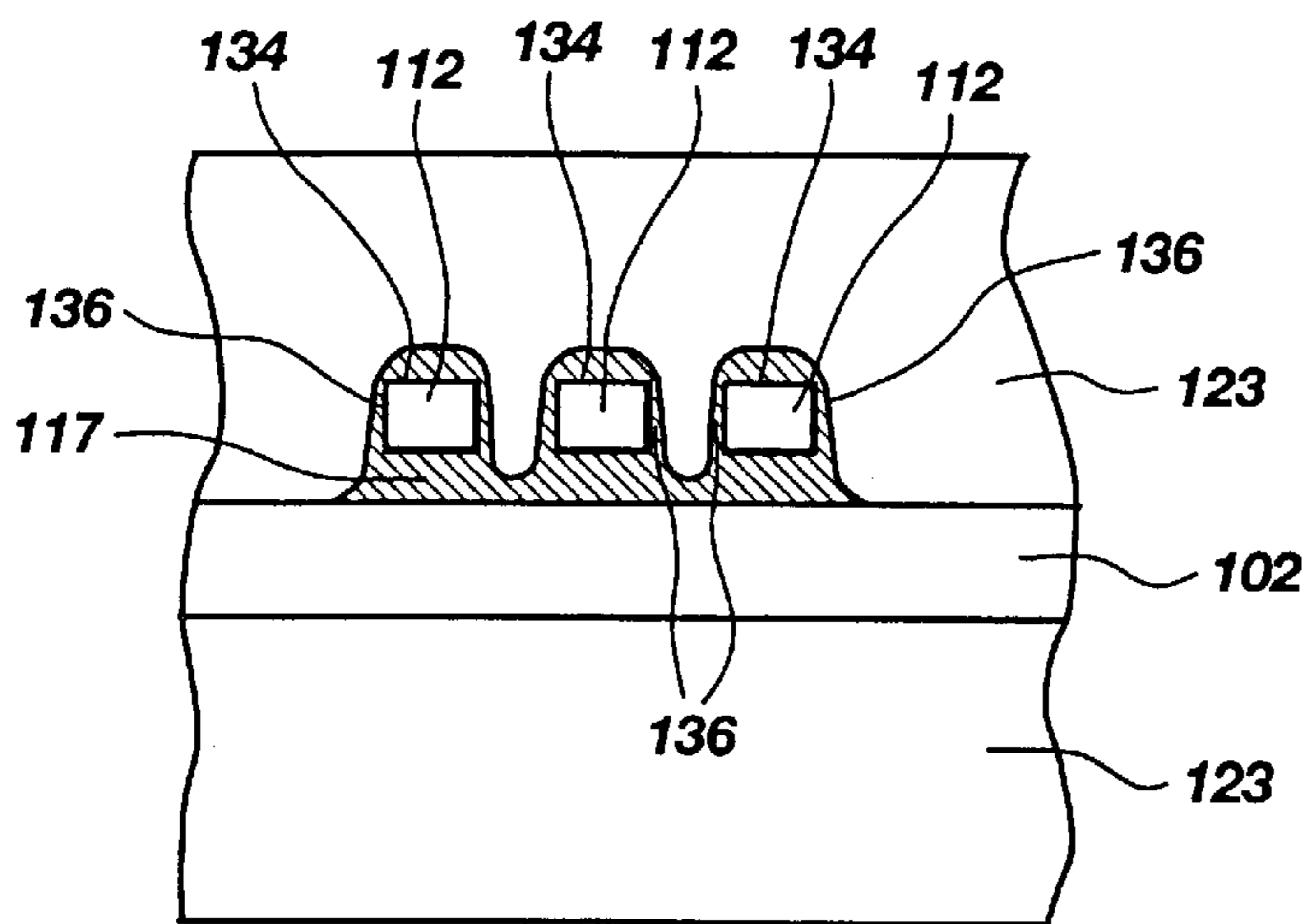
SECTION E-E
