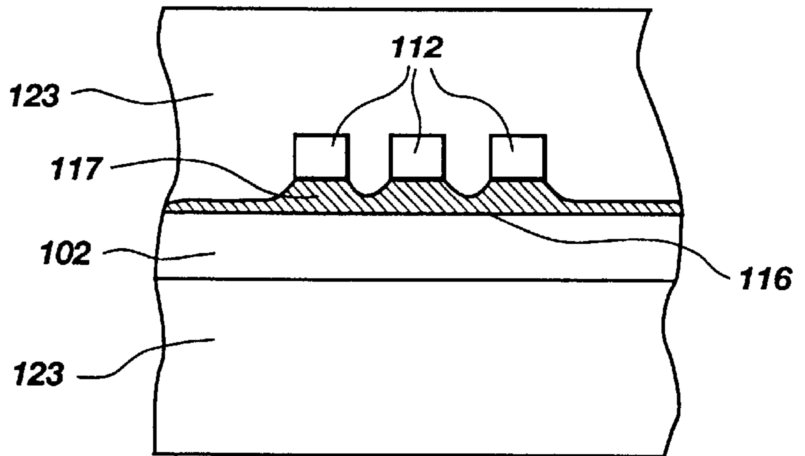
SECTION E-E
