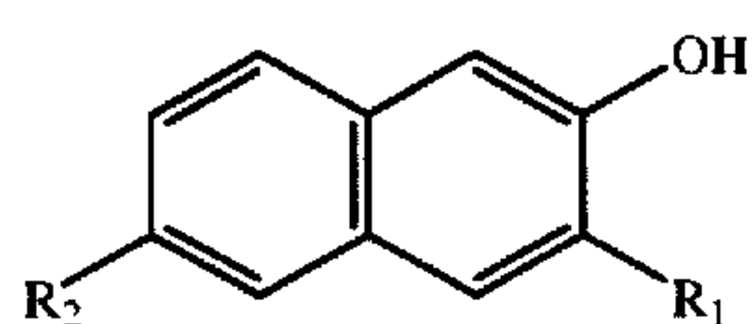
Coupler Compounds Based on Derivatives of 2-Naphthol (V).
