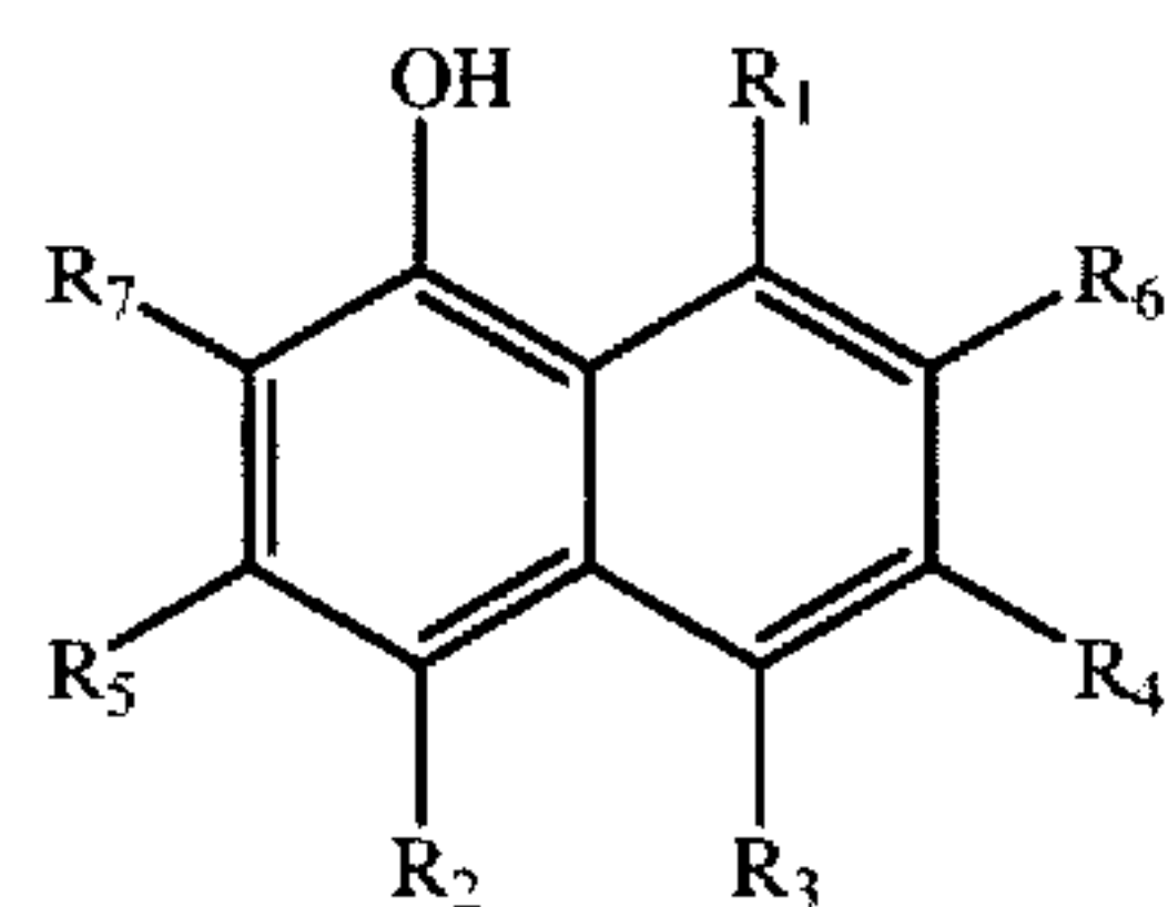
Coupler Compounds Based on 1-Naphthol and Derivatives (IV).
