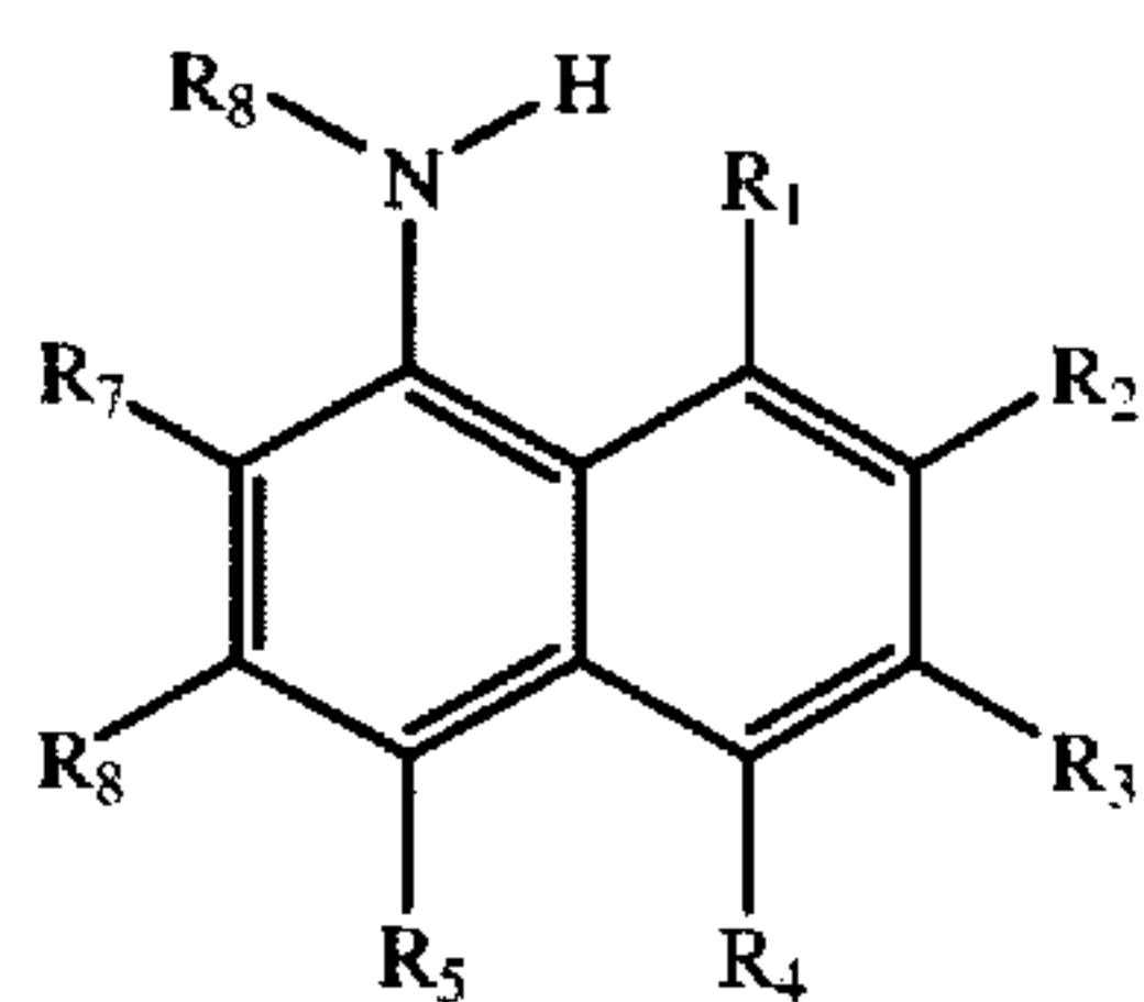
Coupler Compounds Based on Derivatives of 1-Aminonaphthalene (VI).
