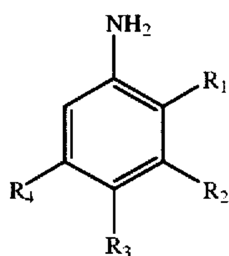
Precursor Compounds Based on Aromatic Amine and Derivatives (I).
