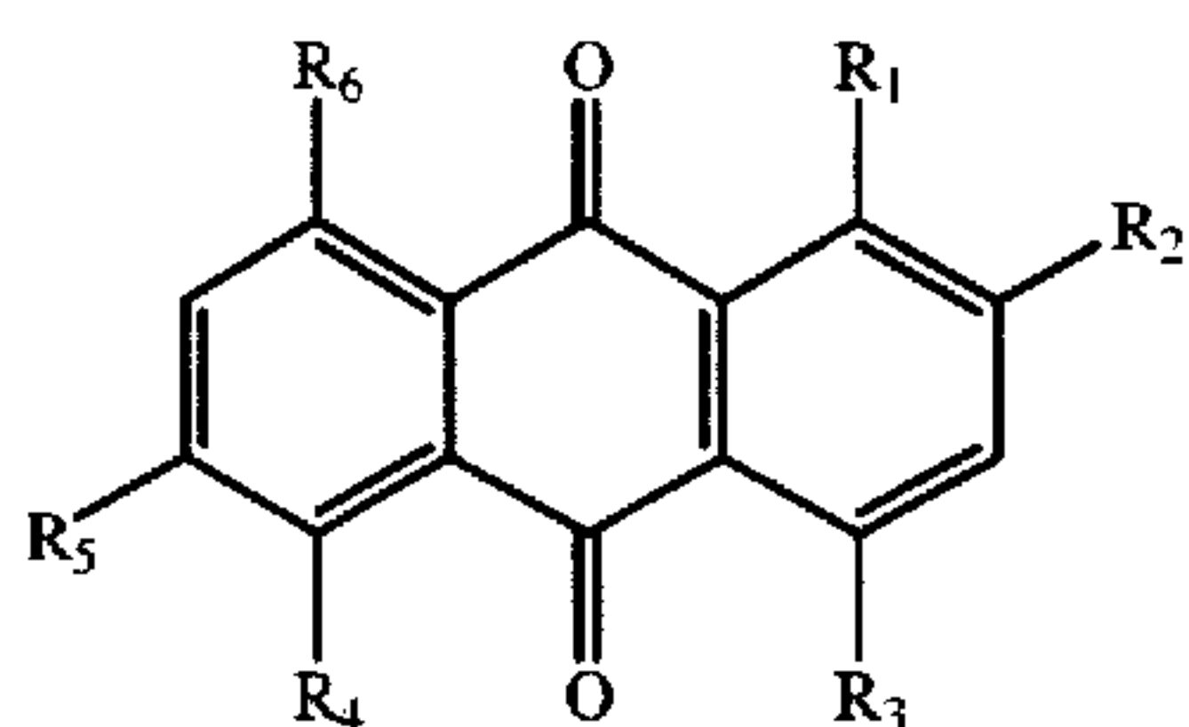
Coupler Compounds Based on Derivatives of Anthraquinone (VII).
