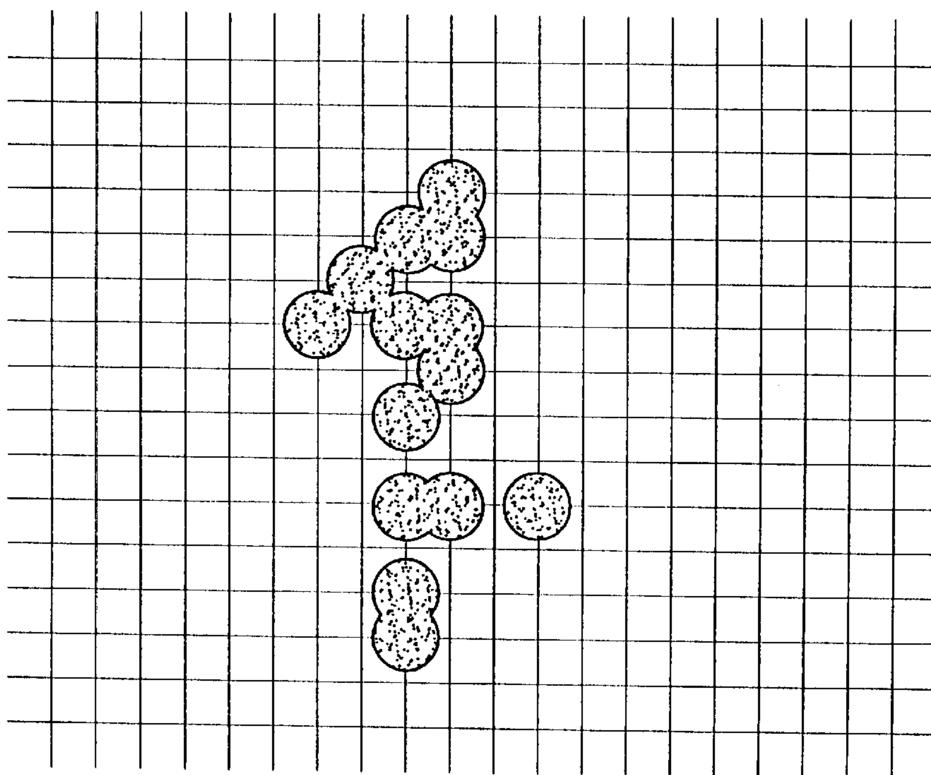
DEPLETED BITMAP
