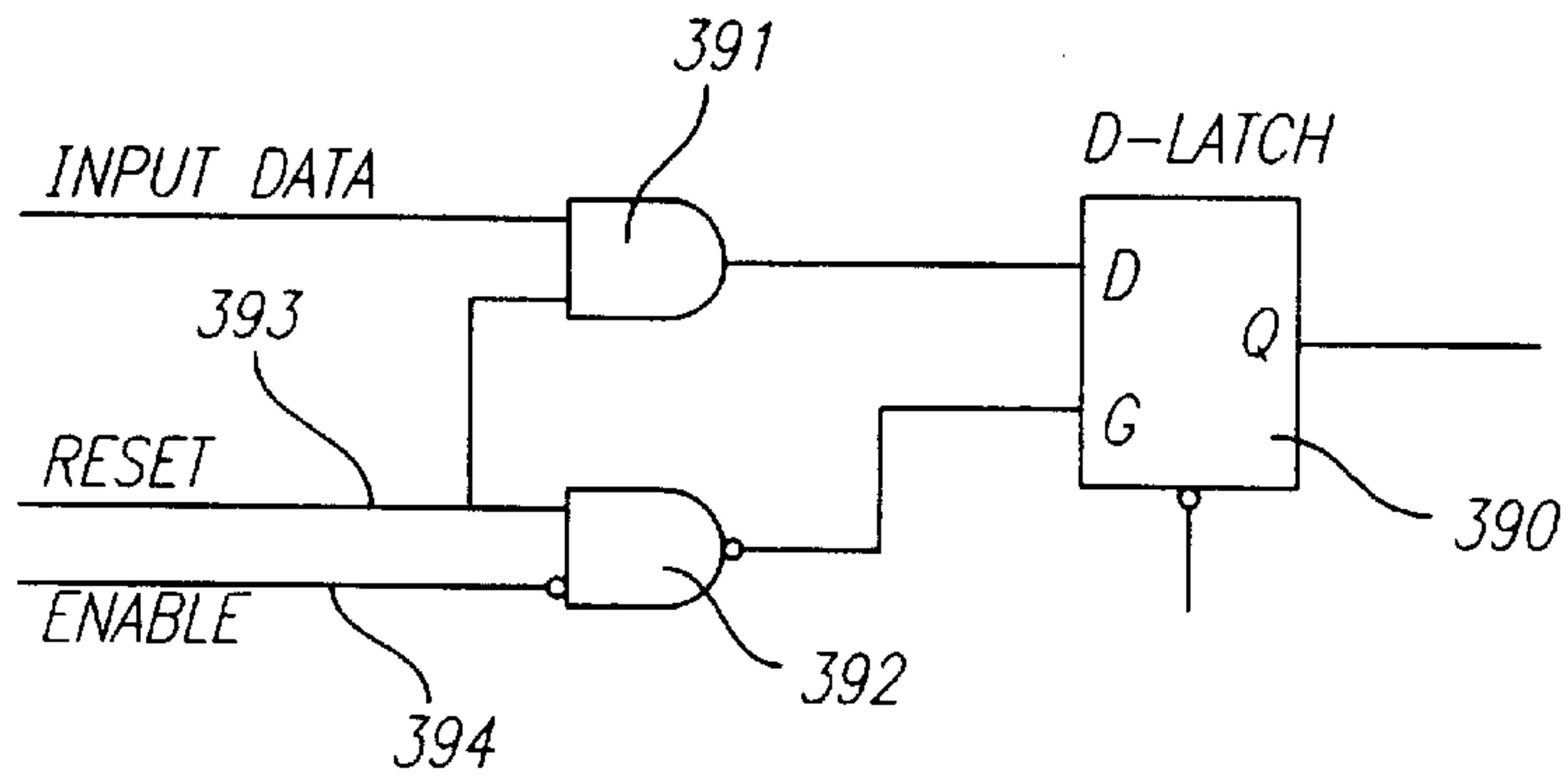
FIG. 37 FAILING IMPLEMENTATION OF A LATCH WITH CLEAR
