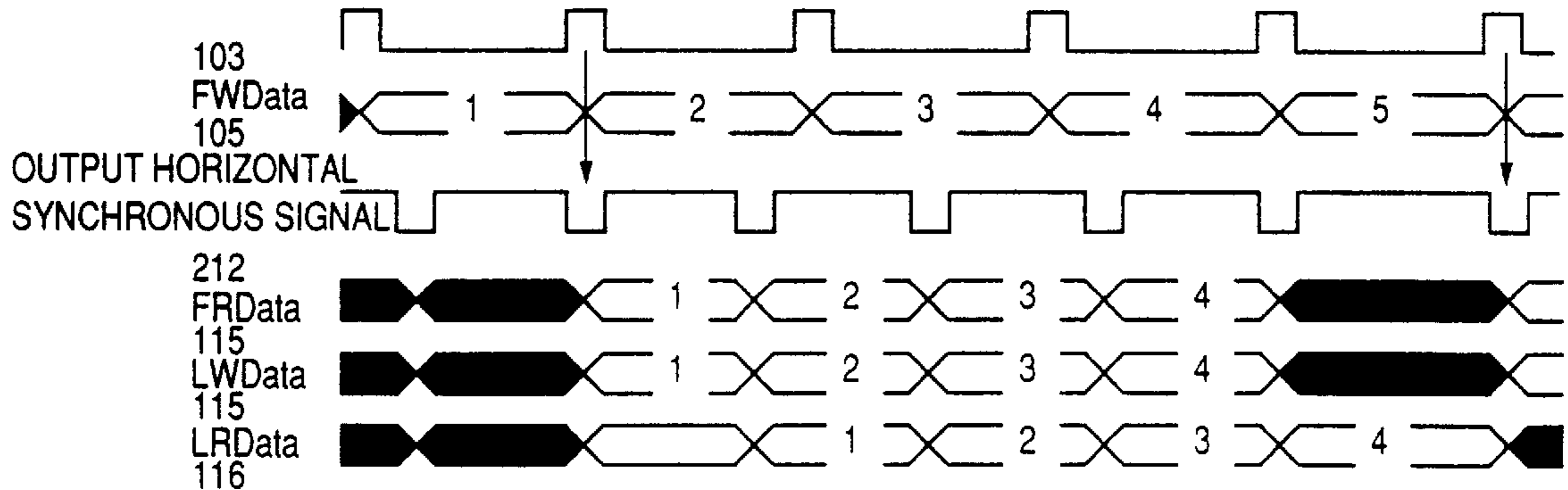
TIMING CHART FOR VERTICAL DIRECTION MEMORY ACCESS OF GRADATION INTEGRATION METHOD(4→5)
