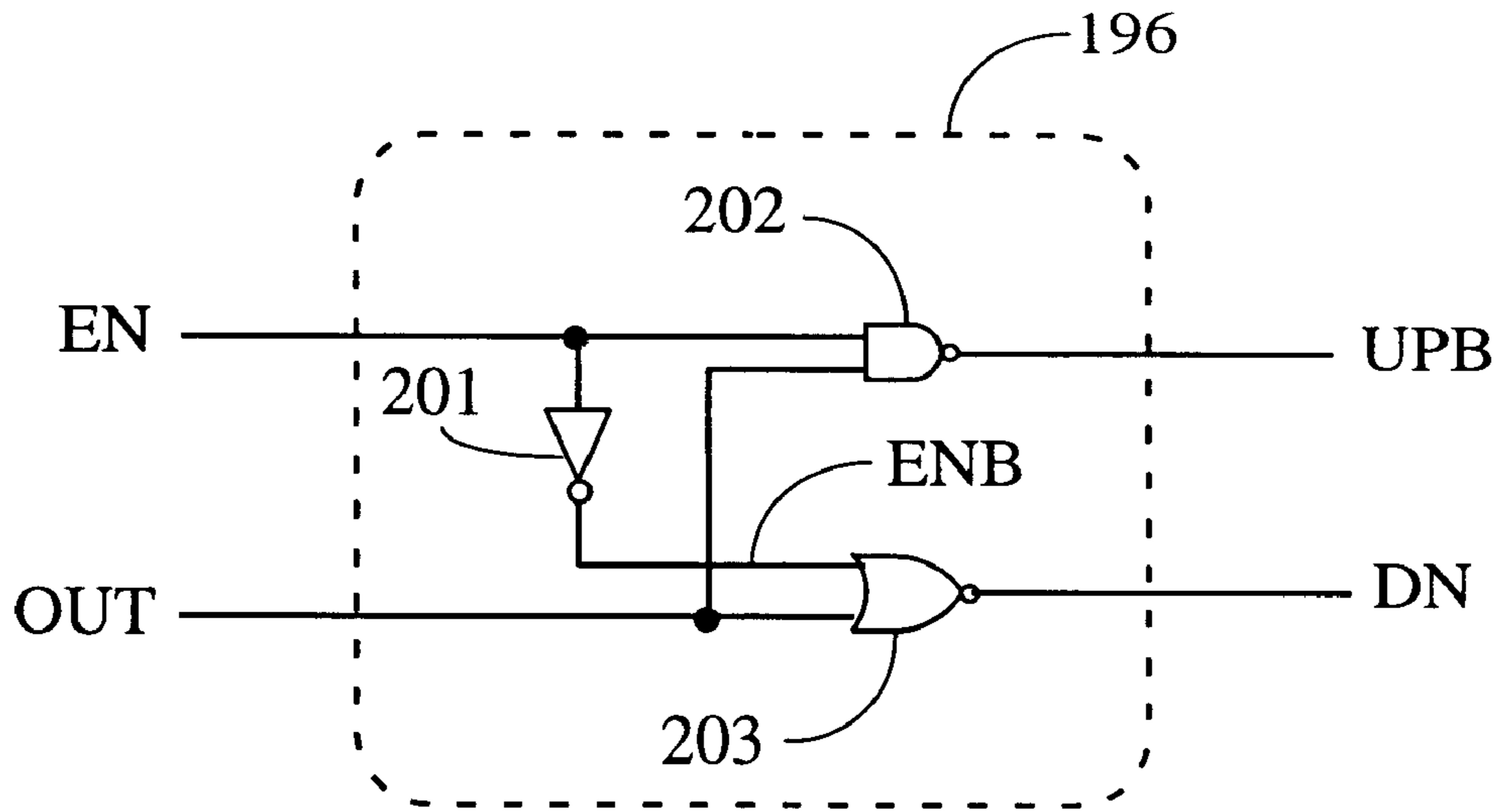
FIG. 2 (Prior Art)
