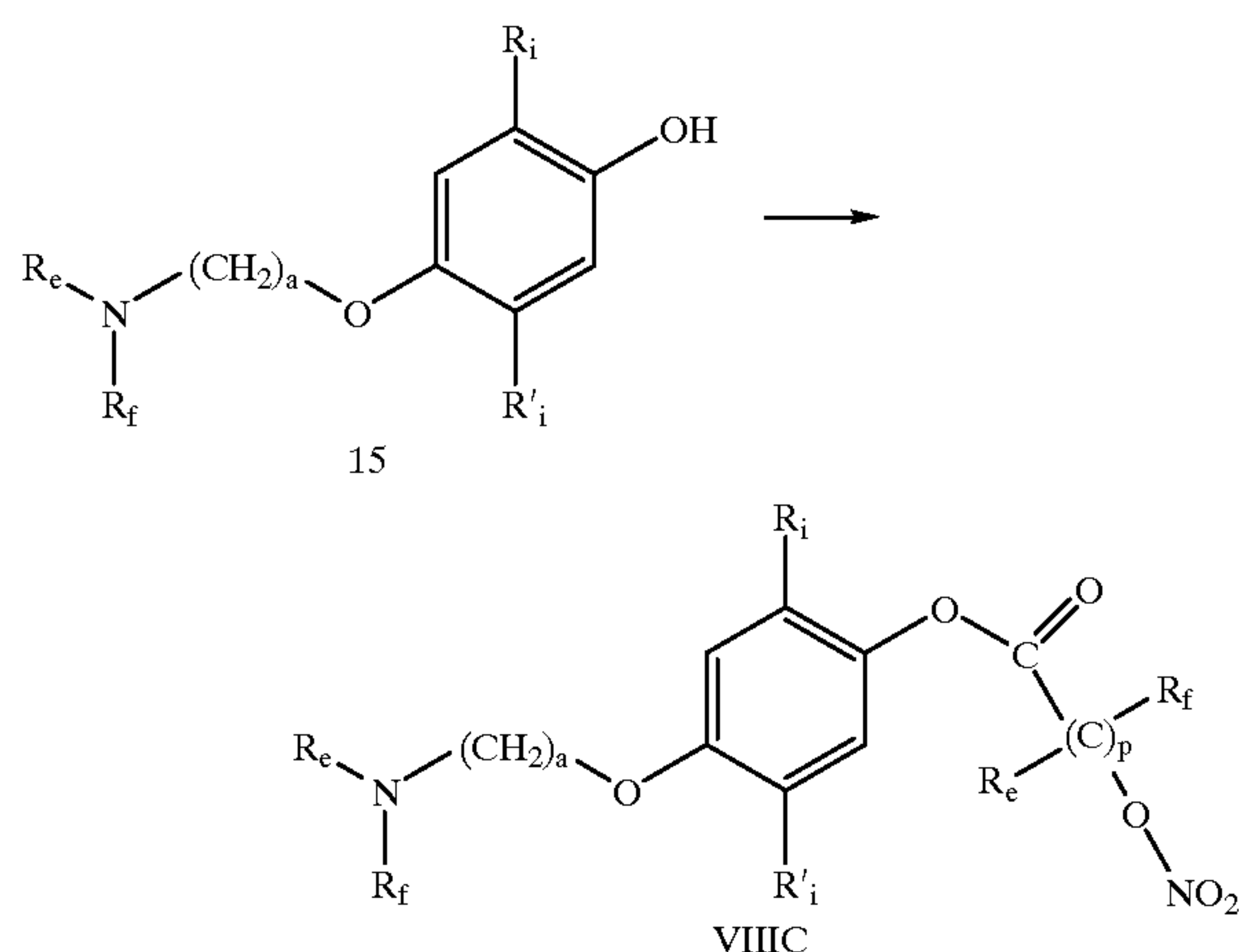
Scheme XXI
