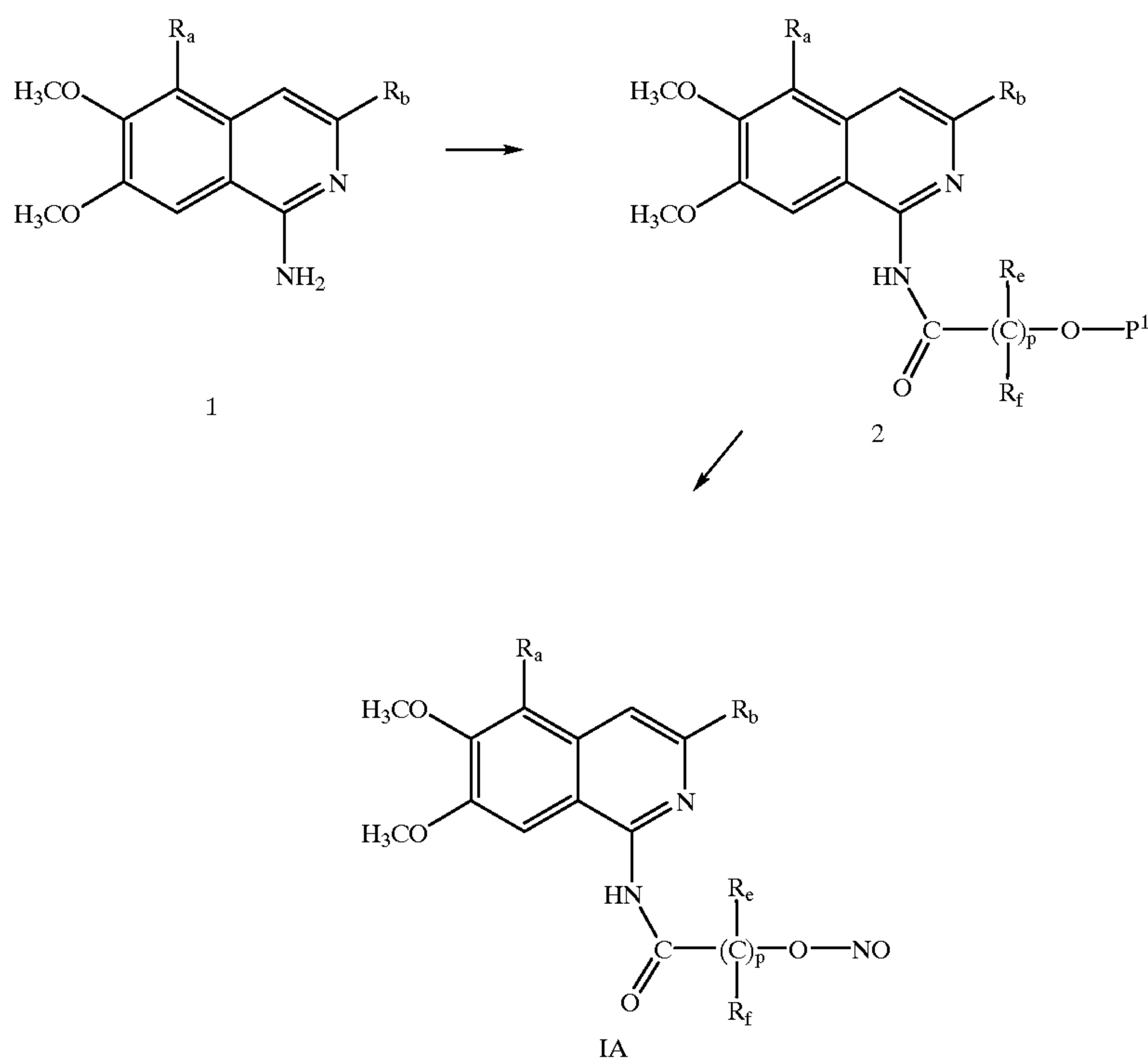
Scheme I
