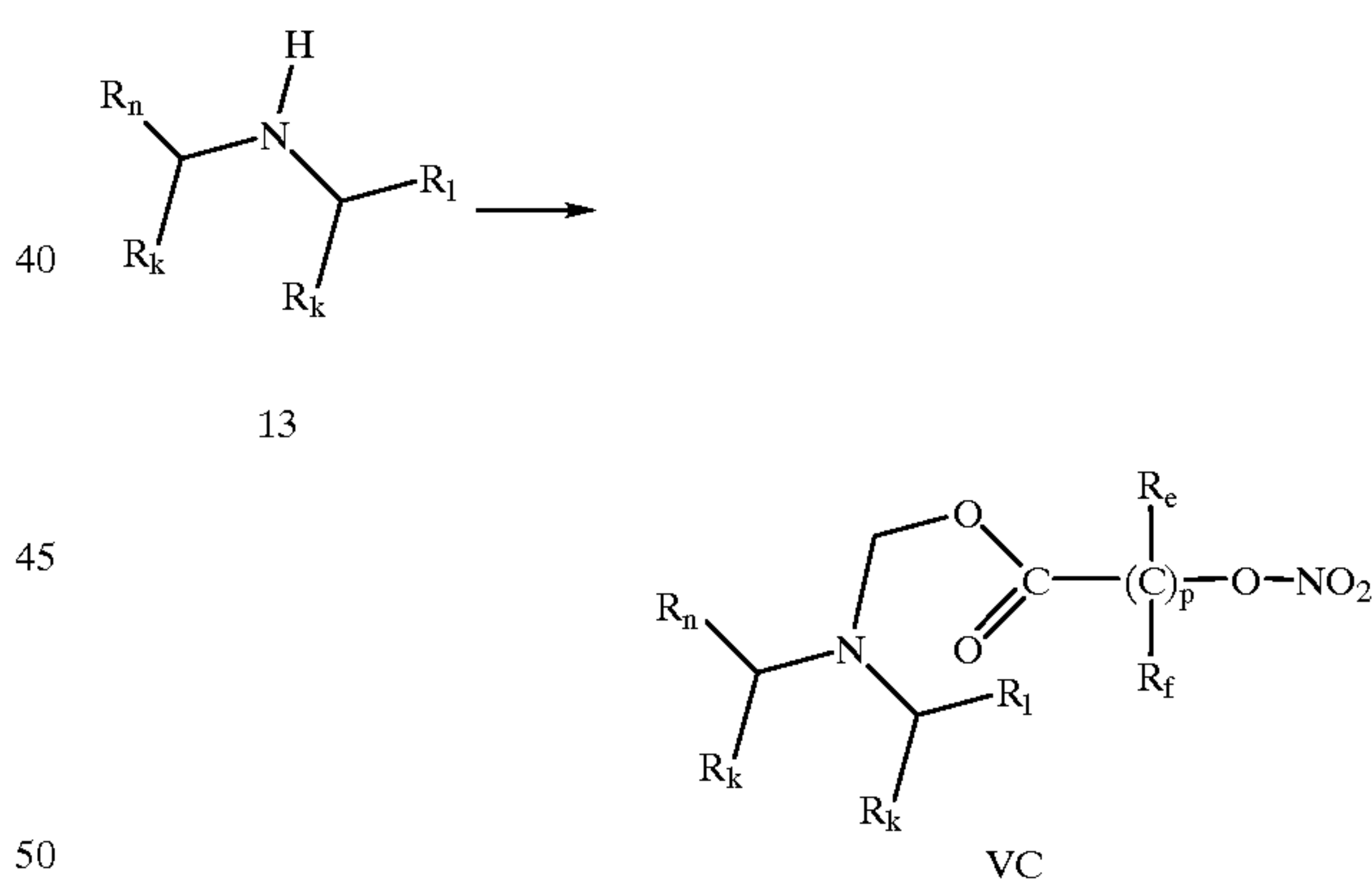
Scheme XV
