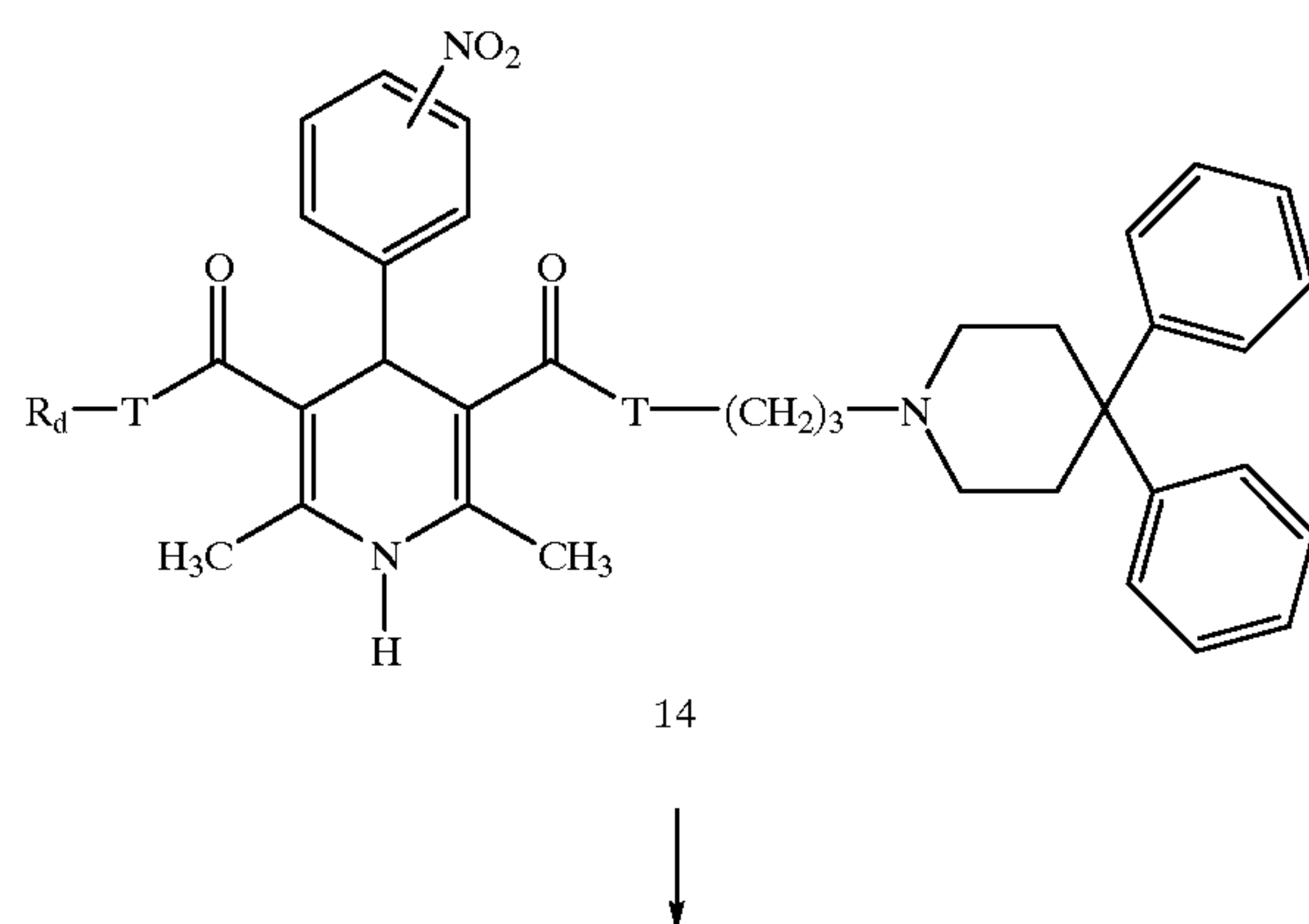
Scheme XVIII
