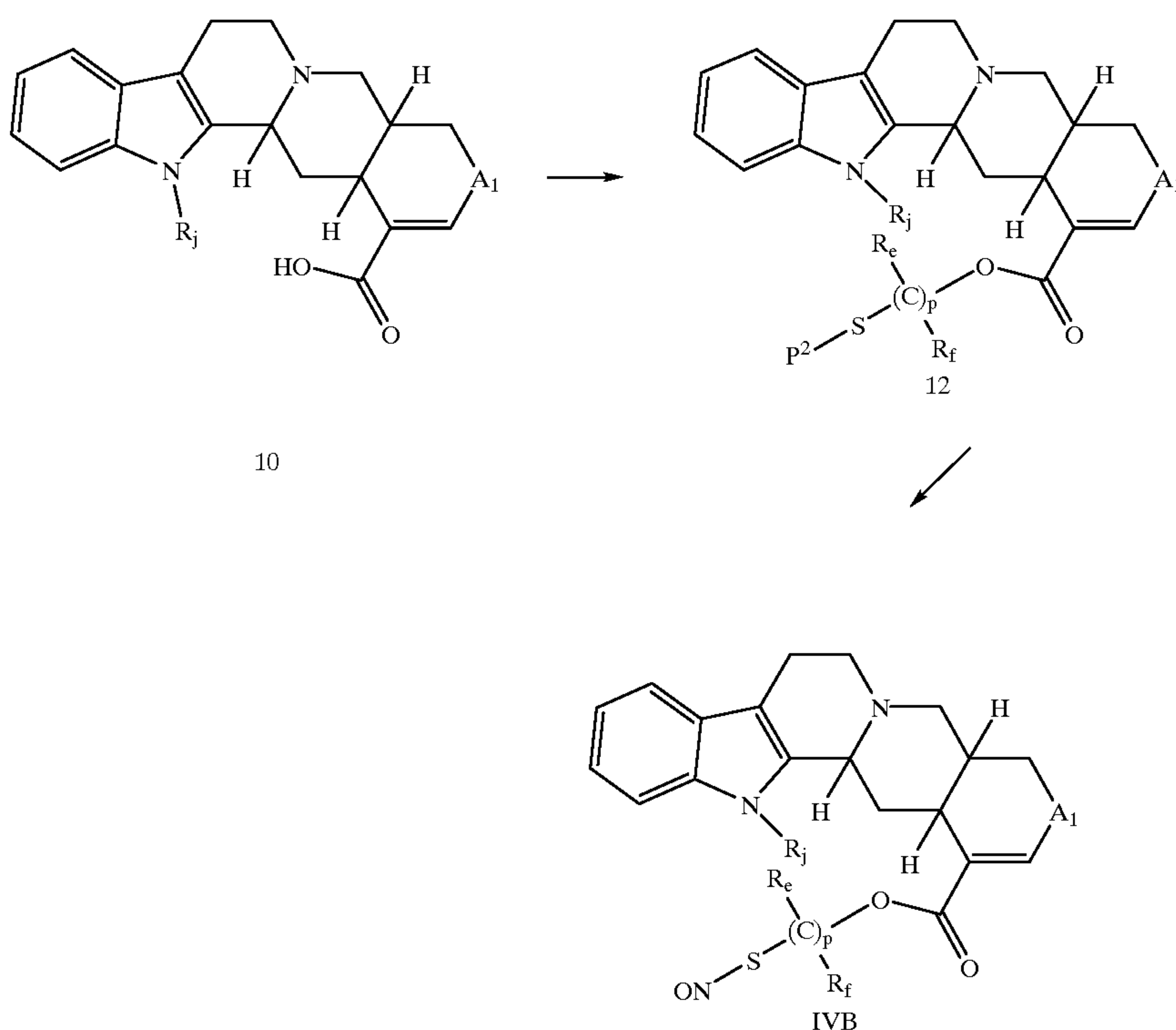
Scheme XI
