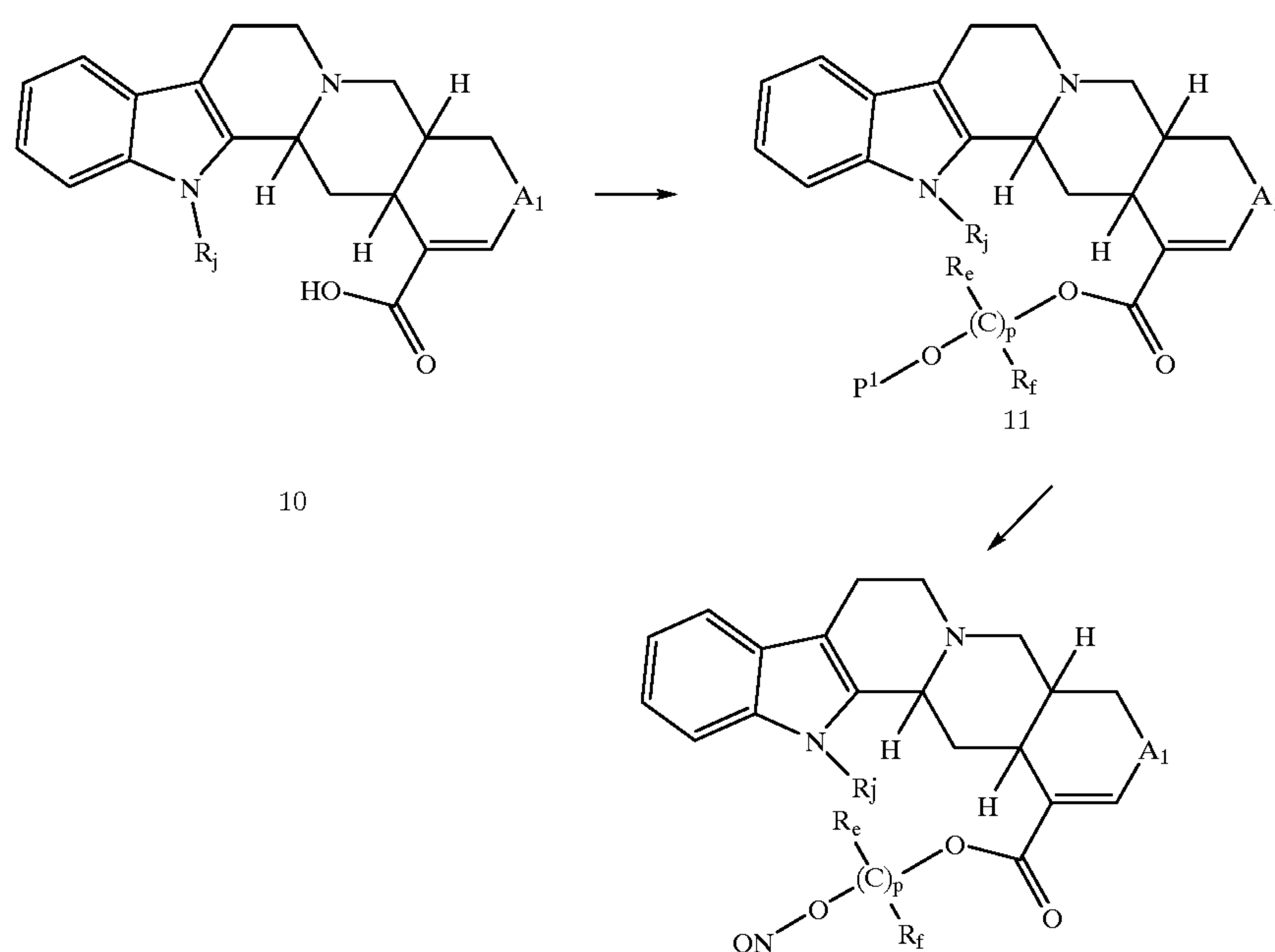
Scheme X
