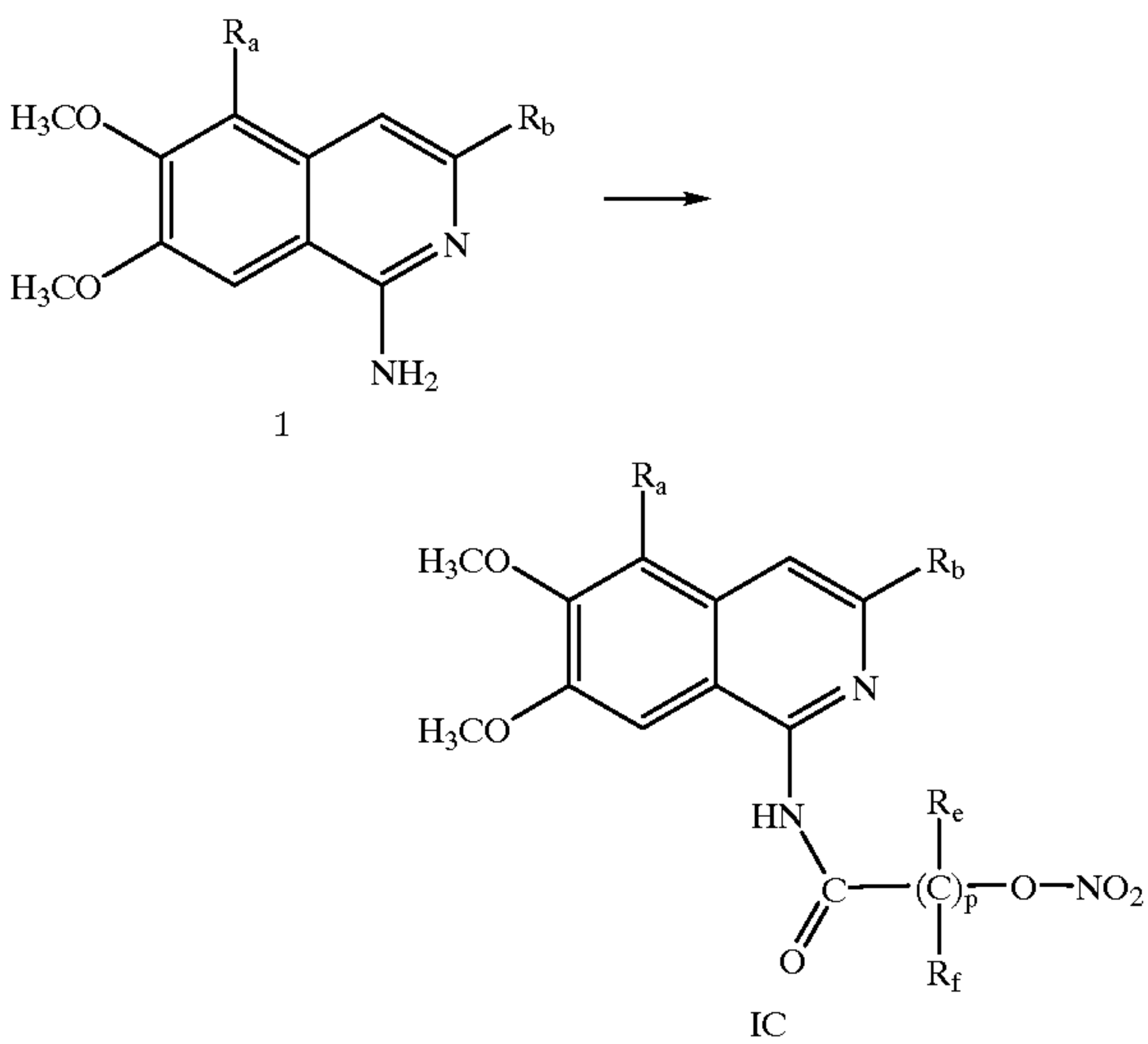
Scheme III
