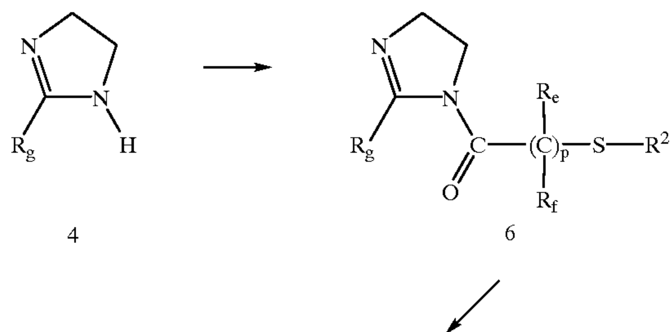
Scheme V
