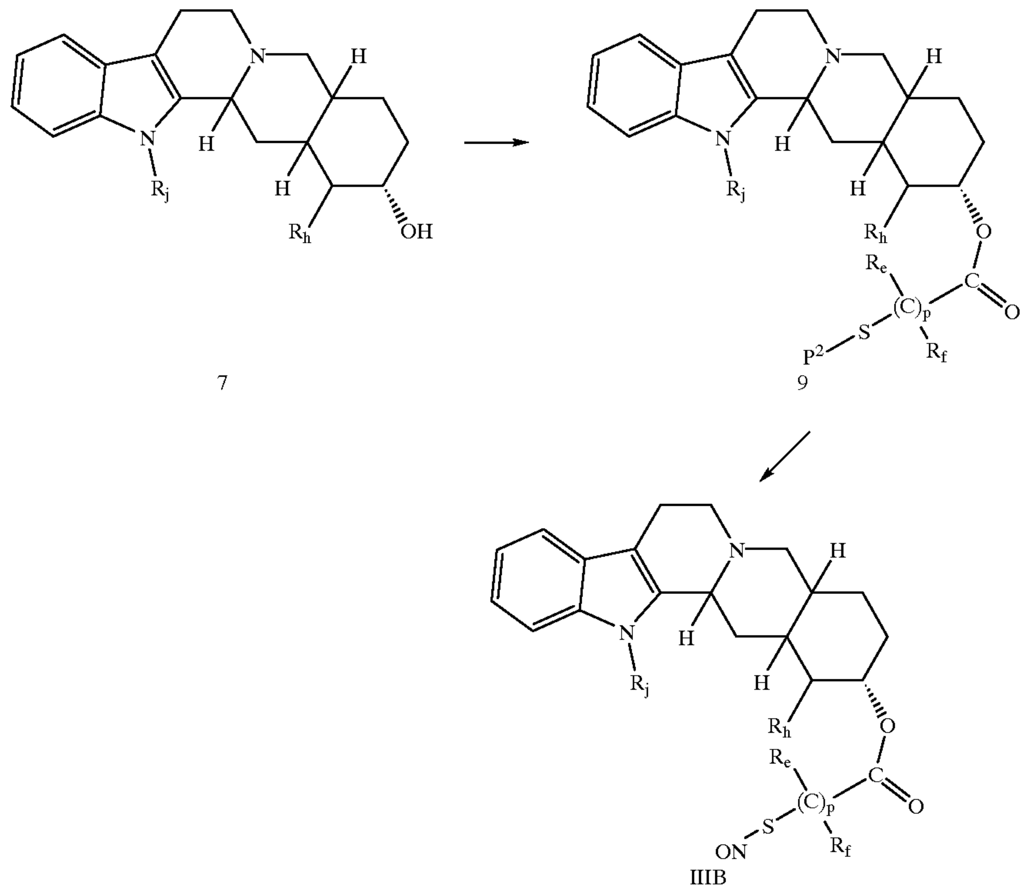
Scheme VIII
