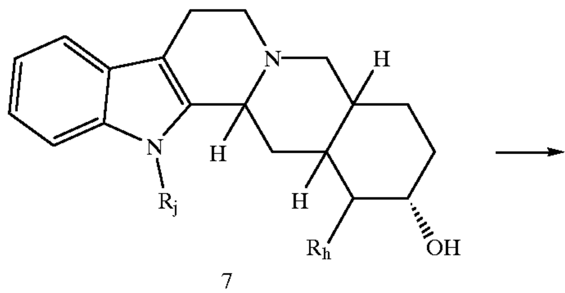
Scheme IX
