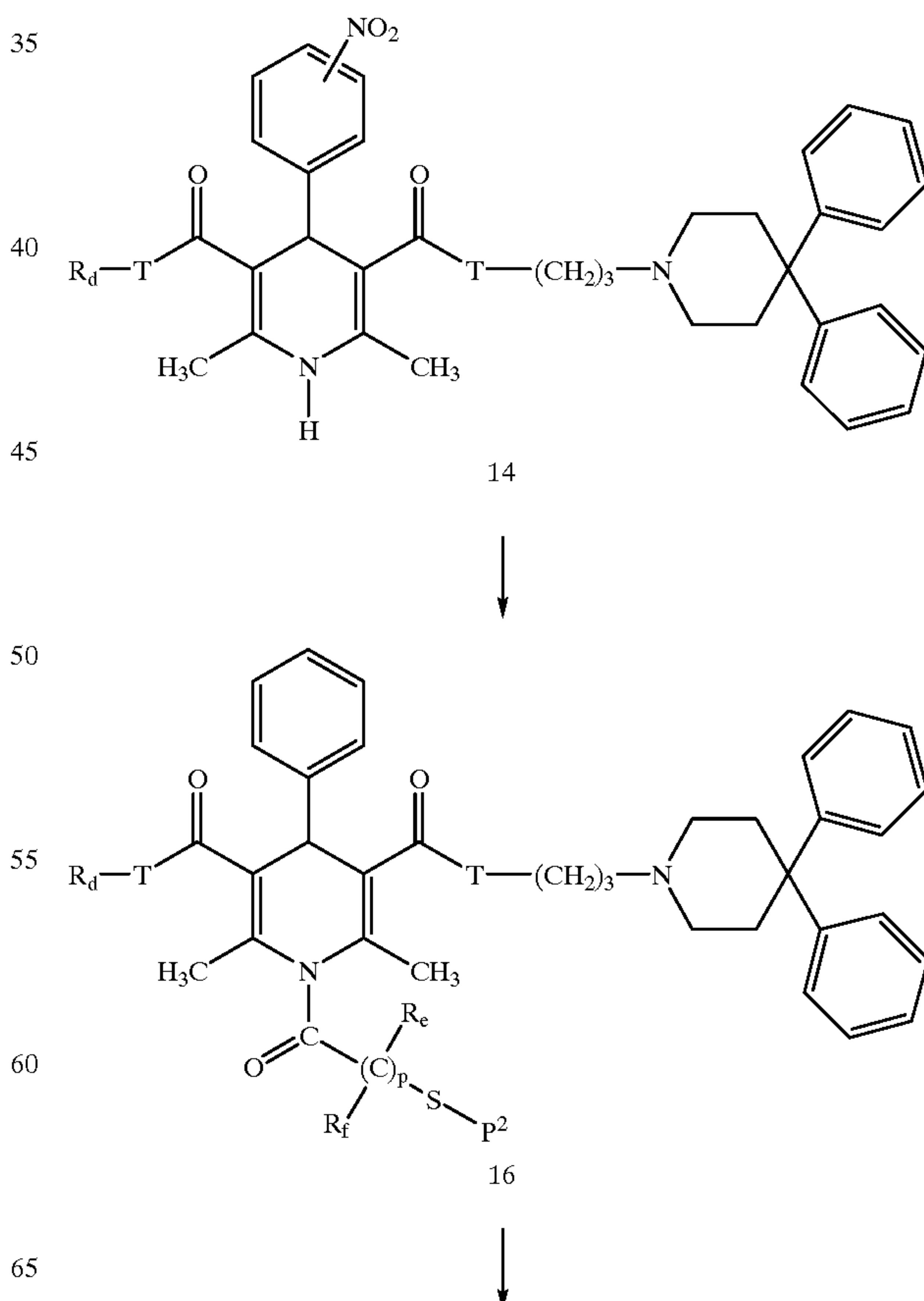
Scheme XVII
