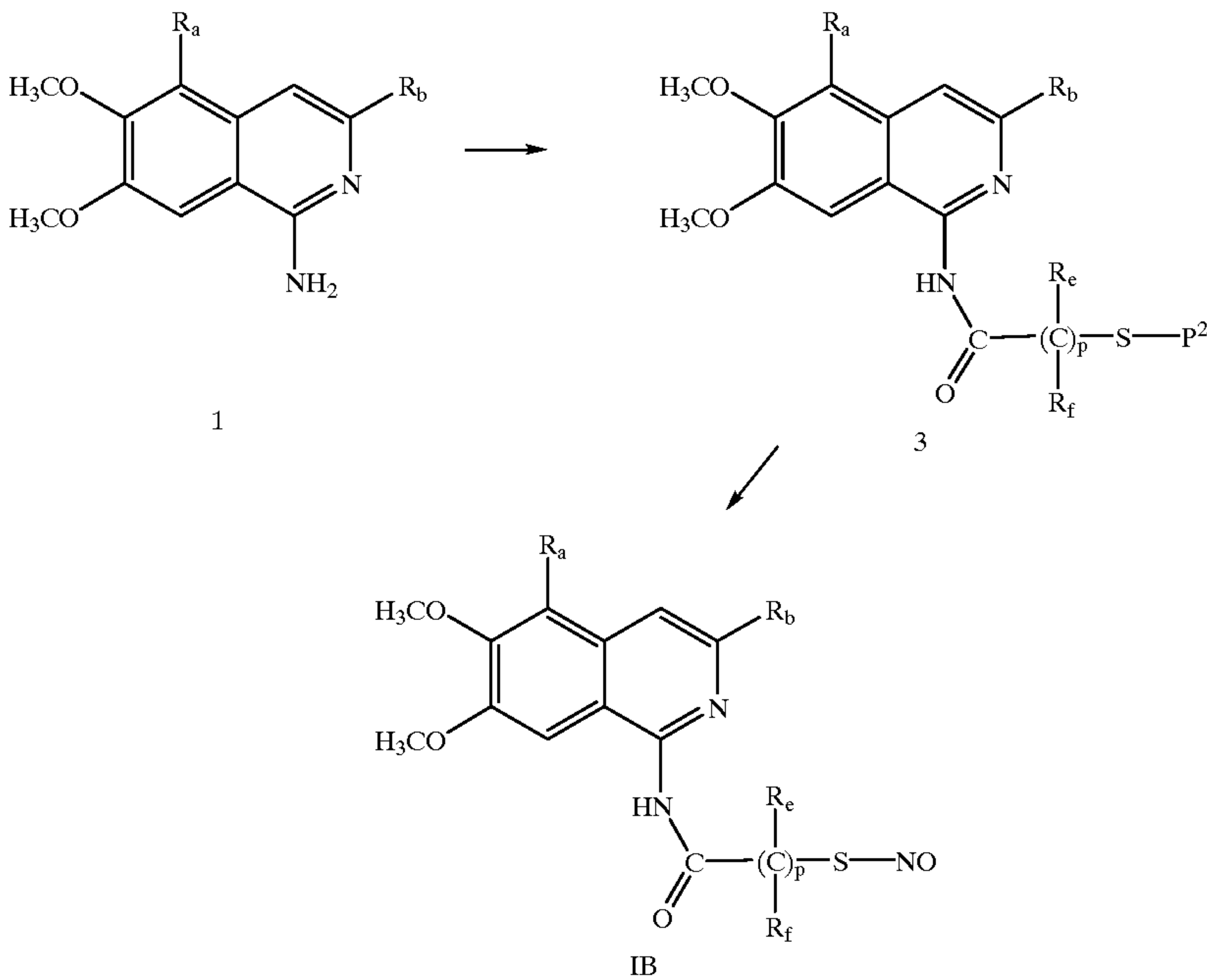
Scheme II
