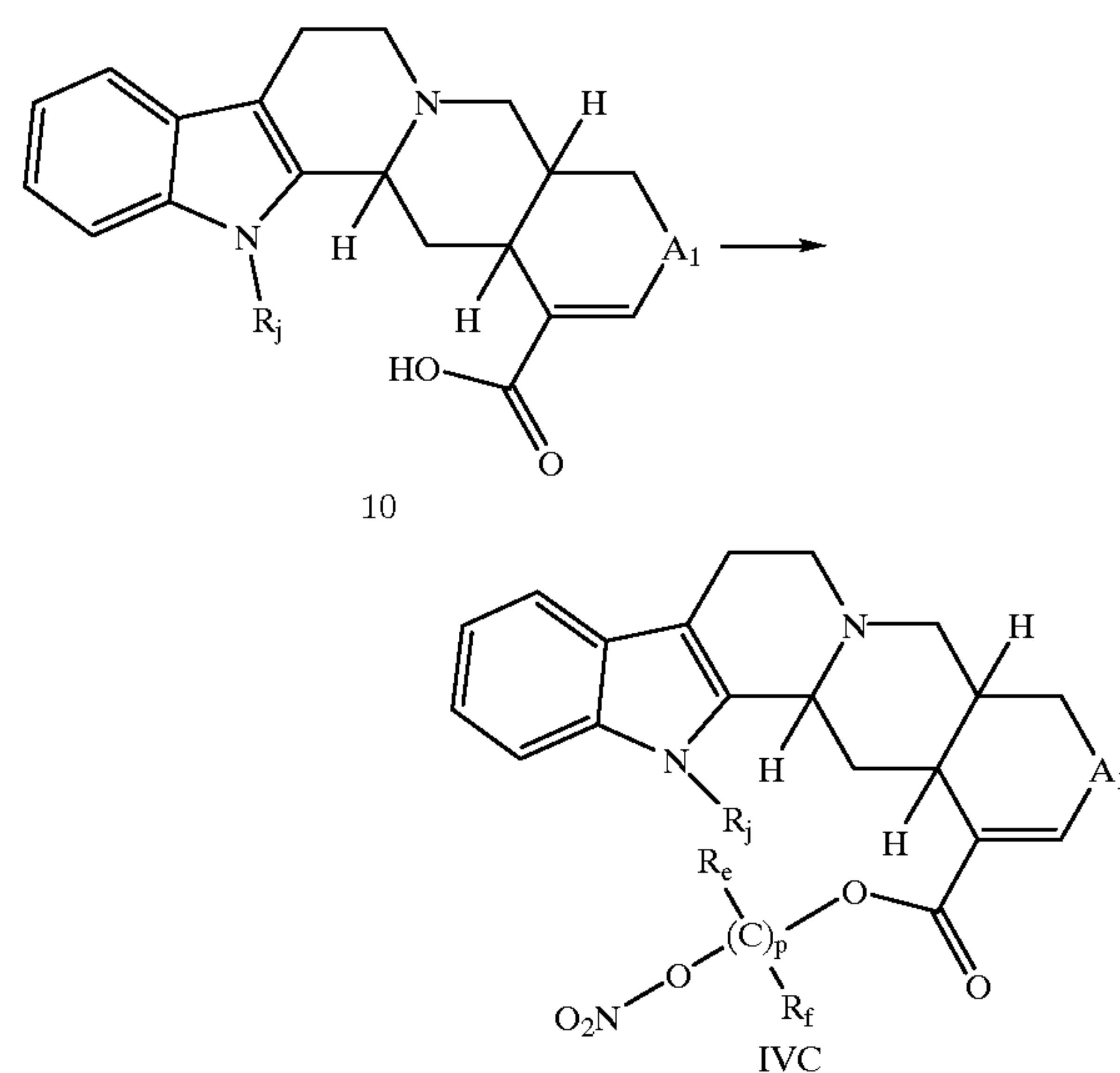
Scheme XII
