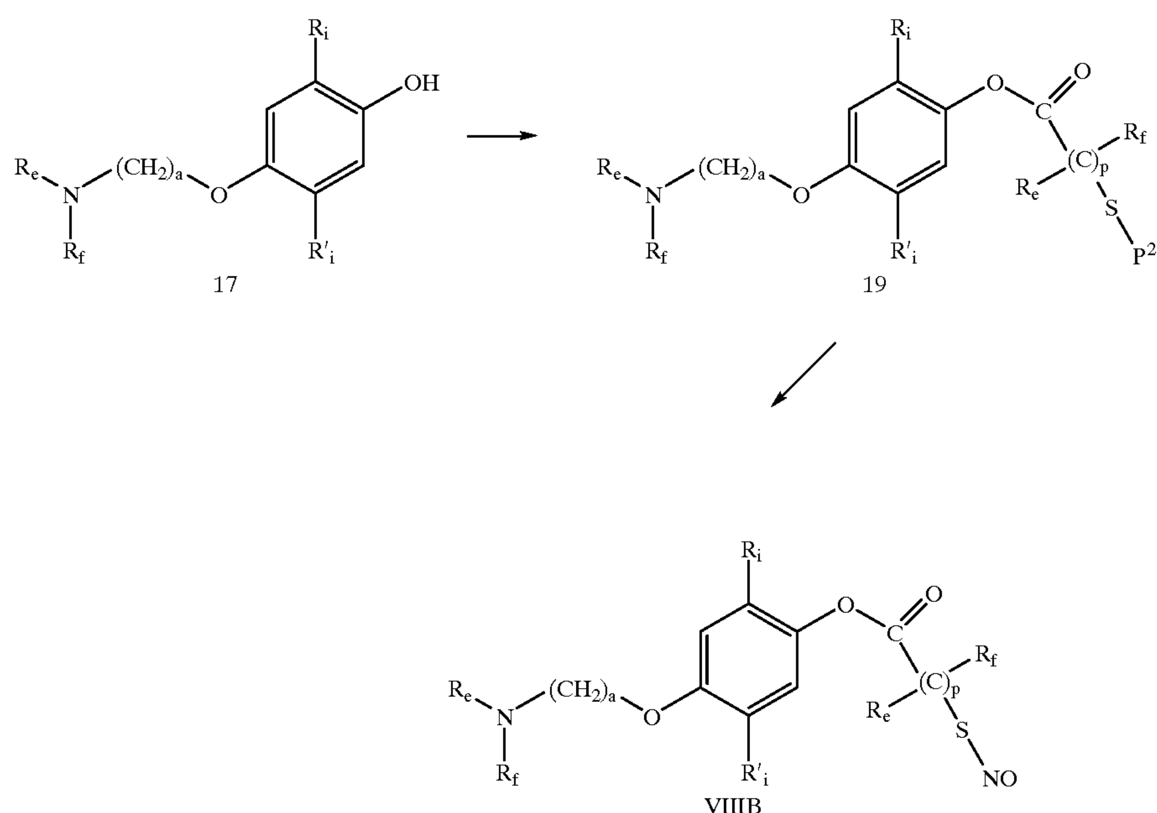
Scheme XX
