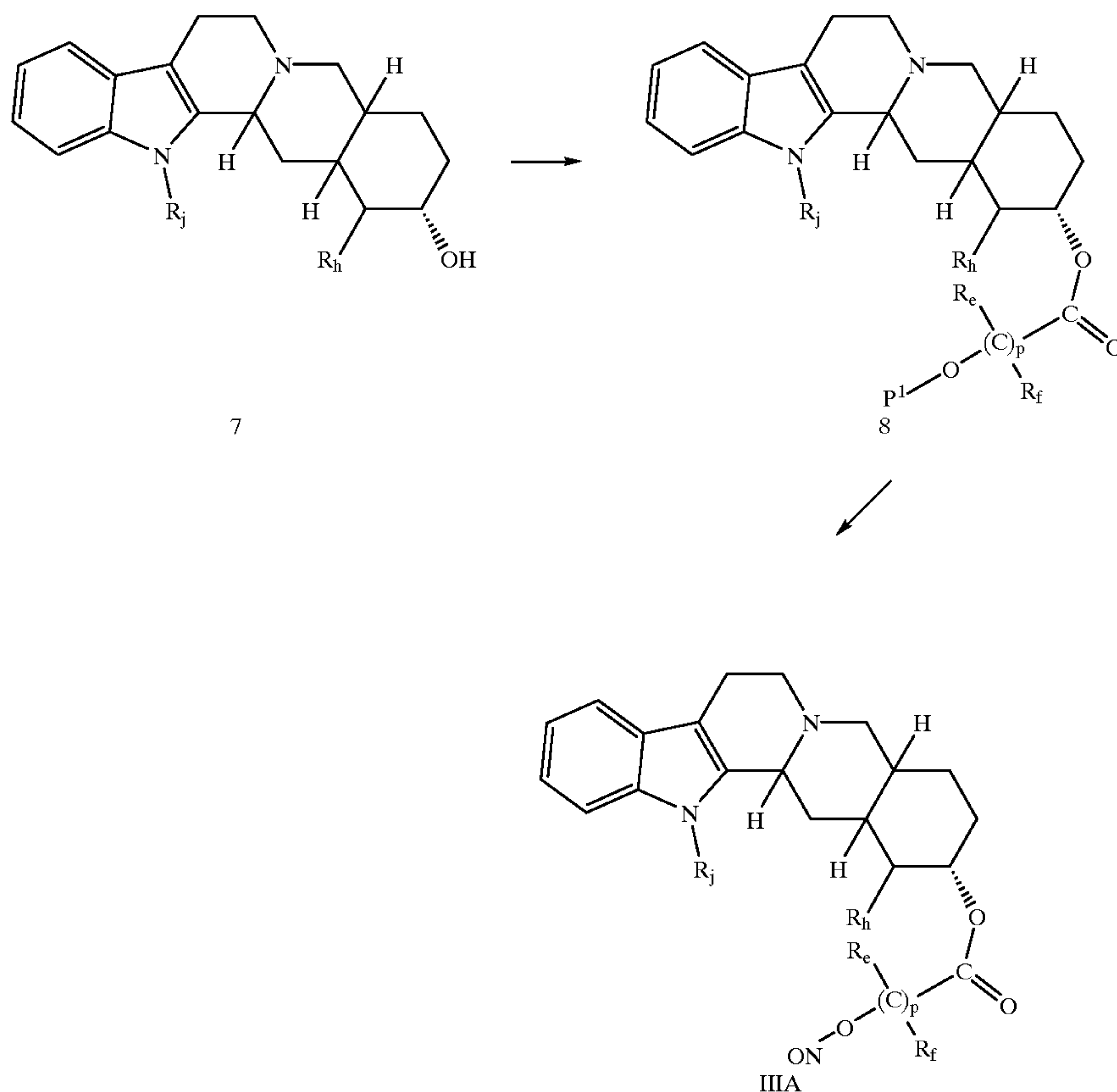
Scheme VII
