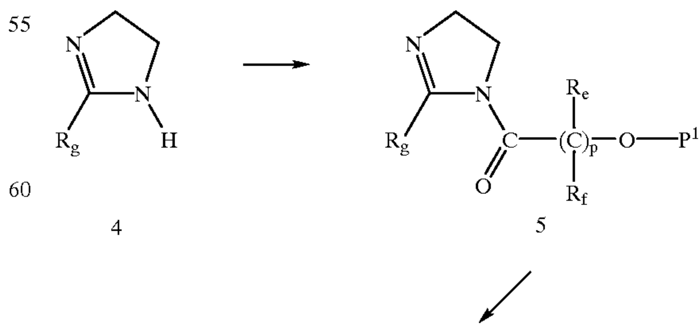
Scheme IV
