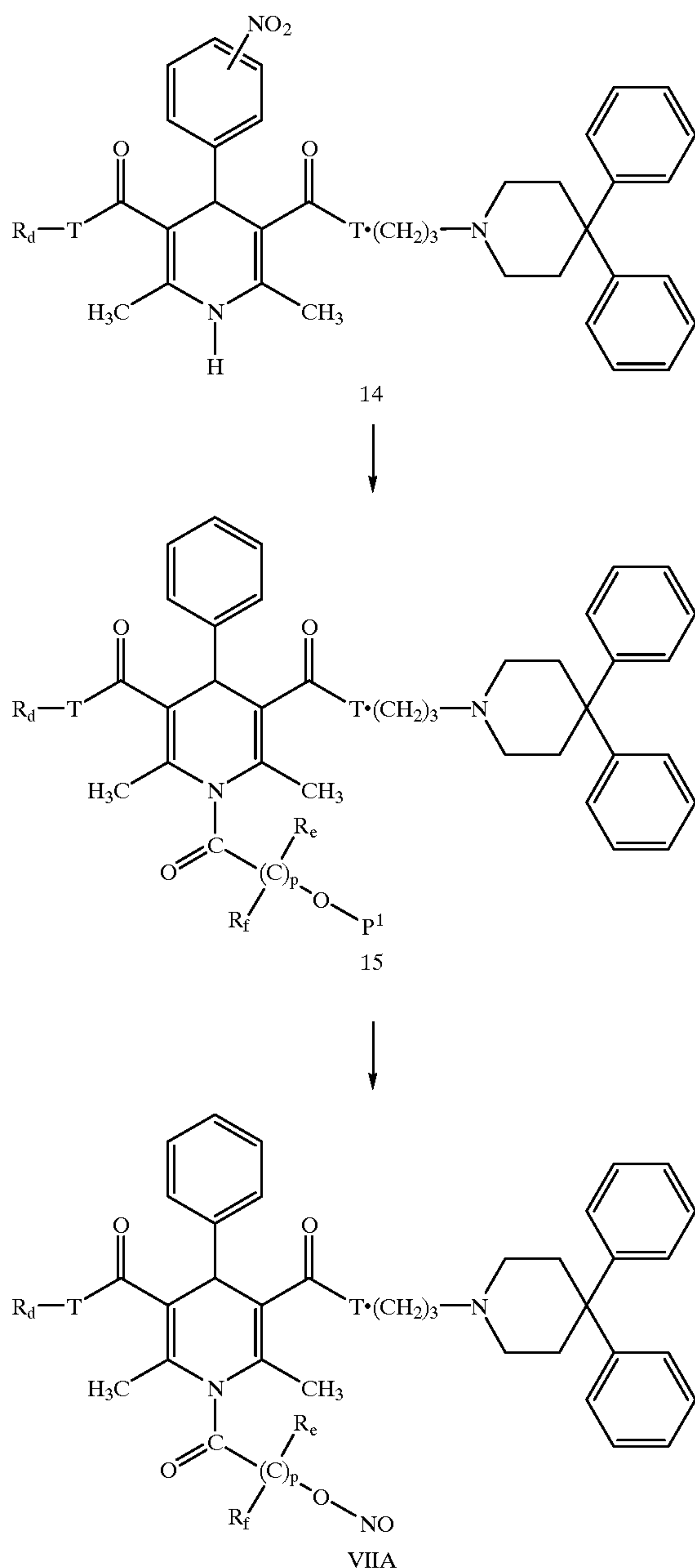
Scheme XVI
