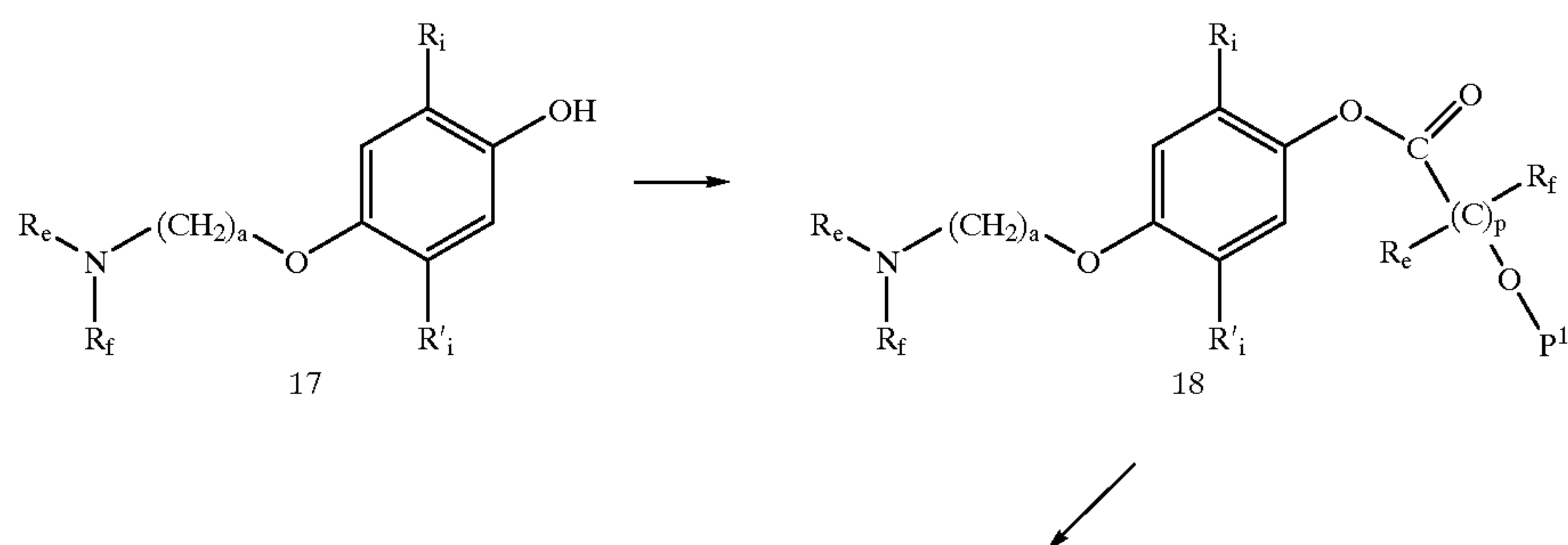
Scheme XIX
