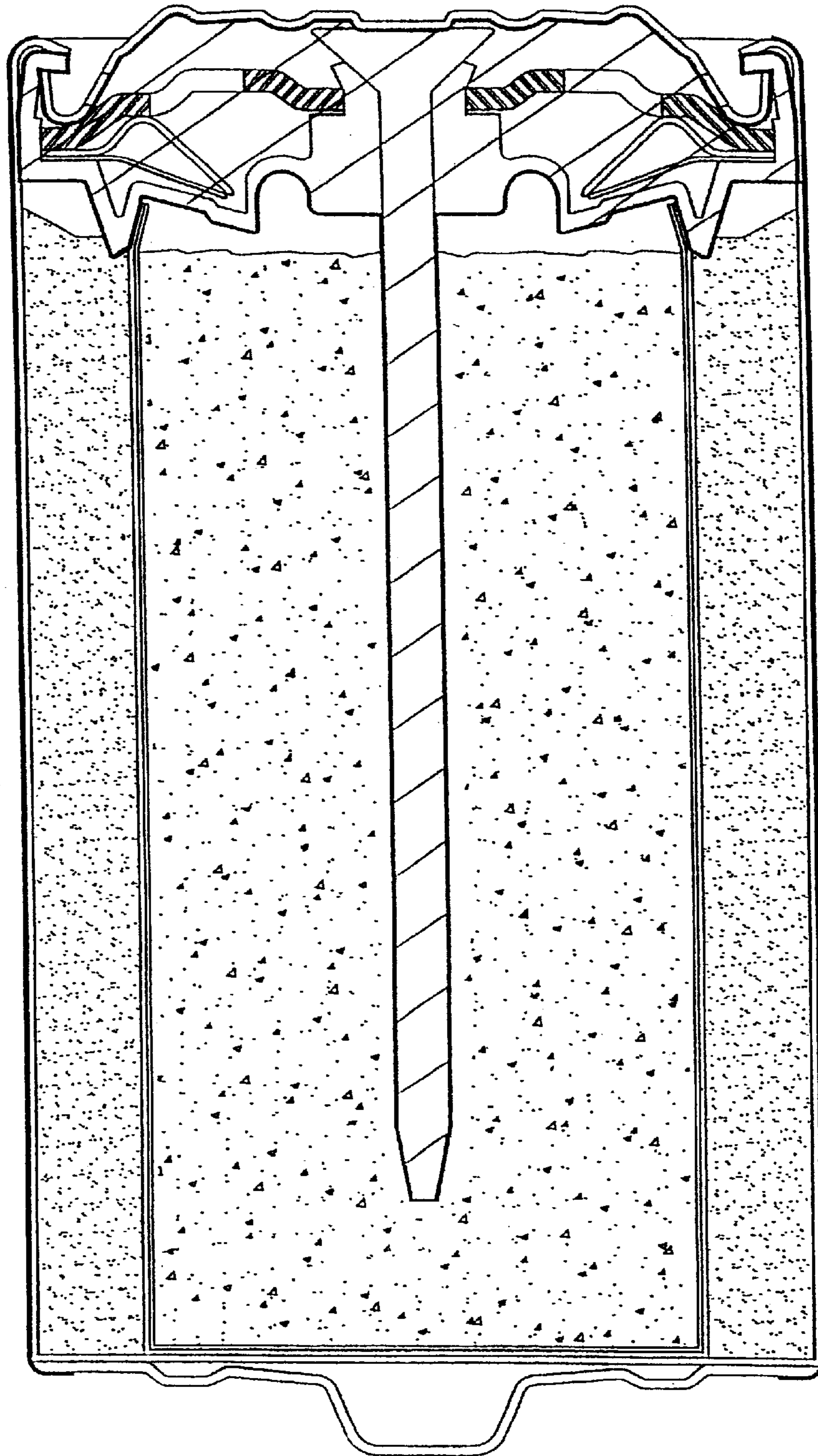
FIG. 3C PRIOR ART
