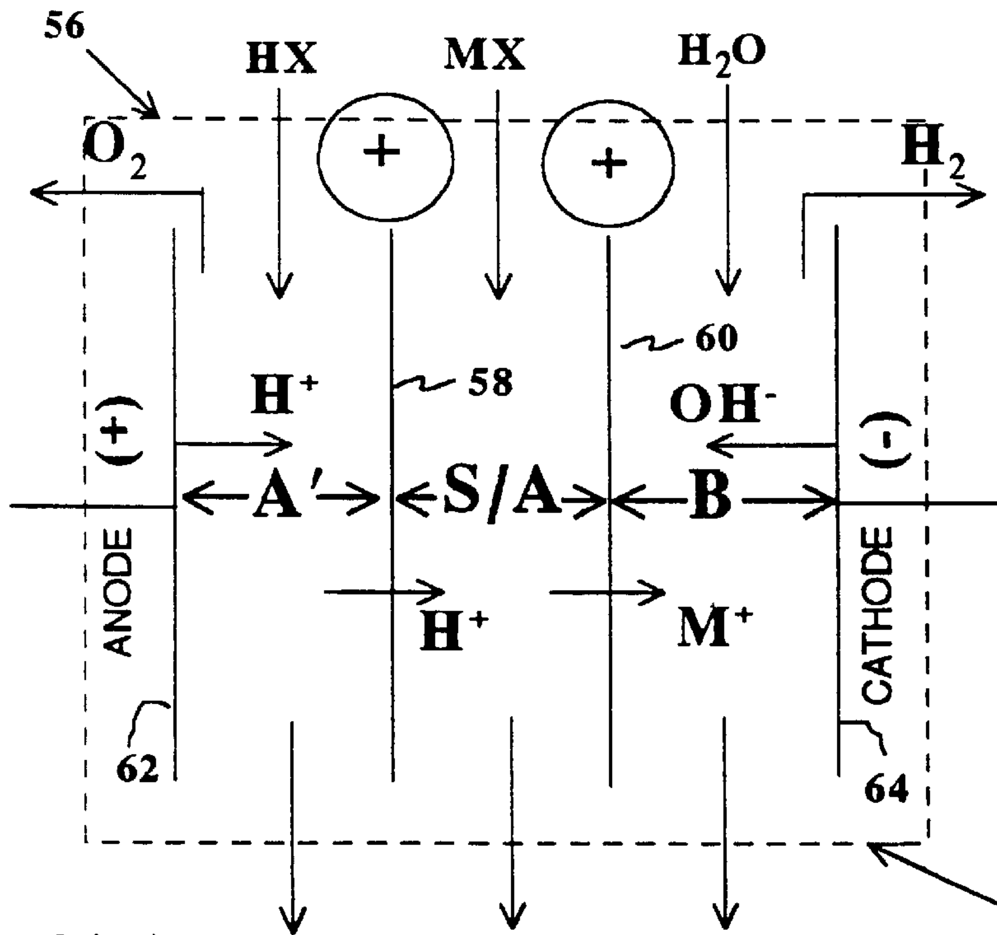
FIG. 2(a) HX HX+MX MOH UNIT CELL
