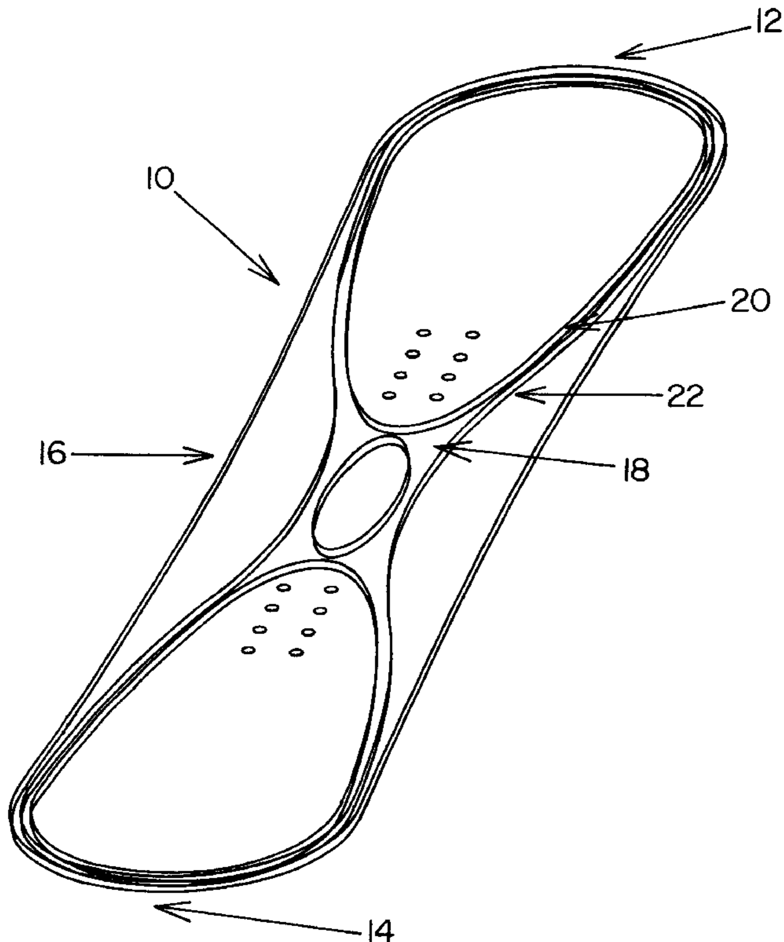
STRUCTURAL COMPONENTS MIRRORED ABOUT THE NEUTRAL AXIS OF THE SNOWBOARD.
