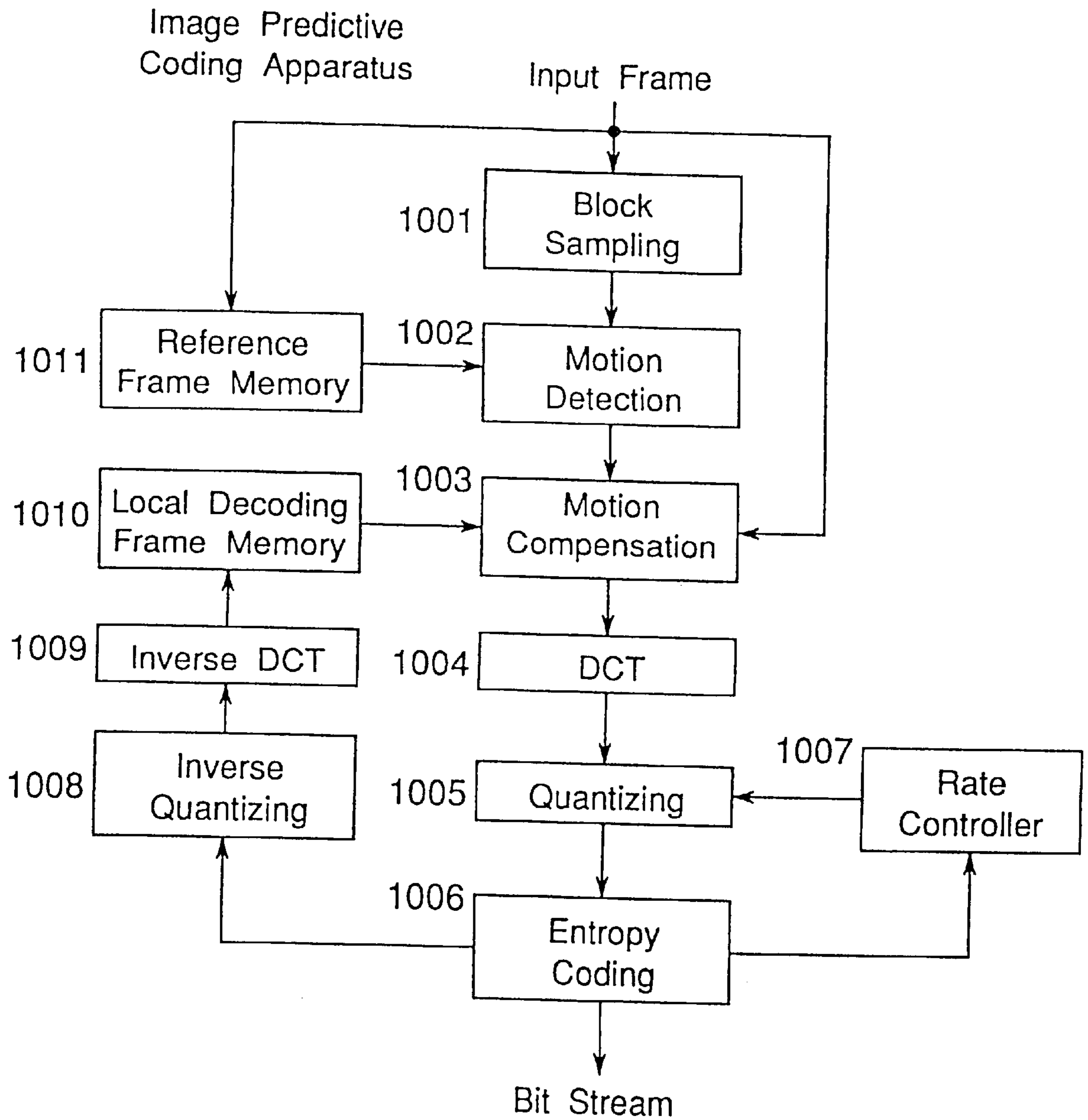
Fig.14 PRIOR ART
