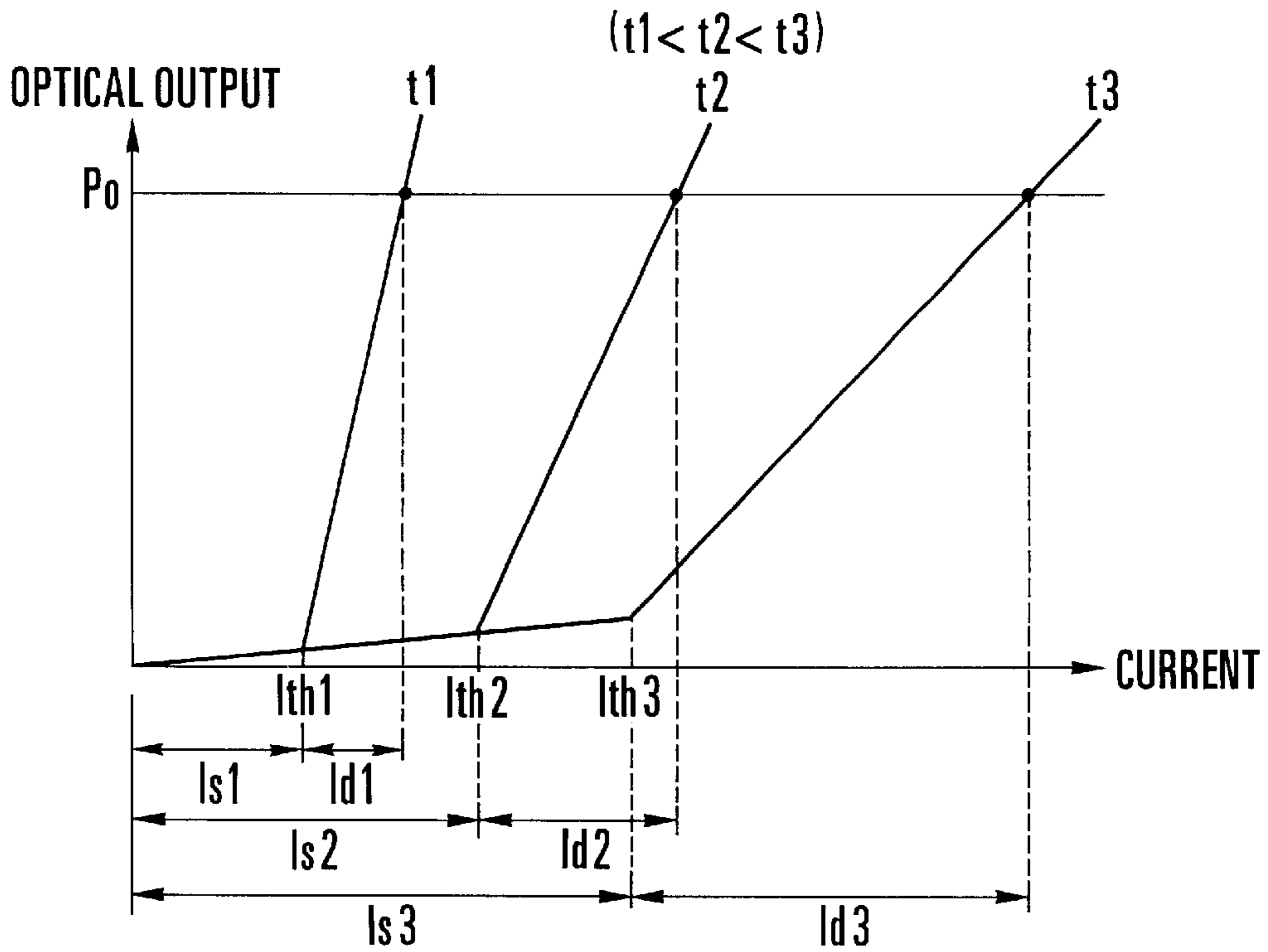
IDEAL DISTRIBUTION OF BIAS CURRENT AND DRIVING CURRENT
