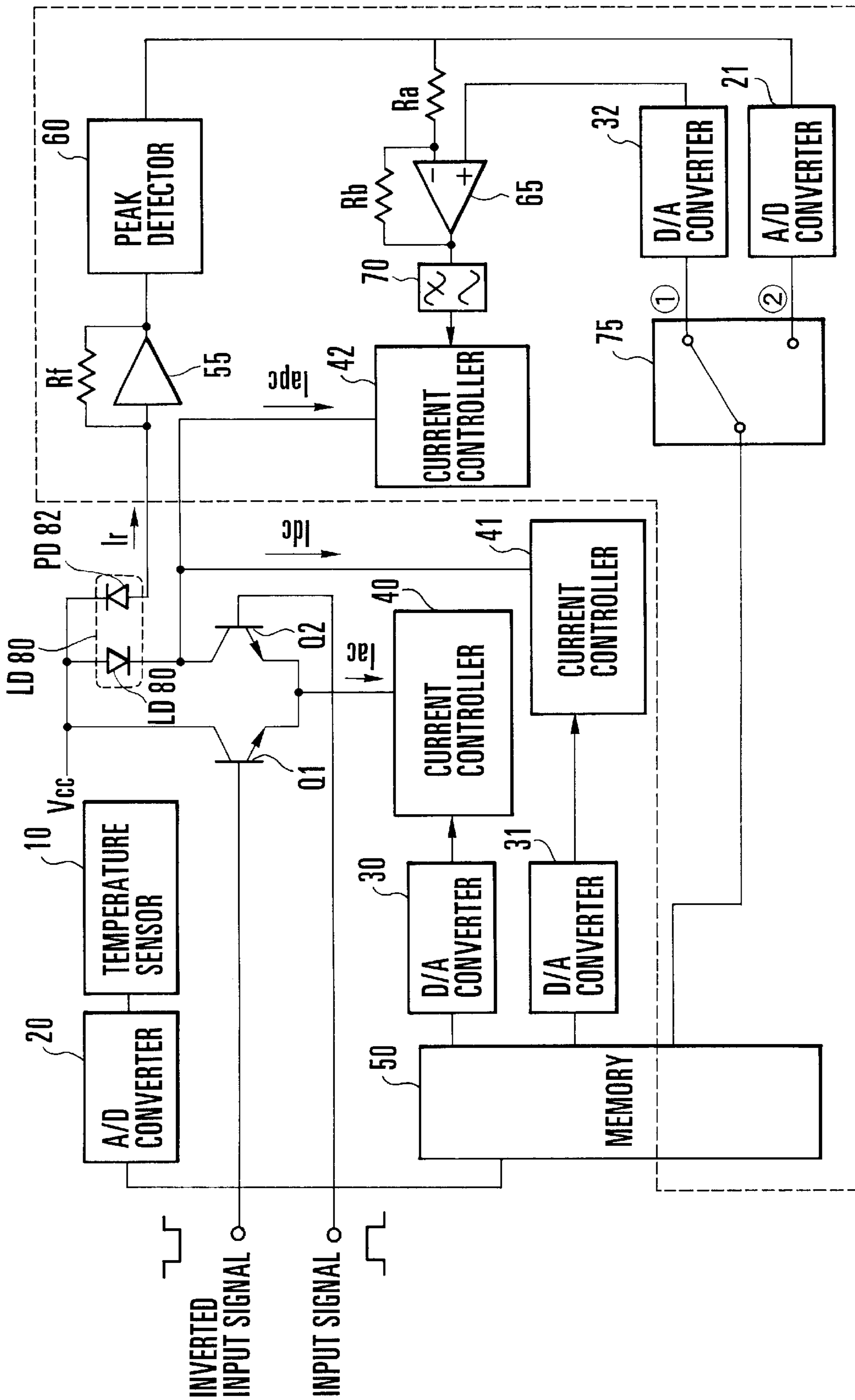
LASER DIODE TIME DETERIORATION COMPENSATION CIRCUIT 1
