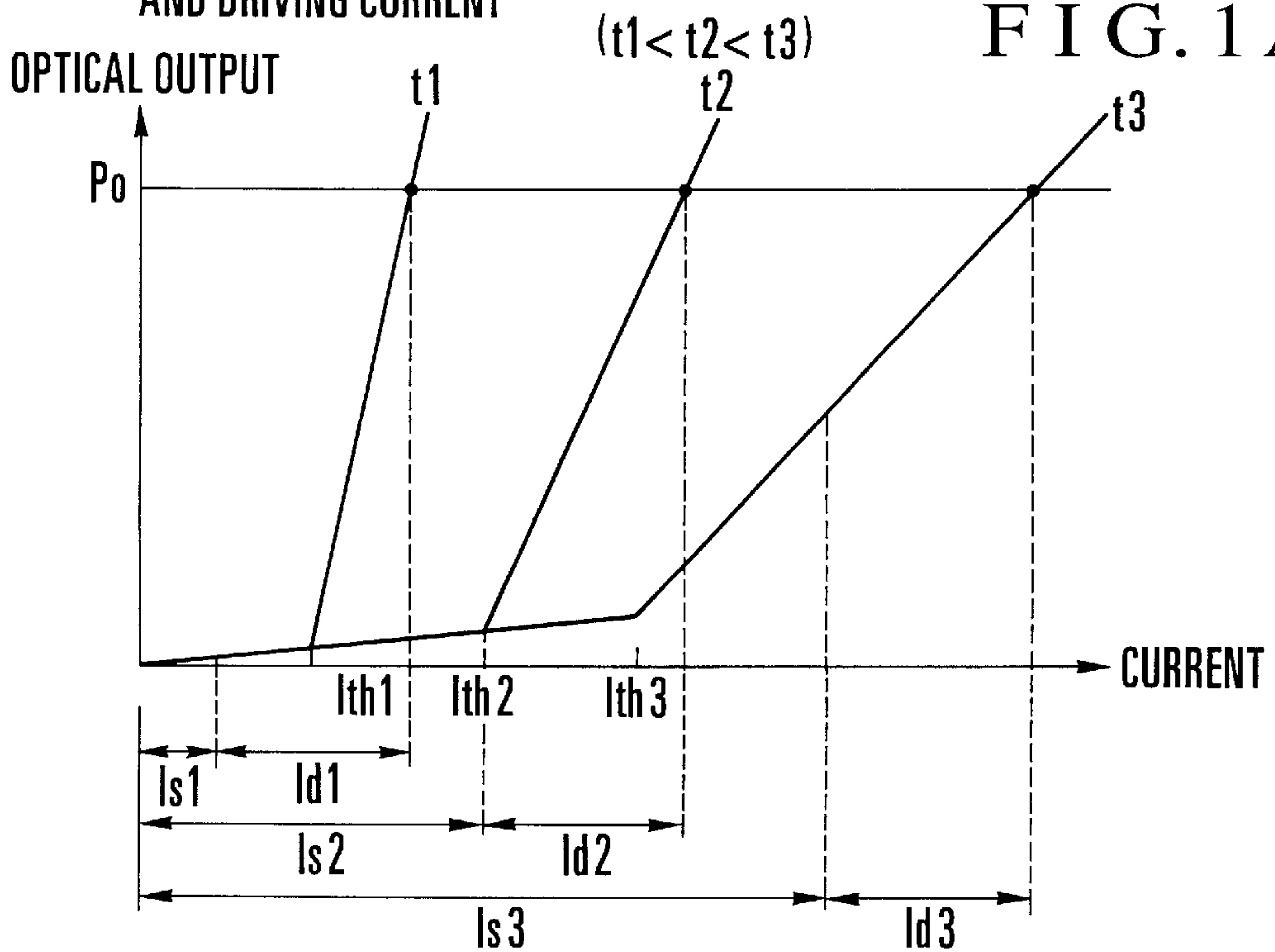
CURRENT DISTRIBUTION FOR CONSTANT DRIVING CURRENT ( l_{d1} < l_{d2} < l_{d3} )
